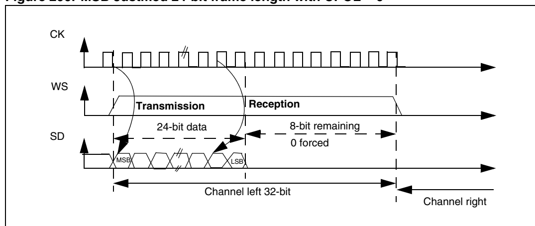
Figure 296. MSB Justified 24-bit frame length with CPOL = 0
