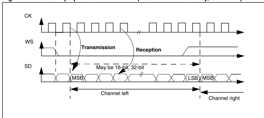
Figure 289. I 2 S Philips protocol waveforms (16/32-bit full accuracy, CPOL = 0)
