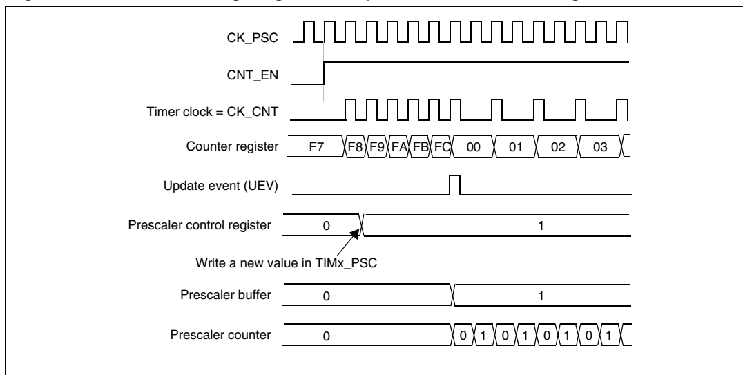
Figure 120. Counter timing diagram with prescaler division change from 1 to 2
