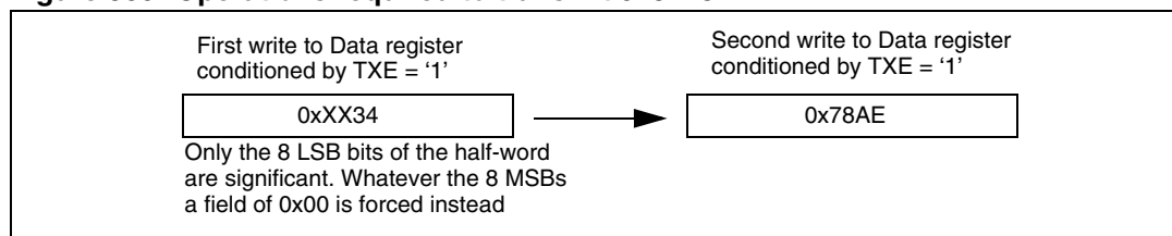
Figure 300. Operations required to transmit 0x3478AE
