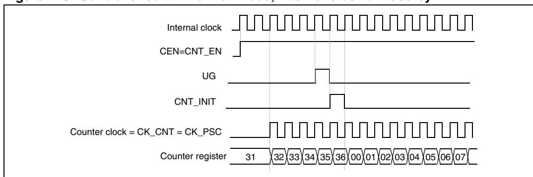
Figure 175. Control circuit in normal mode, internal clock divided by 1
