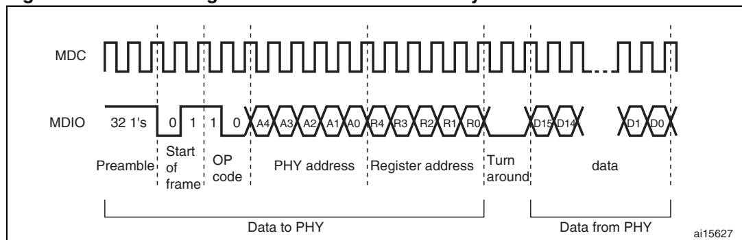
Figure 324. MDIO timing and frame structure - Read cycle
