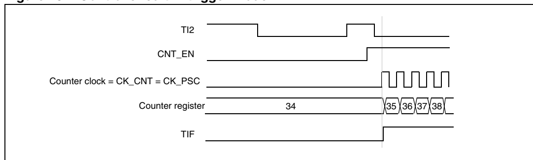
Figure 157. Control circuit in trigger mode
