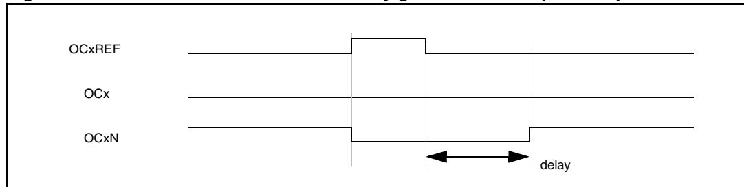
Figure 107. Dead-time waveforms with delay greater than the positive pulse.
