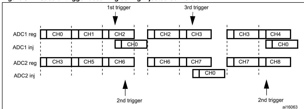
Figure 52. Case of trigger occurring during injected conversion
