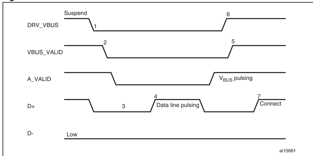
Figure 377. A-device SRP
