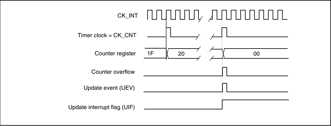
Figure 195. Counter timing diagram, update event when ARPE = 0 (TIMx_ARR not preloaded)
