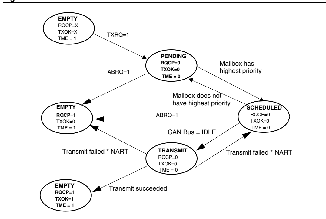
Figure 229. Transmit mailbox states
