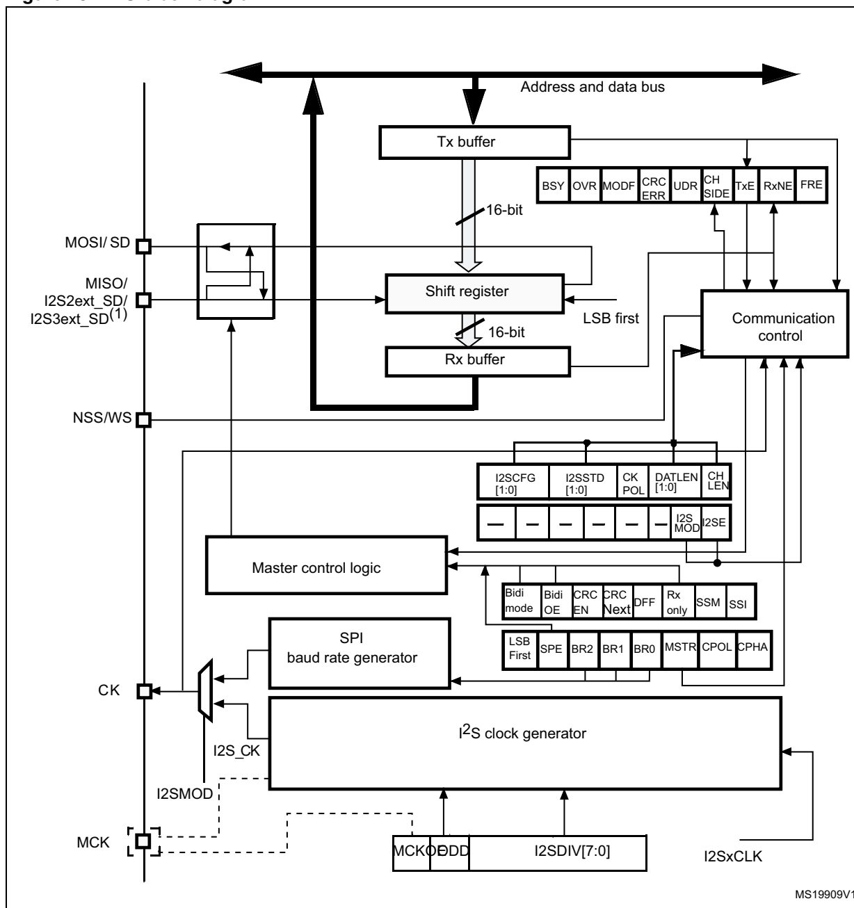
Figure 287. I 2 S block diagram
