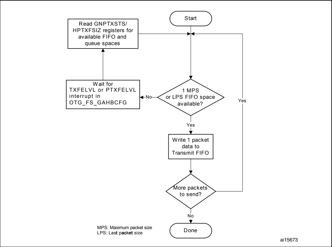
Figure 385. Transmit FIFO write task
