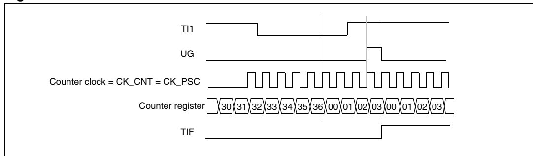
Figure 155. Control circuit in reset mode
