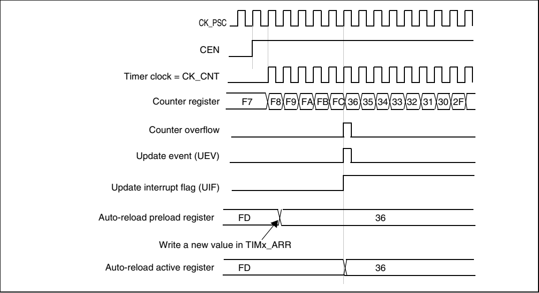
Figure 90. Counter timing diagram, Update event with ARPE=1 (counter overflow)
