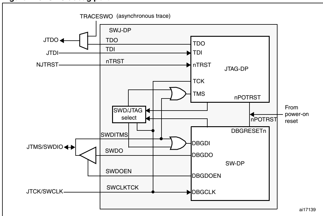
Figure 426. SWJ debug port
