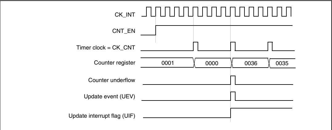
Figure 130. Counter timing diagram, internal clock divided by 4
