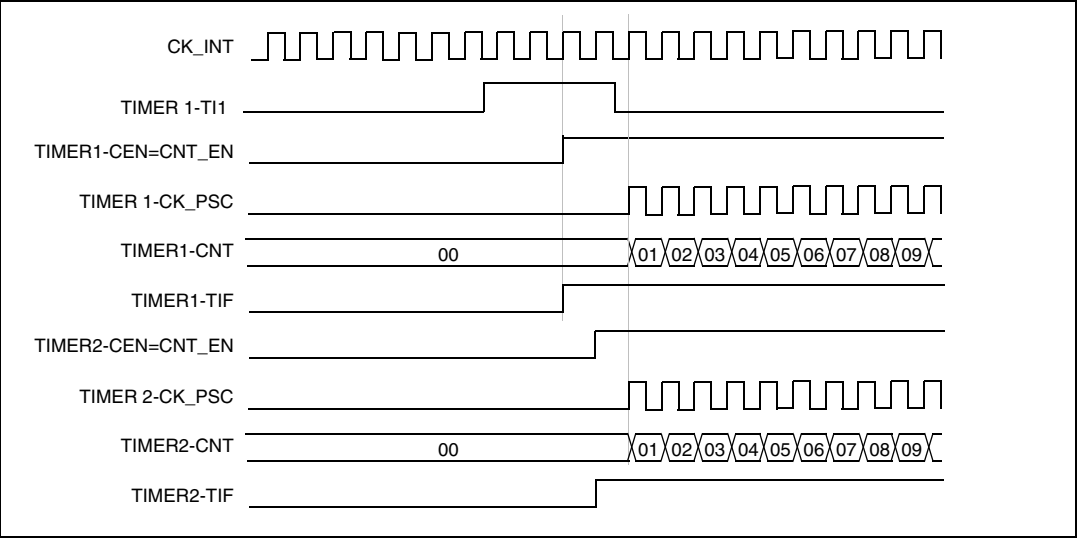
Figure 164. Triggering timer 1 and 2 with timer 1 TI1 input
