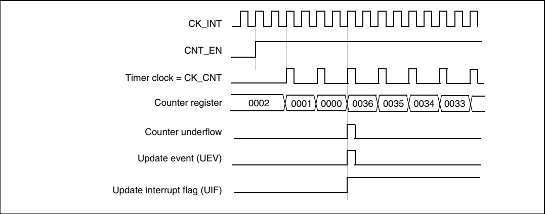
Figure 129. Counter timing diagram, internal clock divided by 2
