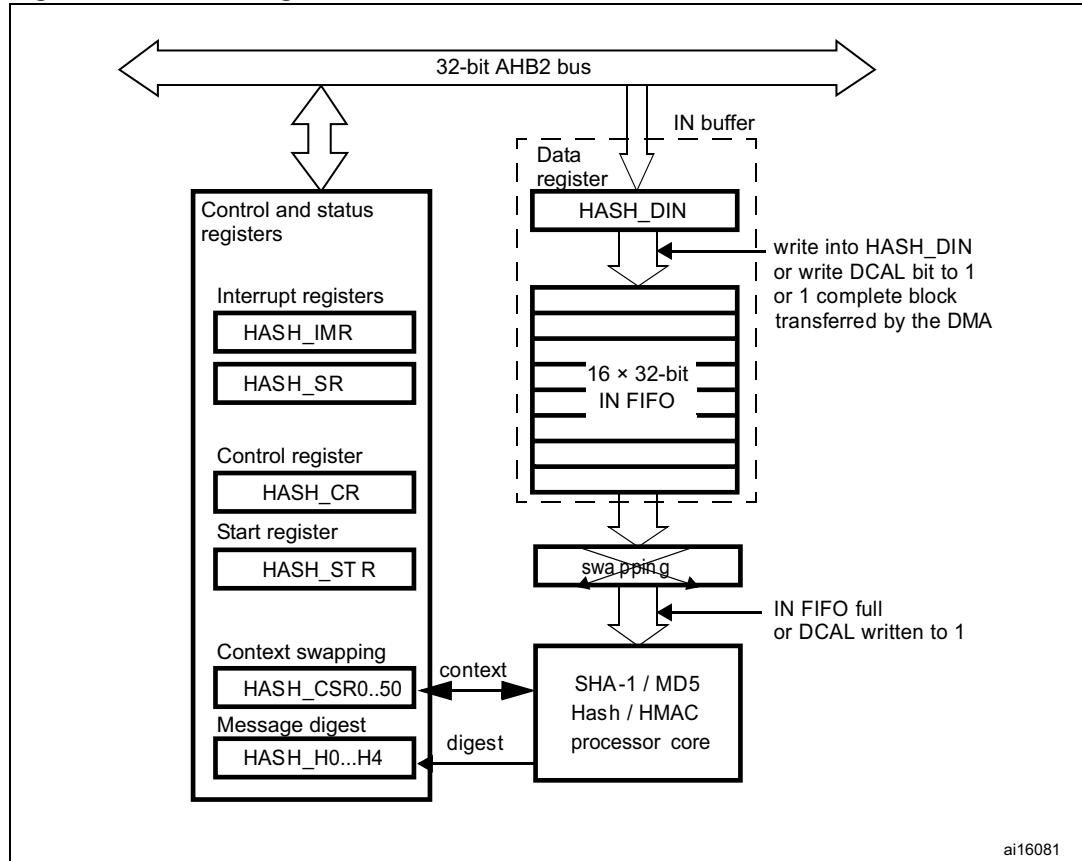
Figure 218. Block diagram for STM32F405xx/07xx and STM32F415xx/17xx
