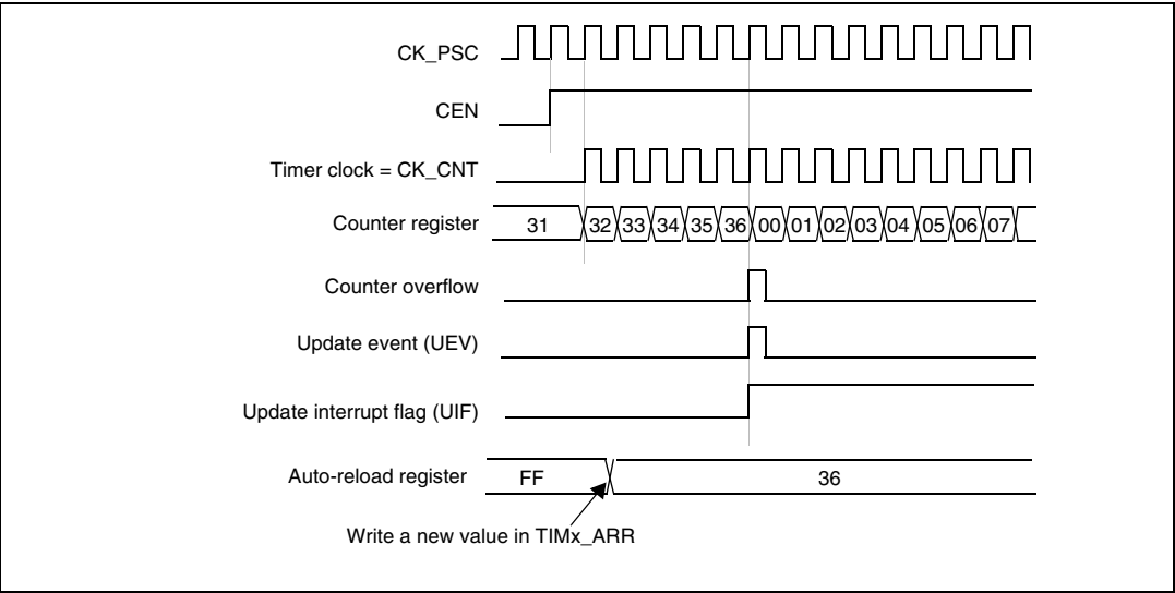
Figure 78. Counter timing diagram, update event when ARPE=0 (TIMx_ARR not preloaded)
