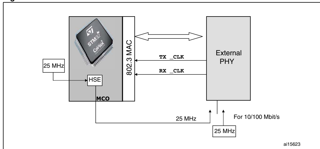
Figure 326. MII clock sources
