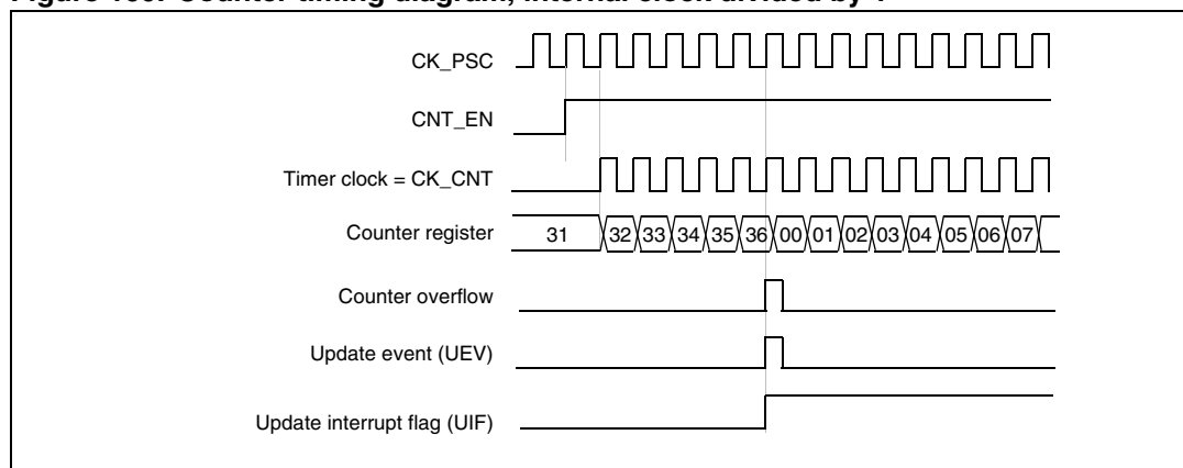
Figure 169. Counter timing diagram, internal clock divided by 1
