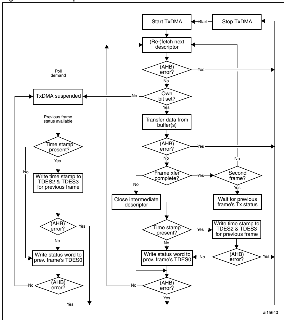
Figure 349. TxDMA operation in OSF mode
