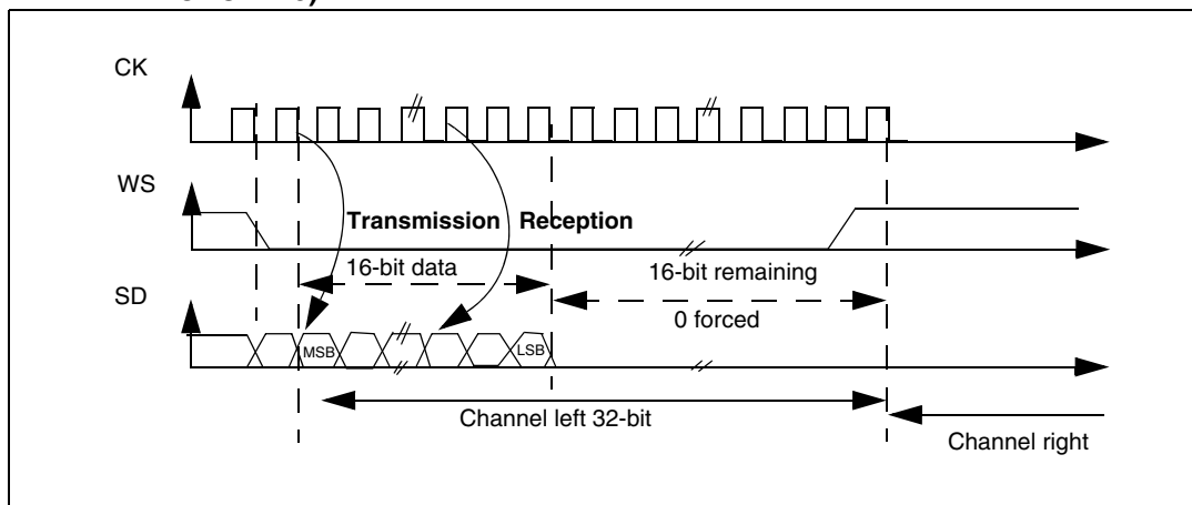
Figure 293. I 2 S Philips standard (16-bit extended to 32-bit packet frame with CPOL = 0)
