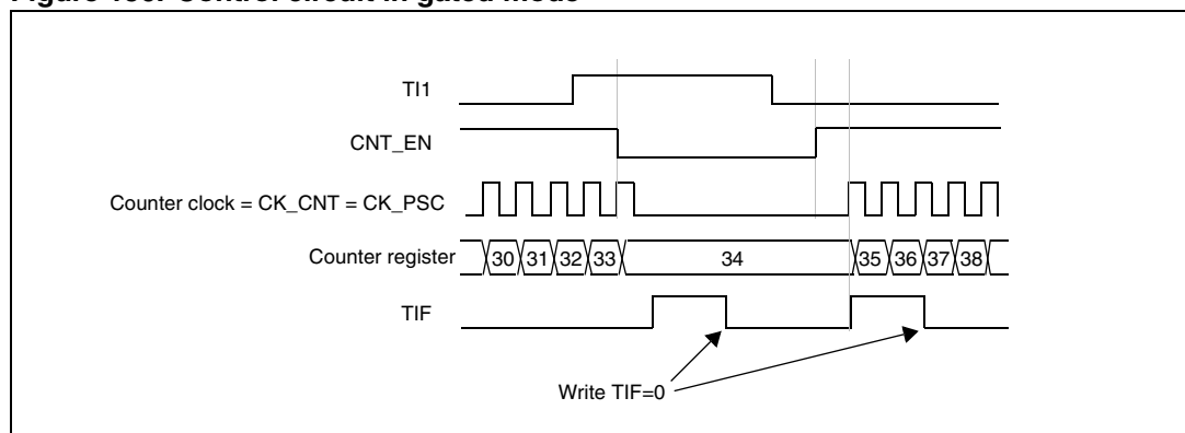
Figure 156. Control circuit in gated mode
