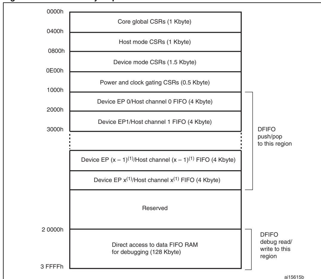
Figure 384. CSR memory map
