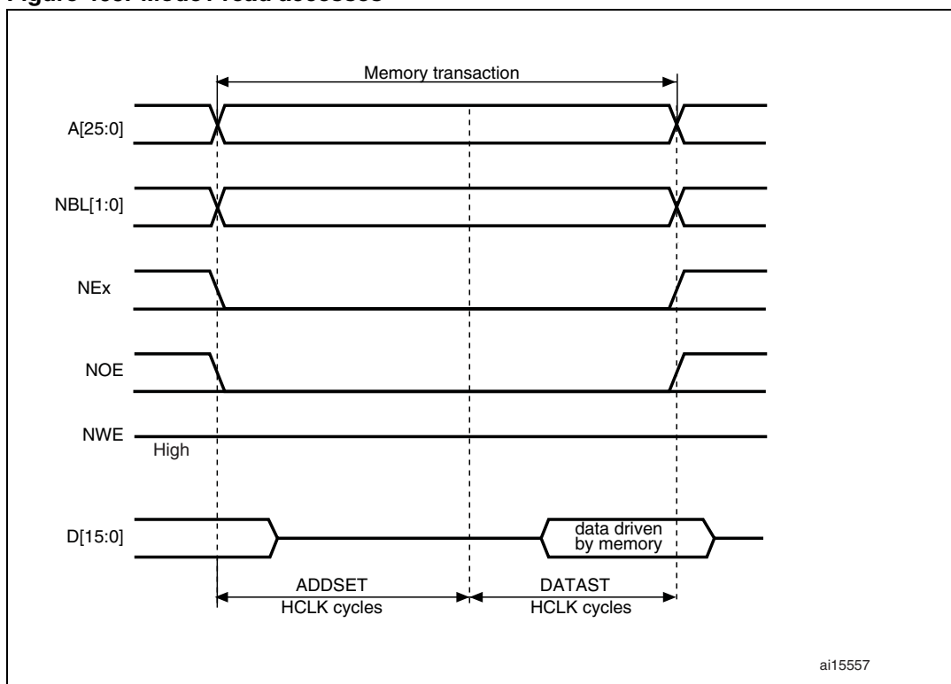
Figure 405. Mode1 read accesses
