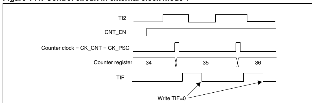
Figure 141. Control circuit in external clock mode 1
