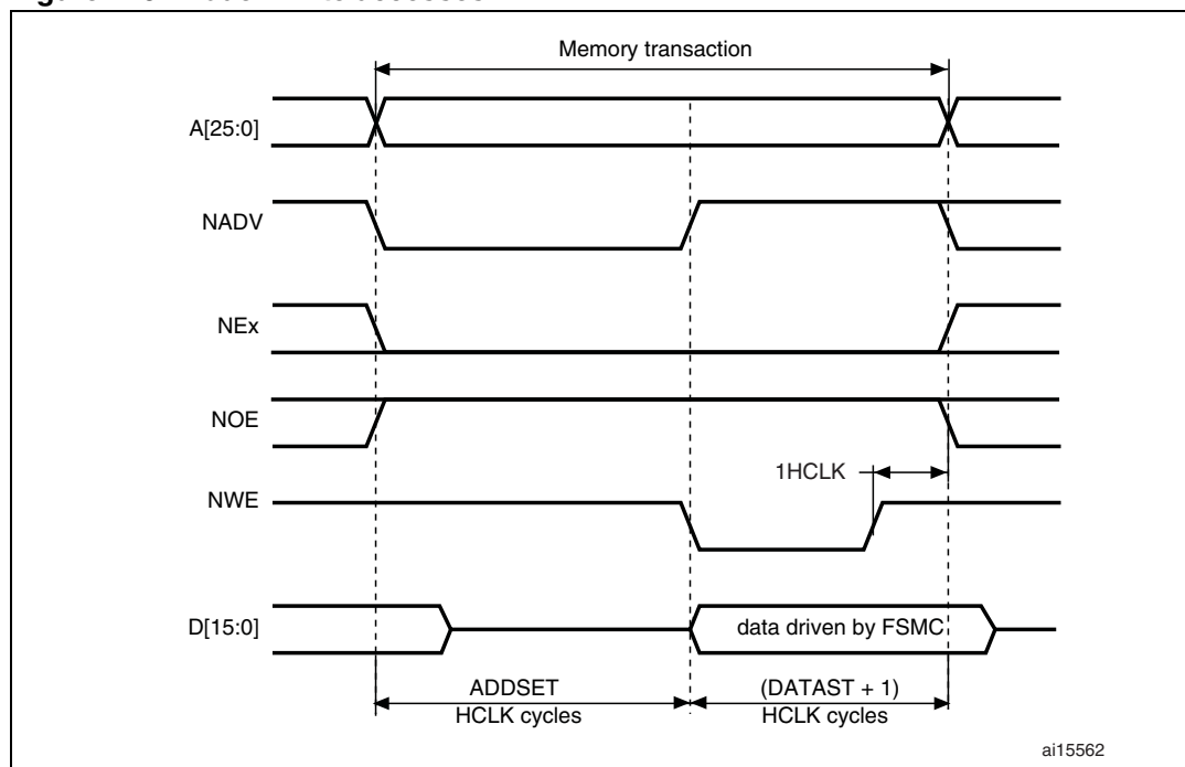
Figure 411. ModeB write accesses
