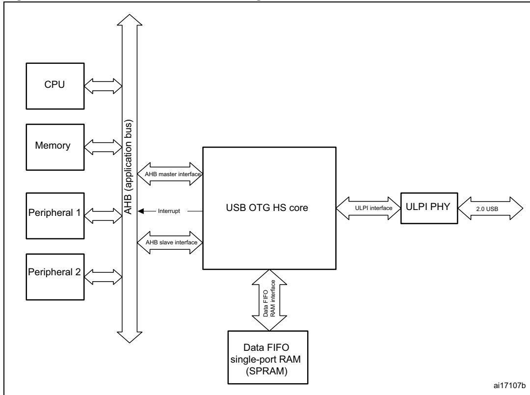
Figure 381. USB OTG interface block diagram
