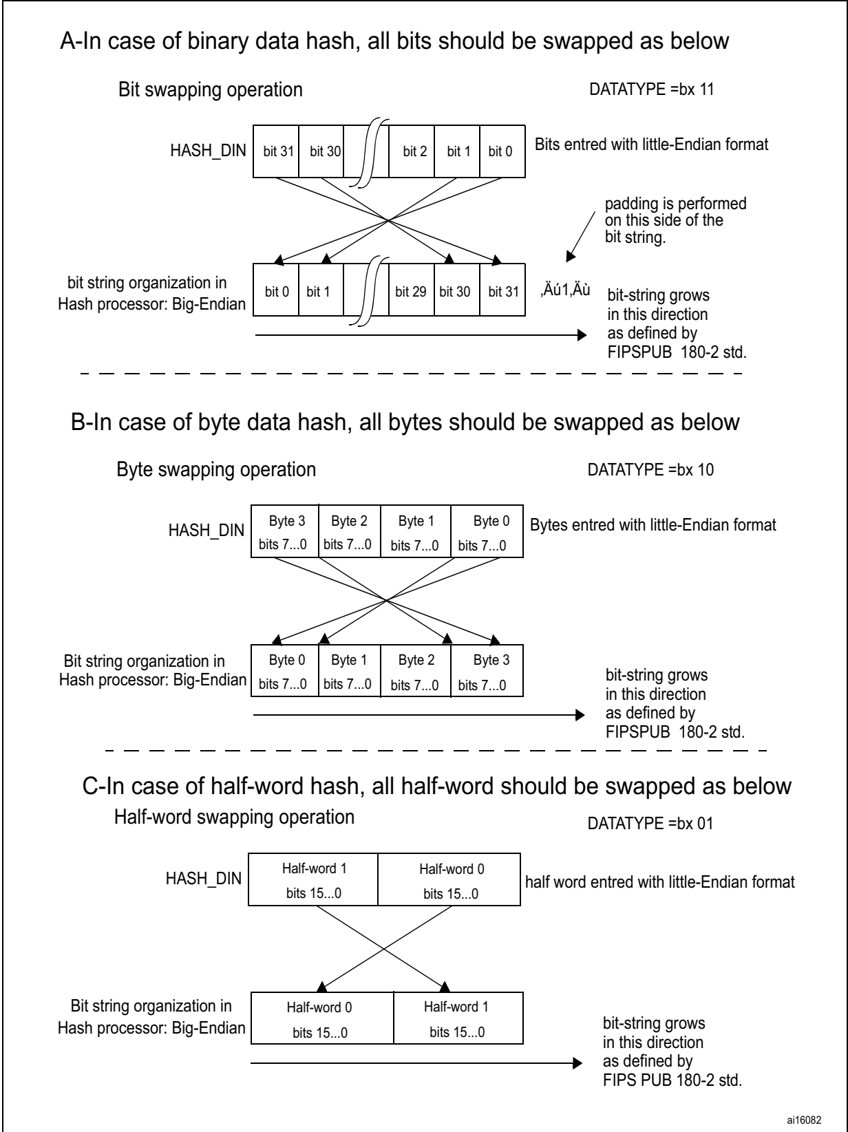
Figure 220. Bit, byte and half-word swapping
