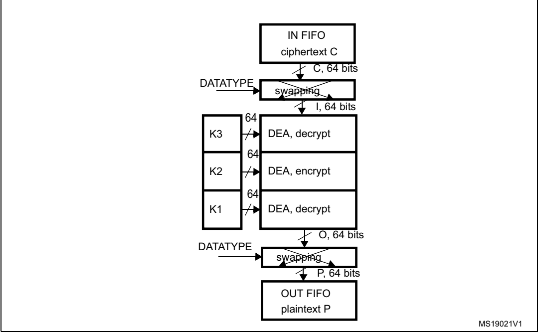
Figure 204. DES/TDES-ECB mode decryption
