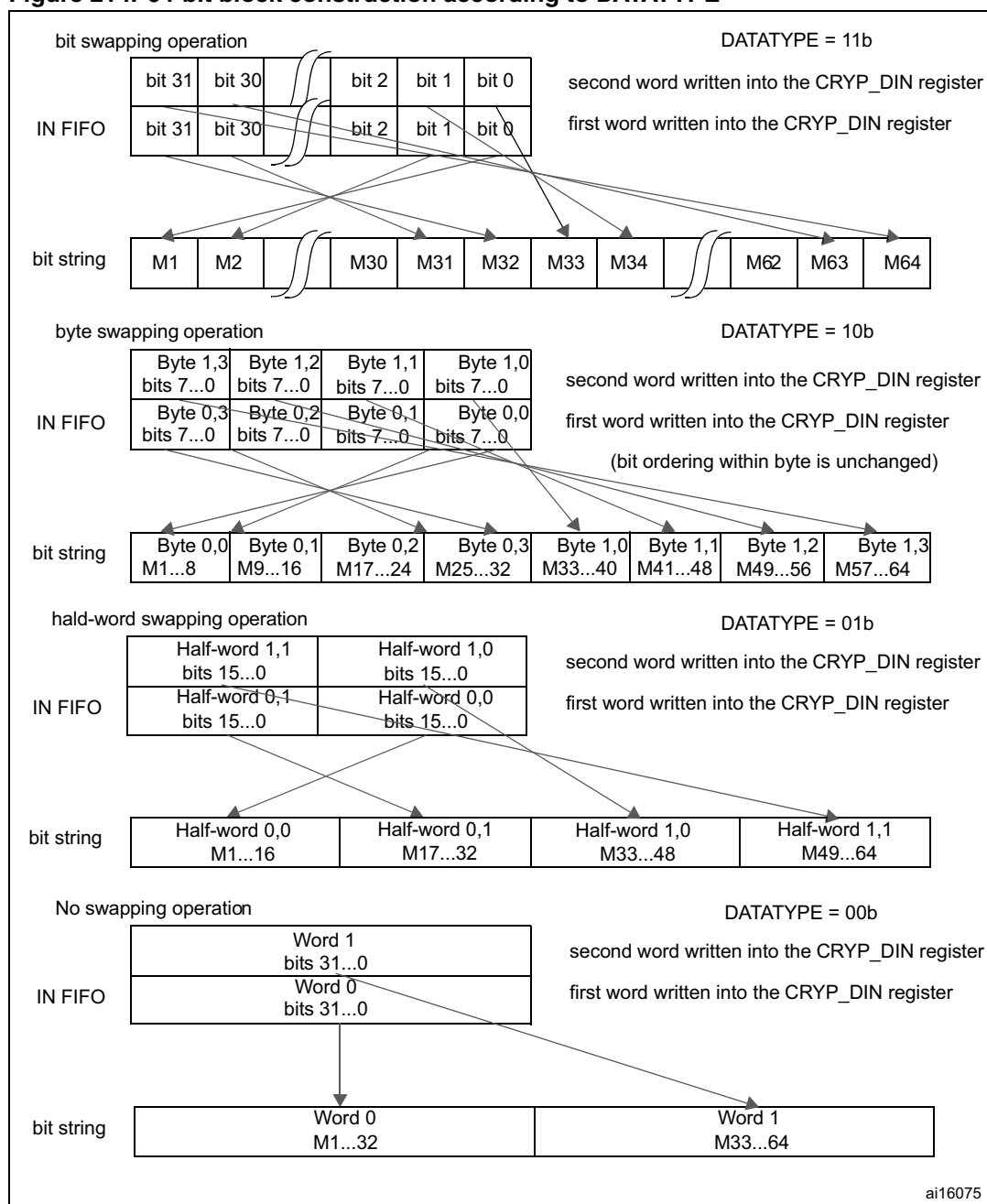
Figure 214. 64-bit block construction according to DATATYPE
