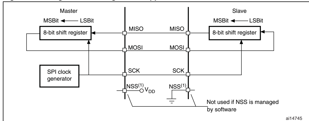
Figure 272. Single master/ single slave application
