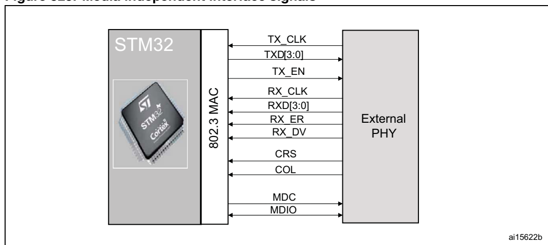
Figure 325. Media independent interface signals
