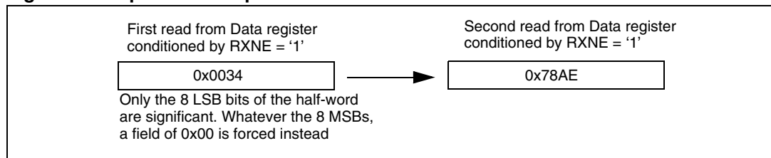
Figure 301. Operations required to receive 0x3478AE
