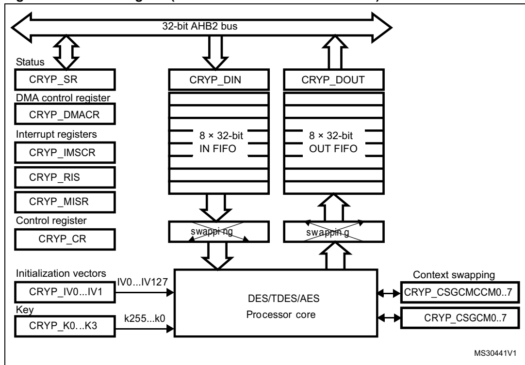
Figure 202. Block diagram (STM32F42xxx and STM32F43xxx)
