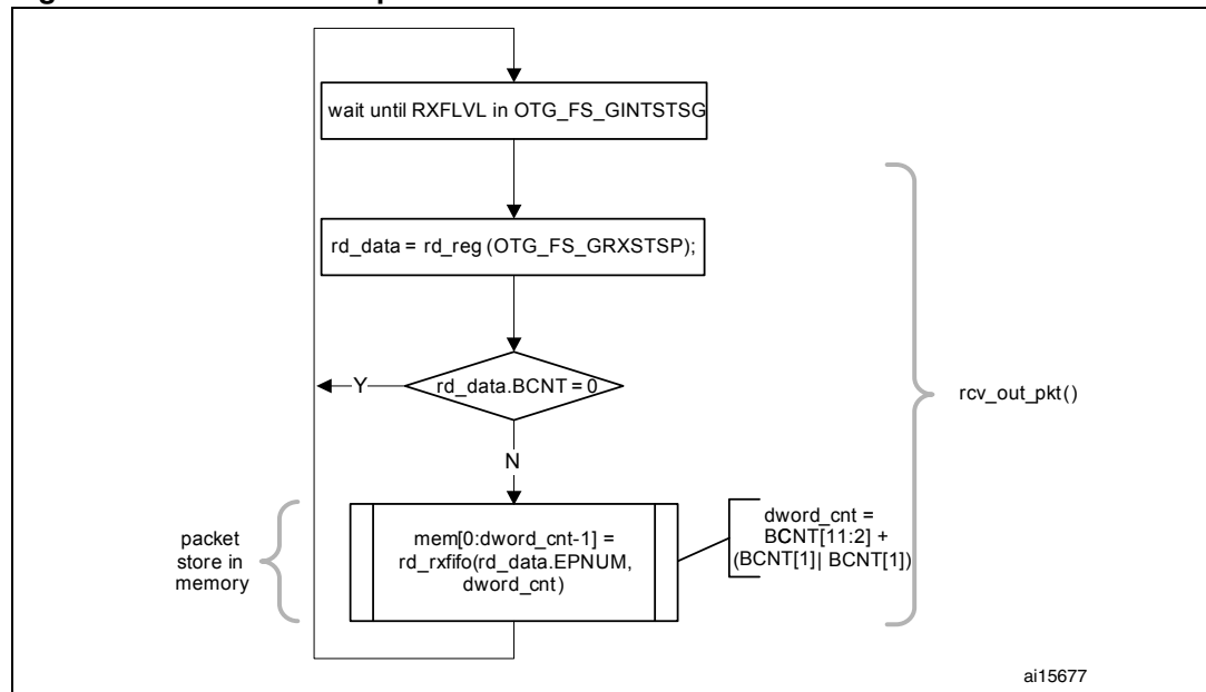
Figure 395. Receive FIFO packet read in slave mode
