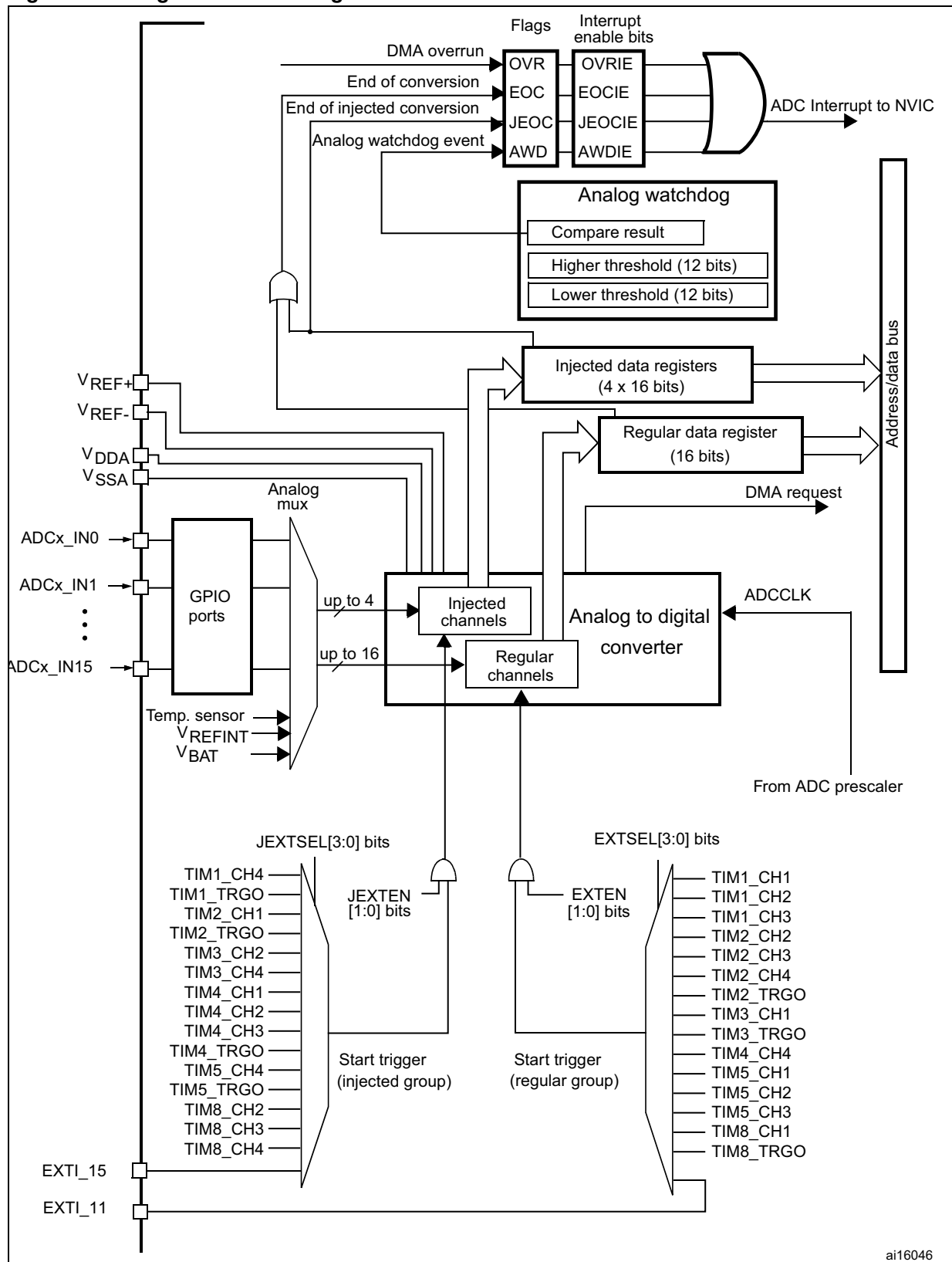
Figure 34. Single ADC block diagram
