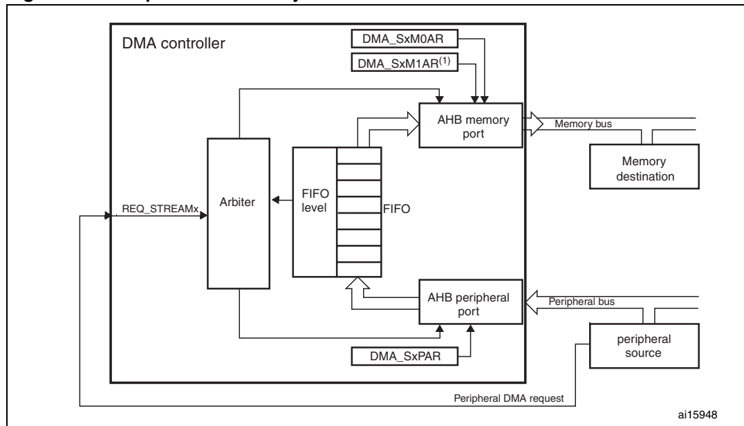
Figure 28. Peripheral-to-memory mode
