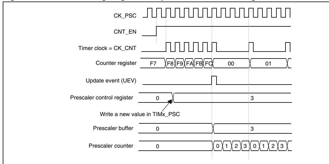
Figure 121. Counter timing diagram with prescaler division change from 1 to 4
