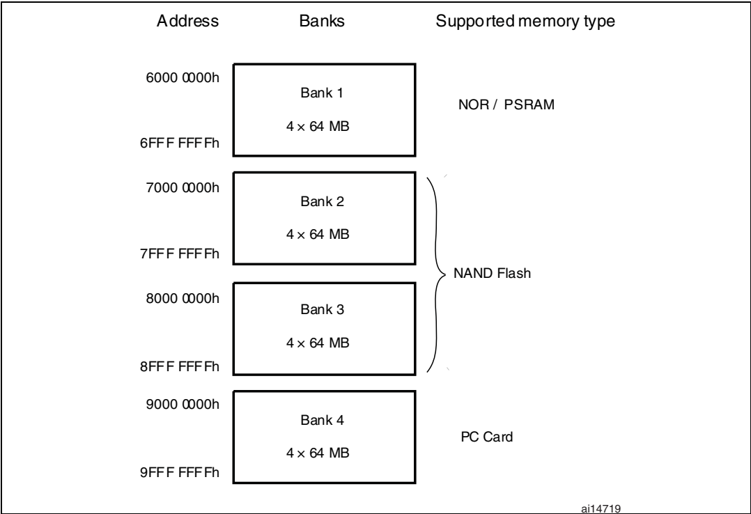
Figure 404. FSMC memory banks
