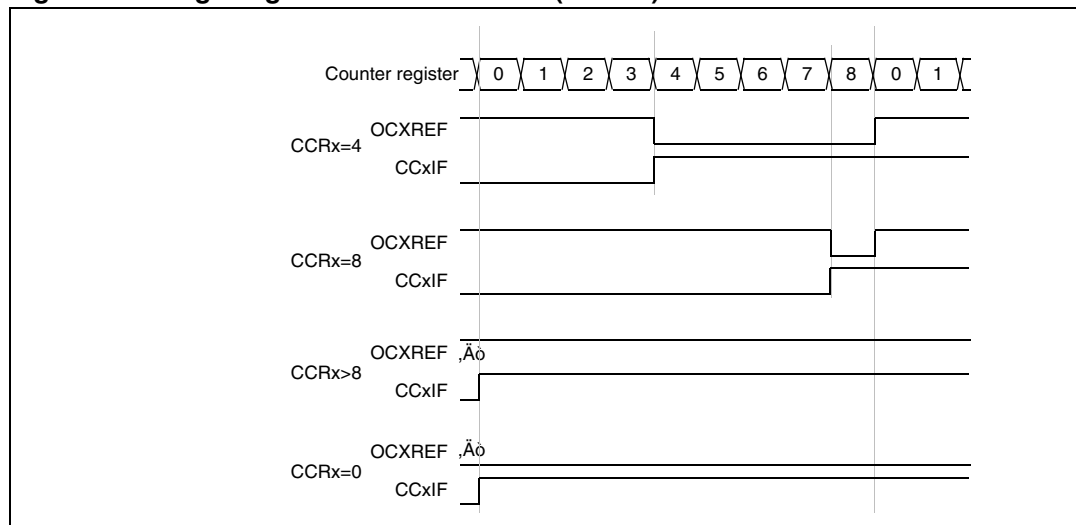
Figure 183. Edge-aligned PWM waveforms (ARR=8)
