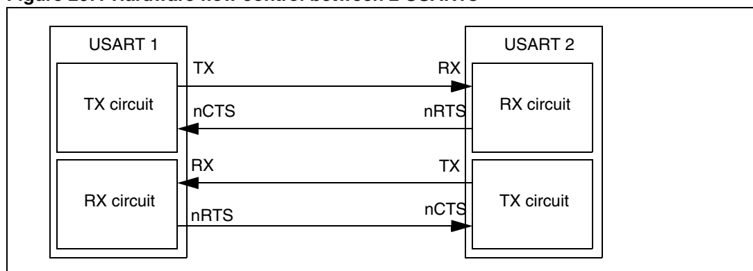
Figure 267. Hardware flow control between 2 USARTs
