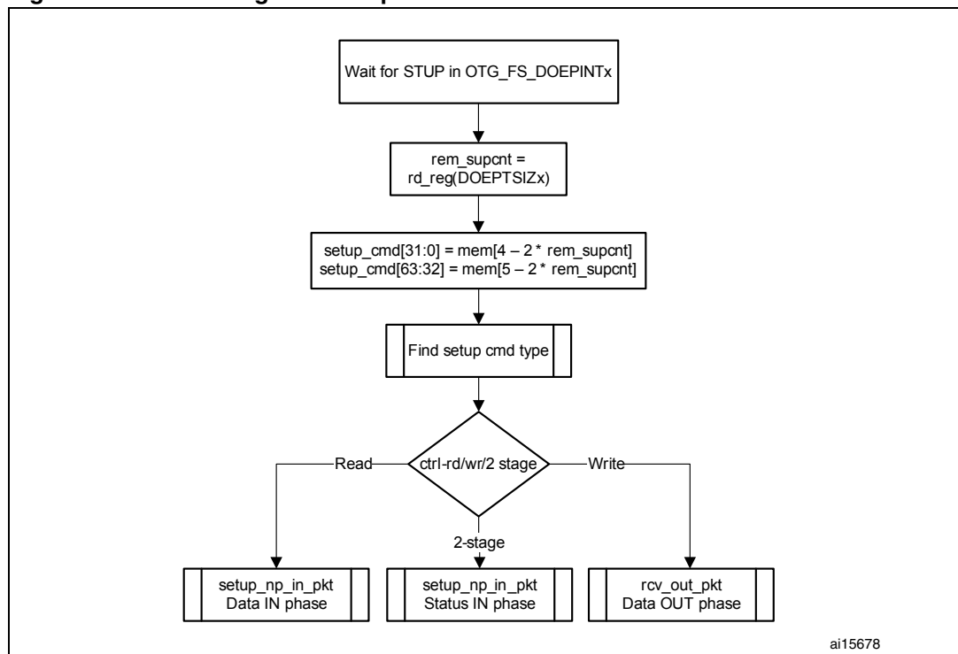
Figure 396. Processing a SETUP packet
