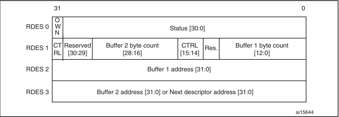
Figure 353. Normal Rx DMA descriptor structure
