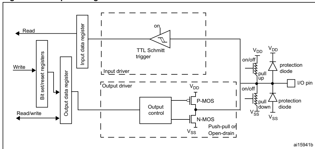
Figure 21. Output configuration
