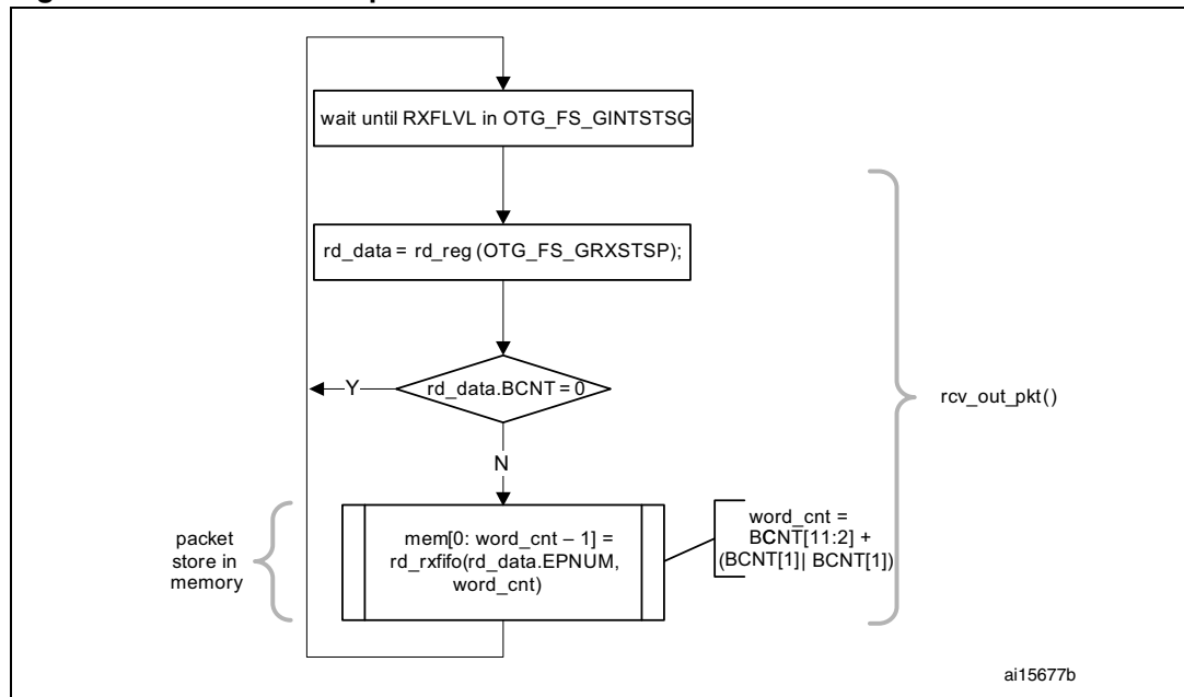
Figure 373. Receive FIFO packet read
