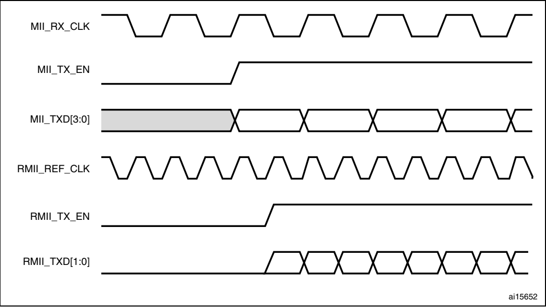
Figure 336. Frame transmission in MMI and RMII modes
