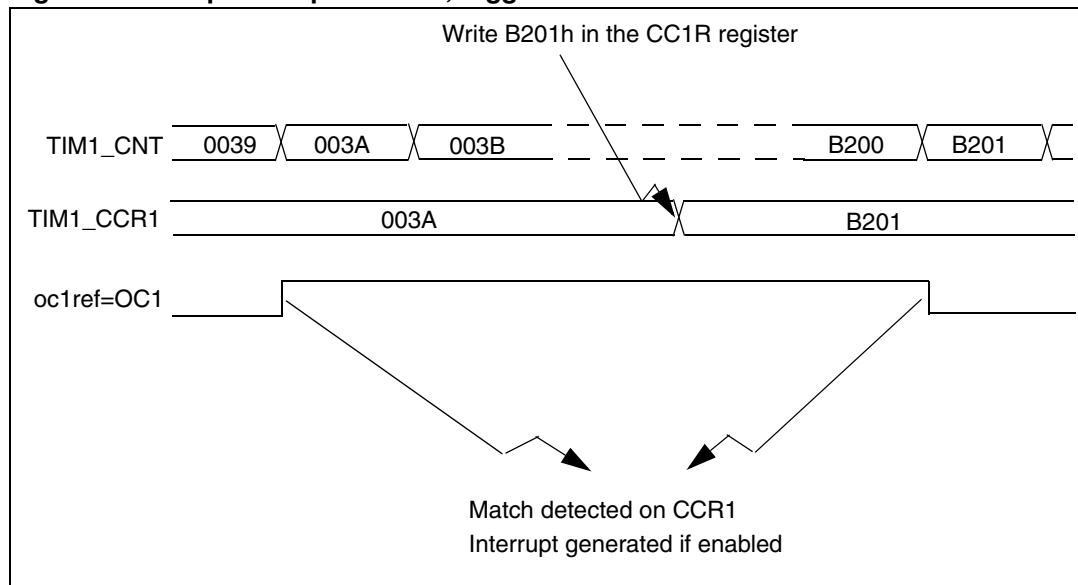
Figure 102. Output compare mode, toggle on OC1.
