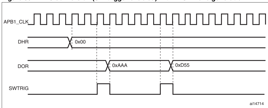
Figure 59. DAC conversion (SW trigger enabled) with LFSR wave generation
