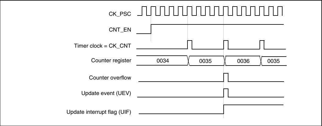
Figure 87. Counter timing diagram, internal clock divided by 4, TIMx_ARR=0x36
