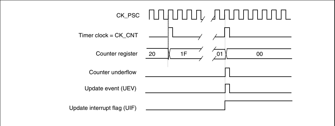
Figure 88. Counter timing diagram, internal clock divided by N
