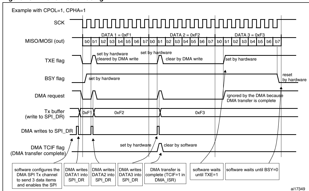
Figure 284. Transmission using DMA
