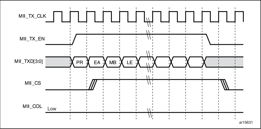
Figure 334. Transmission with no collision
