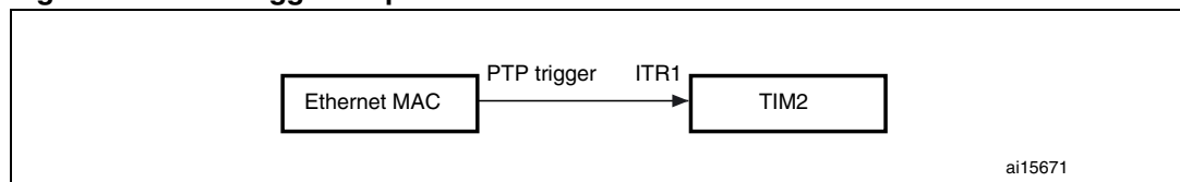
Figure 345. PTP trigger output to TIM2 ITR1 connection
