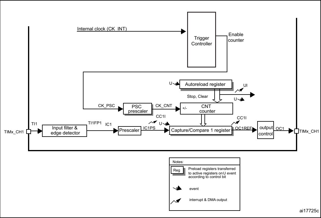
Figure 166. General-purpose timer block diagram (TIM10/11/13/14)
