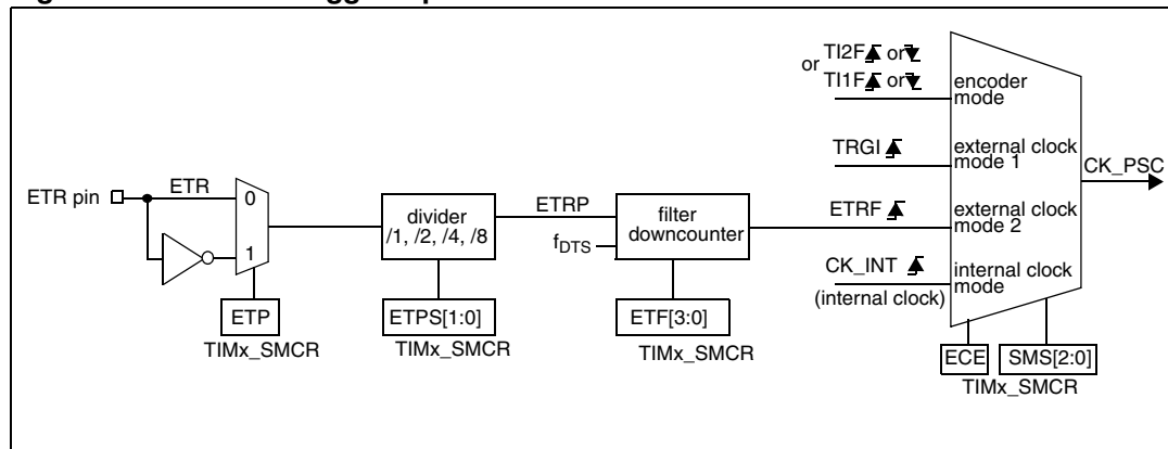
Figure 95. External trigger input block
