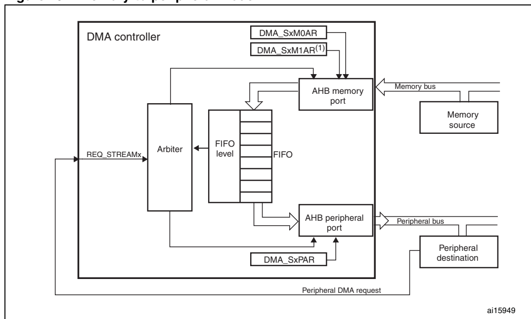
Figure 29. Memory-to-peripheral mode
