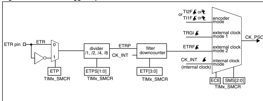
Figure 142. External trigger input block
