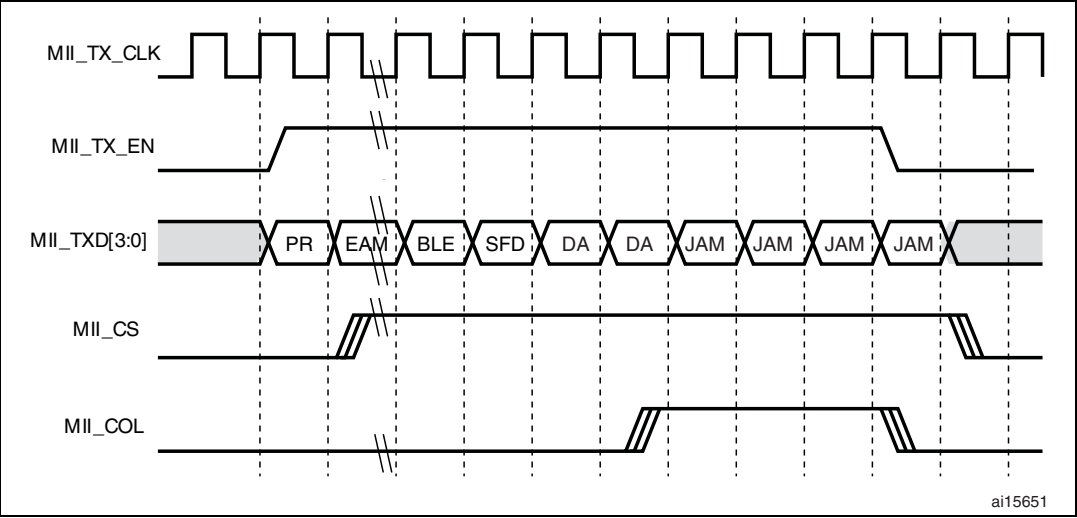
Figure 335. Transmission with collision
