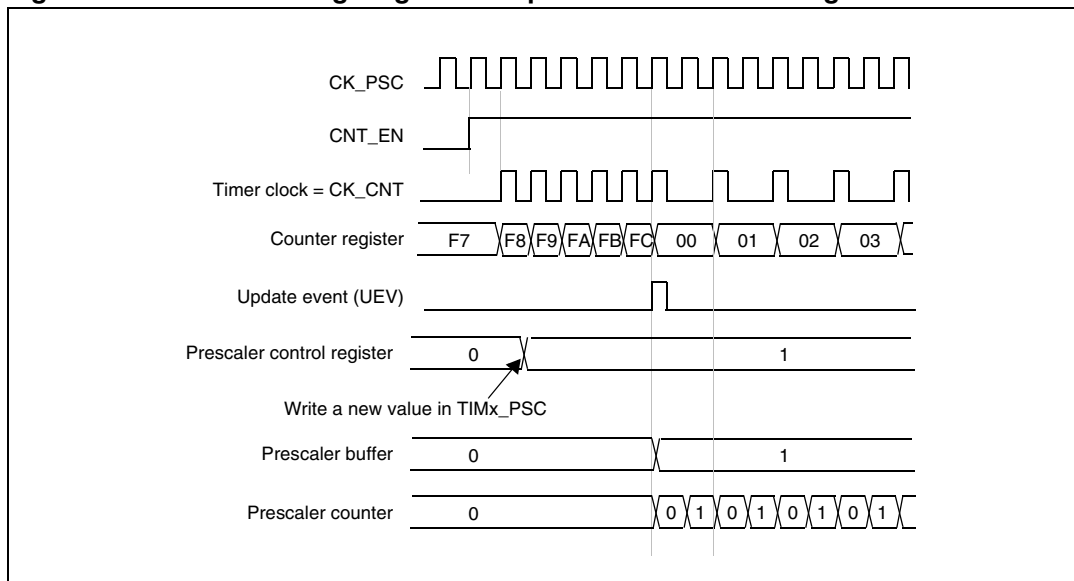
Figure 189. Counter timing diagram with prescaler division change from 1 to 2
