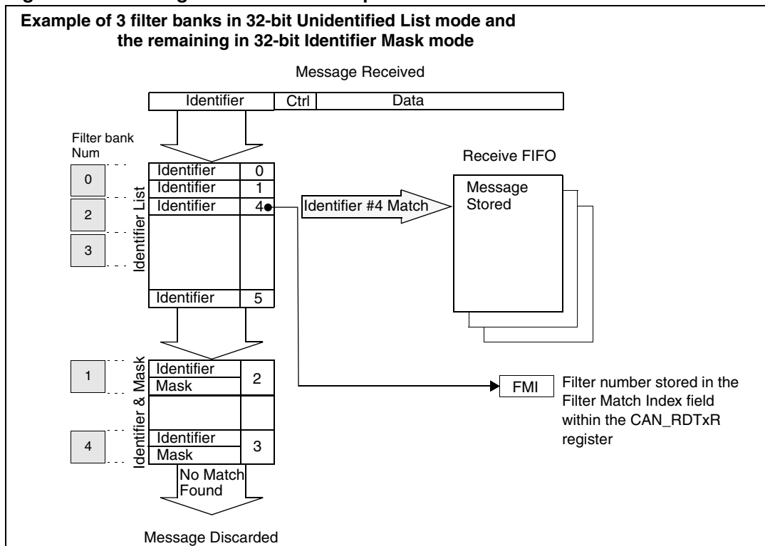
Figure 233. Filtering mechanism - example
