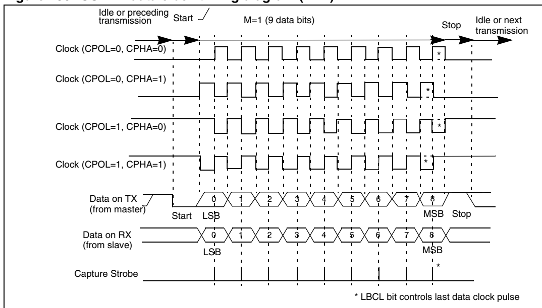
Figure 259. USART data clock timing diagram (M=1)
