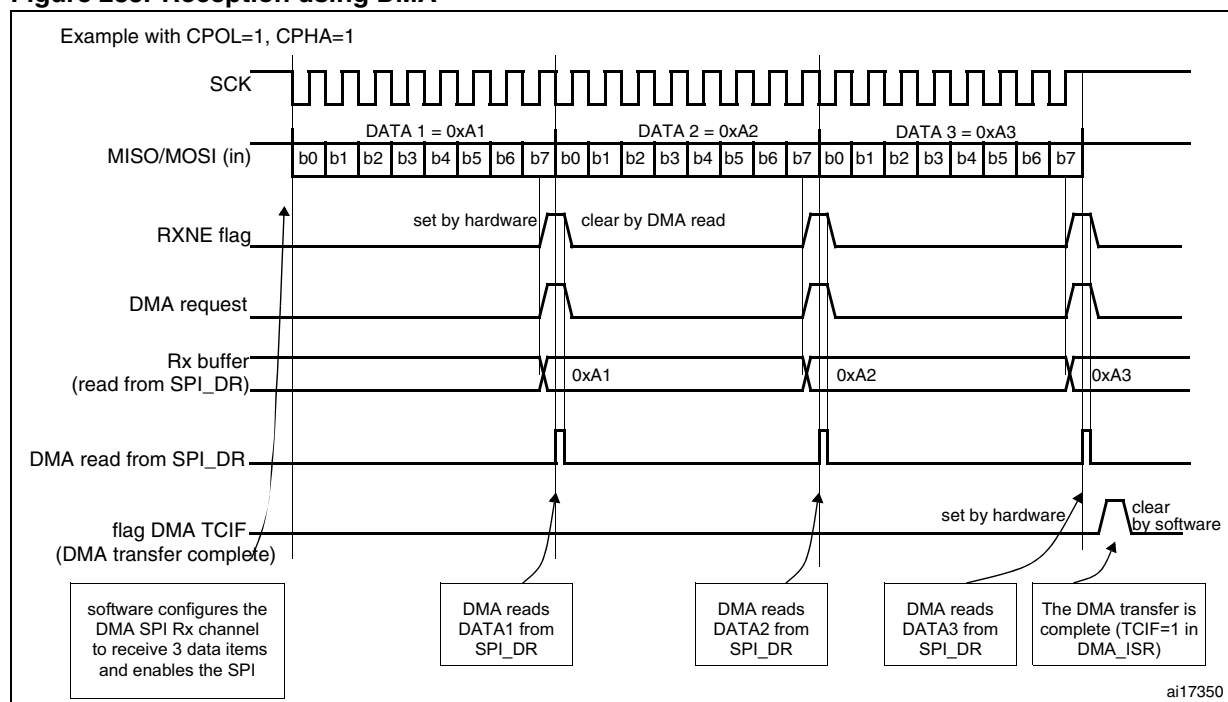
Figure 285. Reception using DMA
