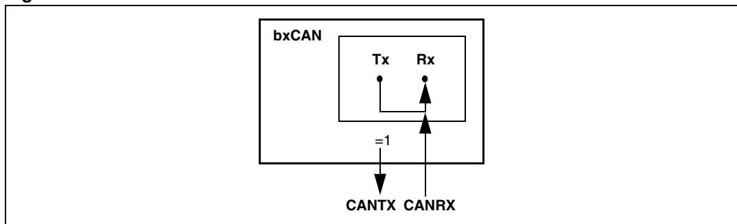
Figure 226. bxCAN in silent mode
