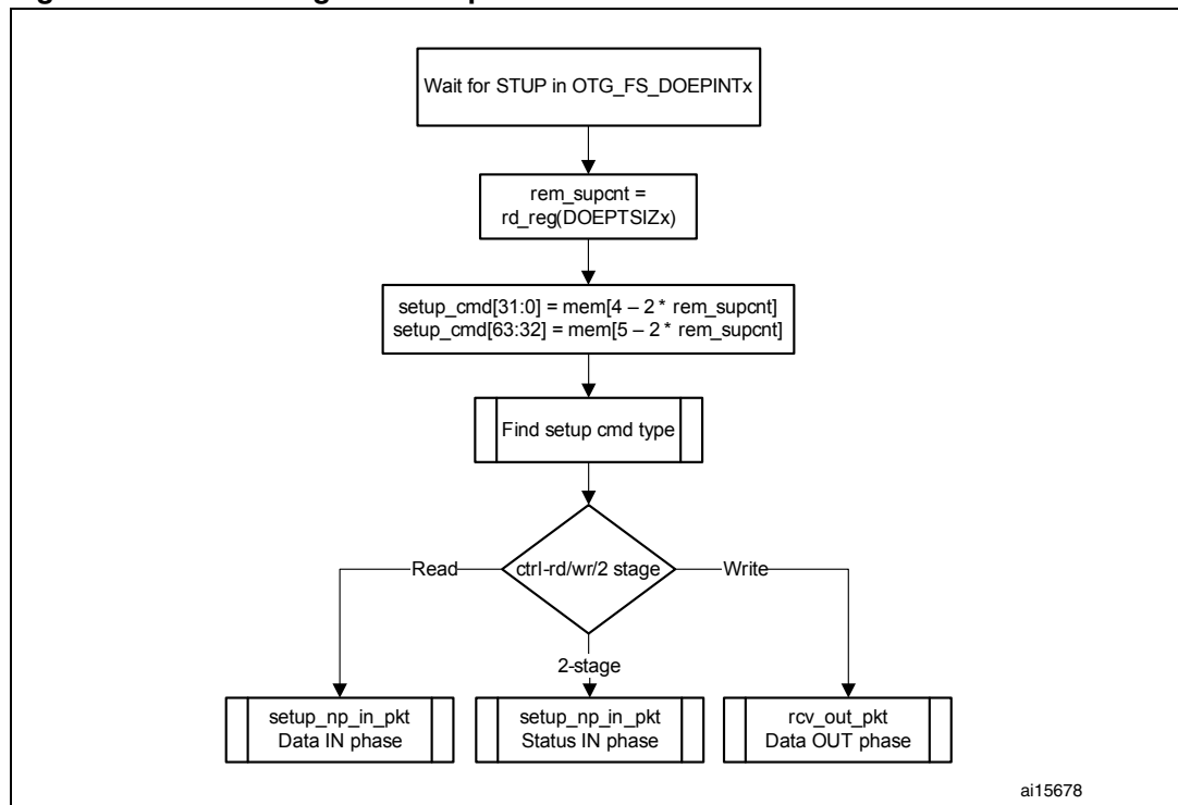
Figure 374. Processing a SETUP packet
