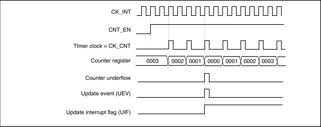
Figure 134. Counter timing diagram, internal clock divided by 2
