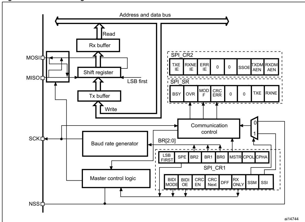
Figure 271. SPI block diagram
