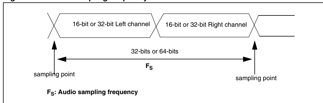
Figure 306. Audio sampling frequency definition
