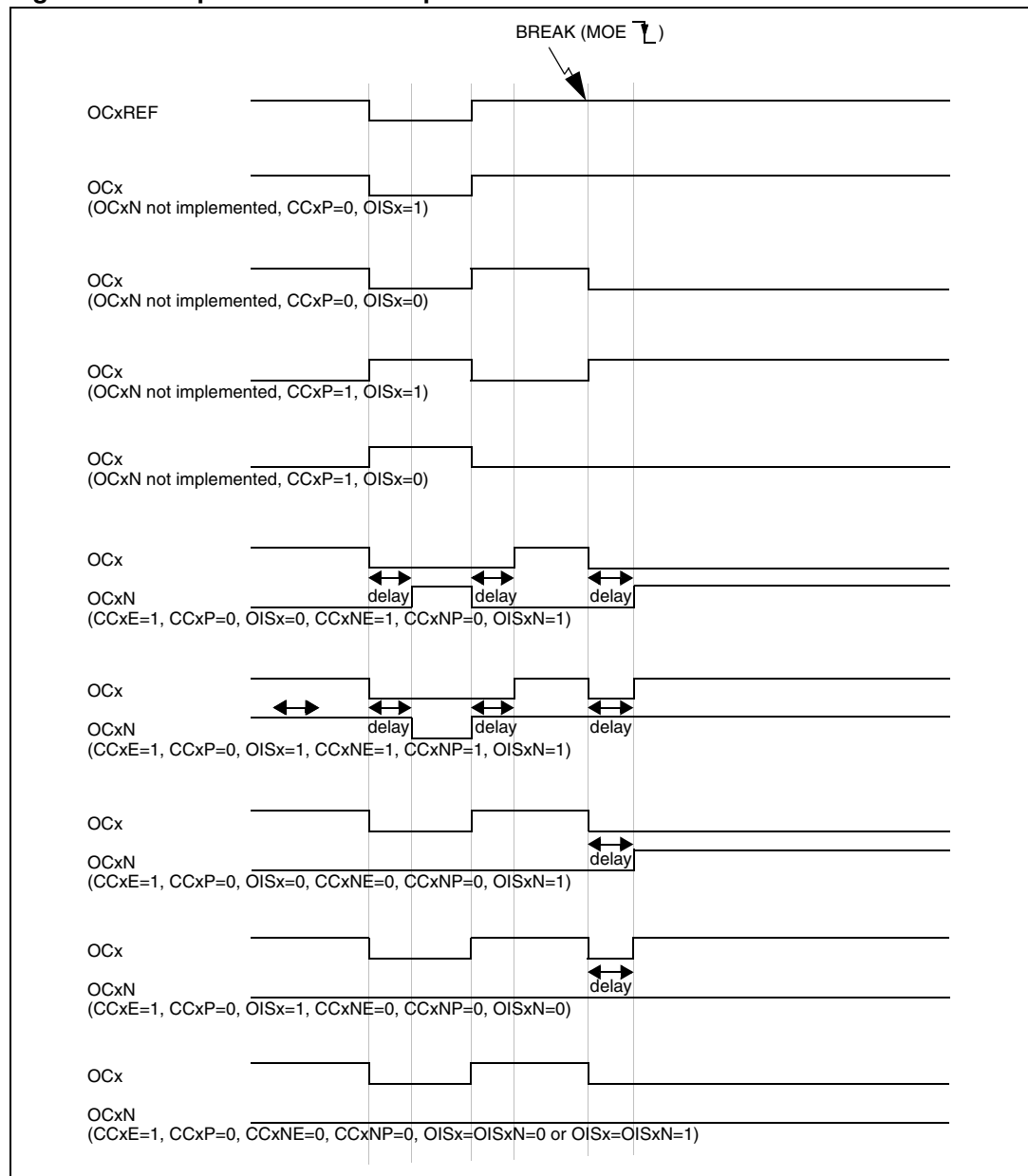
Figure 108. Output behavior in response to a break.
