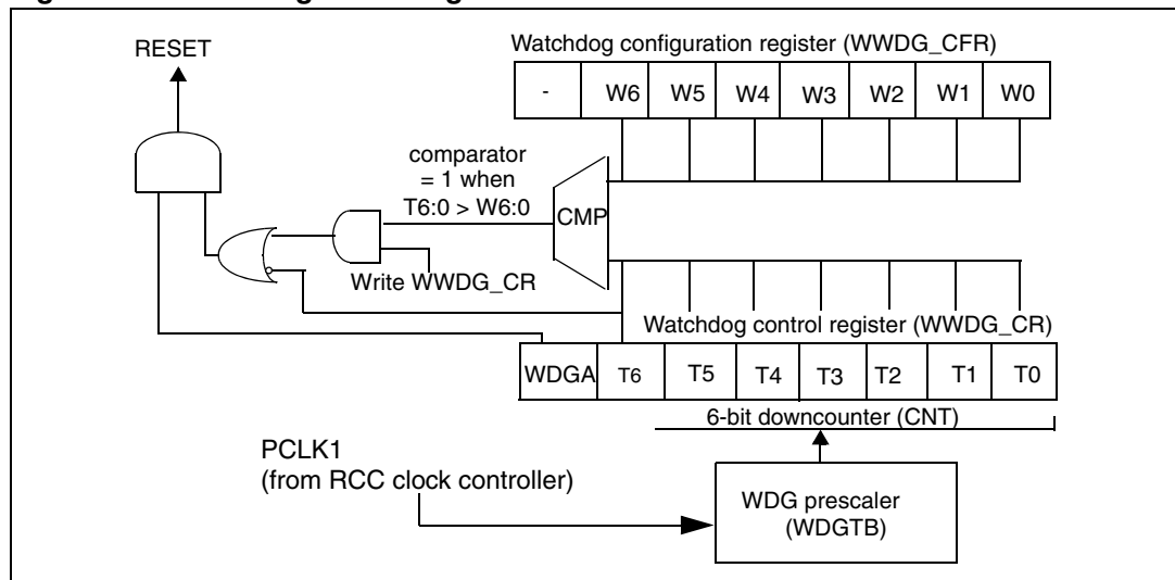
Figure 199. Watchdog block diagram
