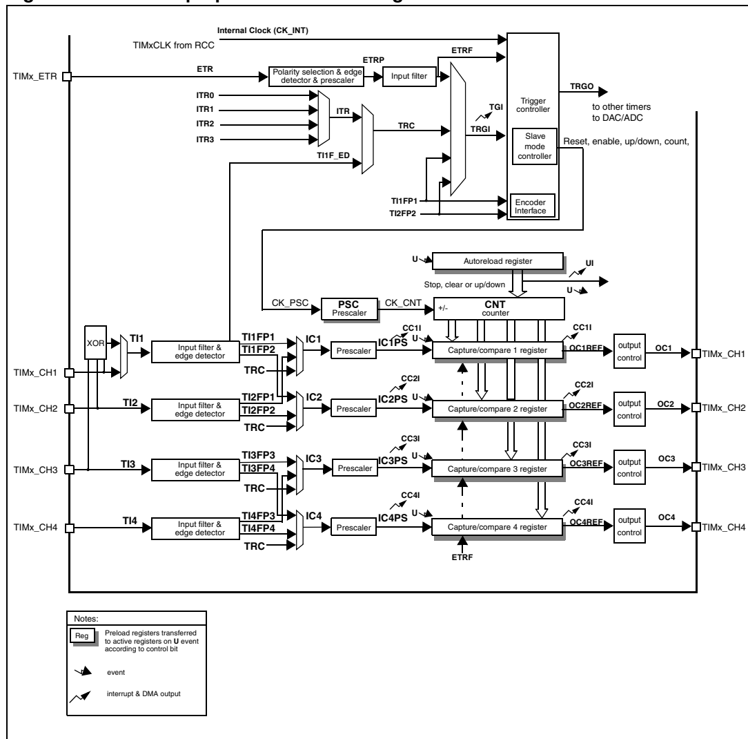
Figure 119. General-purpose timer block diagram
