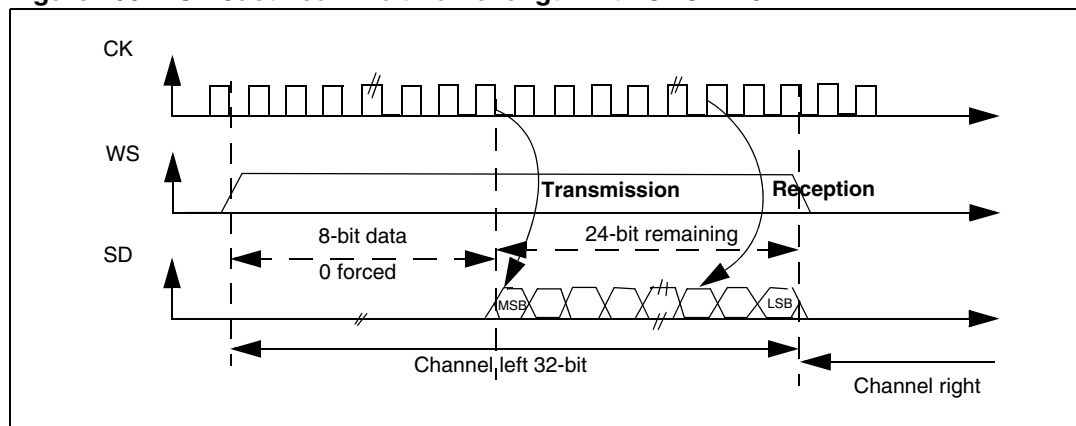
Figure 299. LSB Justified 24-bit frame length with CPOL = 0
