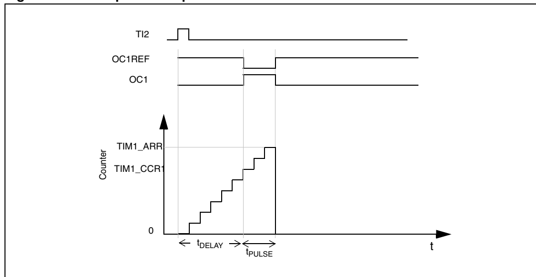
Figure 184. Example of one pulse mode.
