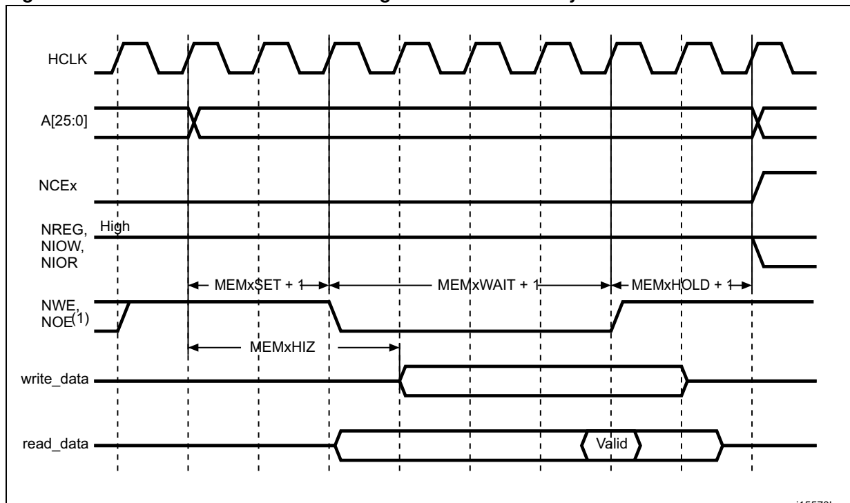
Figure 423. NAND/PC Card controller timing for common memory access
