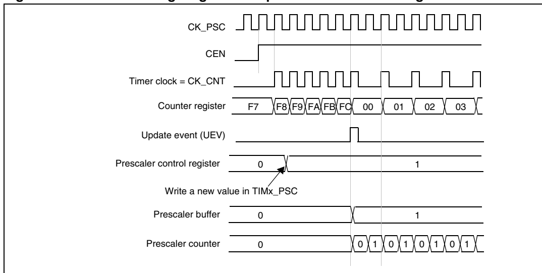
Figure 167. Counter timing diagram with prescaler division change from 1 to 2
