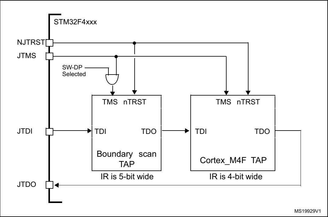
Figure 427. JTAG TAP connections
