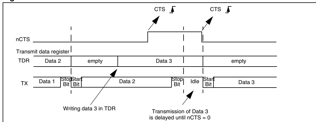
Figure 269. CTS flow control
