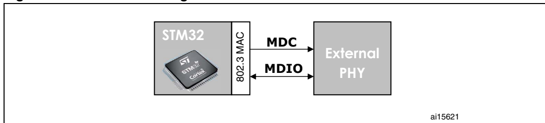
Figure 322. SMI interface signals
