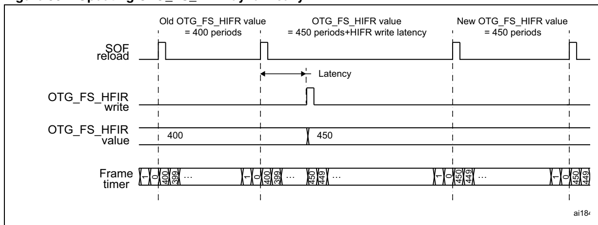
Figure 362. Updating OTG_FS_HFIR dynamically
