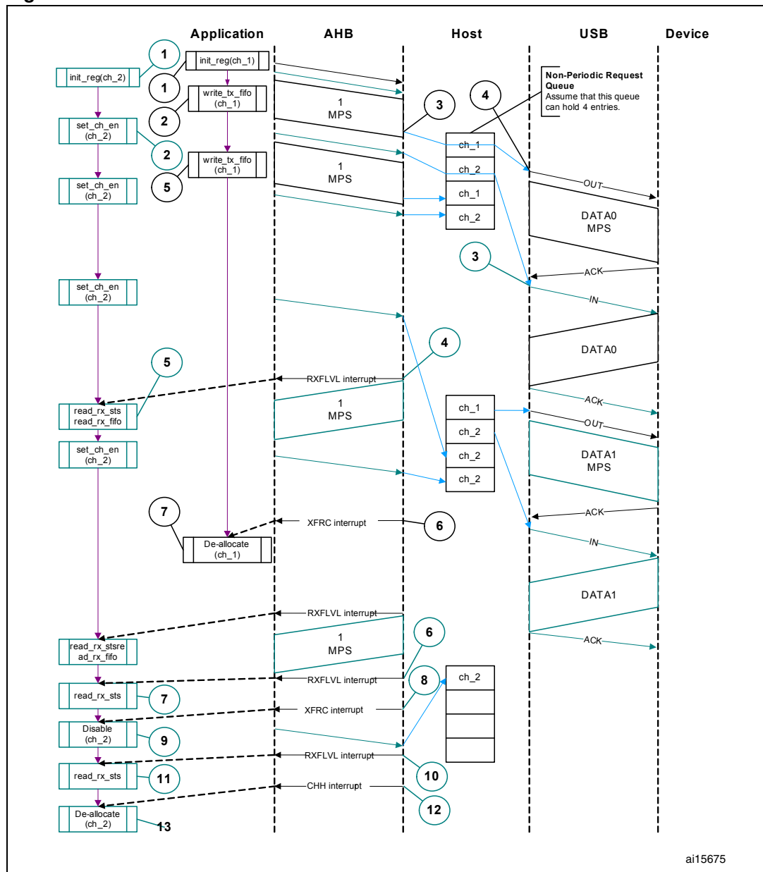
Figure 369. Normal bulk/control OUT/SETUP and bulk/control IN transactions
