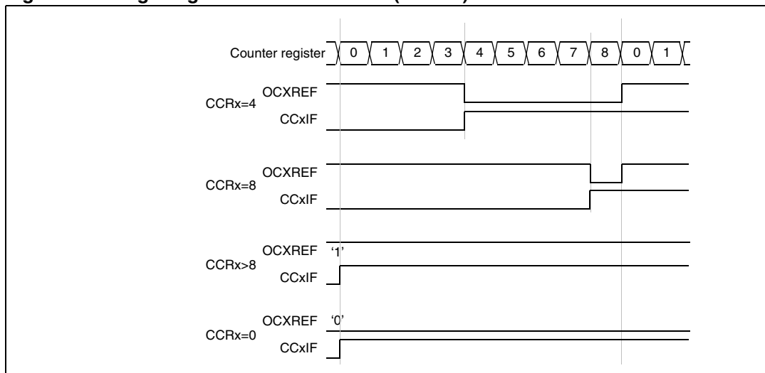
Figure 103. Edge-aligned PWM waveforms (ARR=8)
