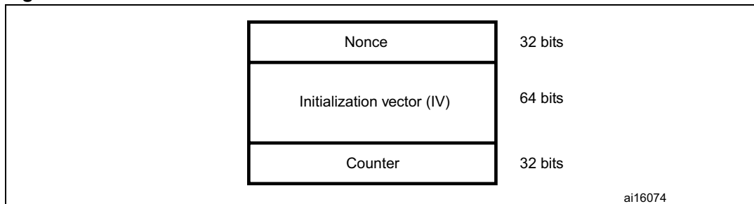
Figure 213. Initial counter block structure for the Counter mode
