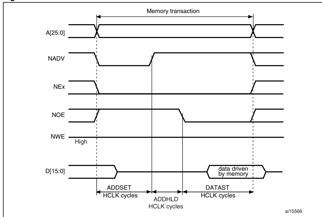
Figure 414. Mode D read accesses
