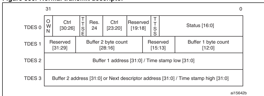
Figure 350. Normal transmit descriptor
