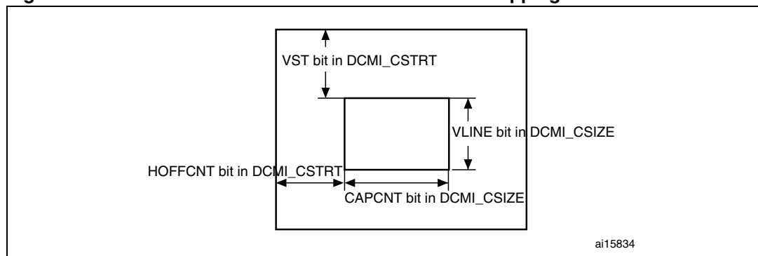
Figure 68. Coordinates and size of the window after cropping
