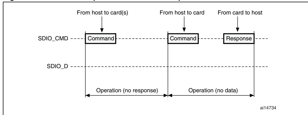
Figure 308. SDIO “no response” and “no data” operations
