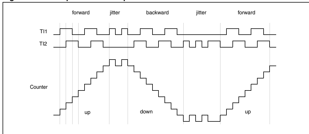
Figure 112. Example of counter operation in encoder interface mode.
