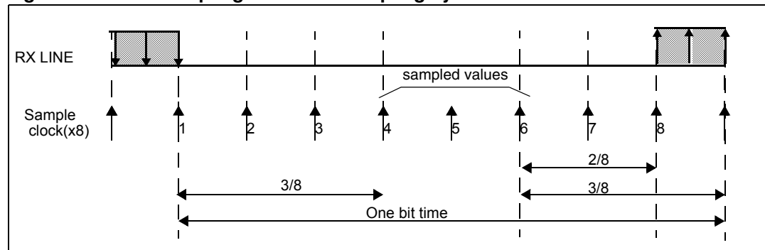
Figure 252. Data sampling when oversampling by 8
