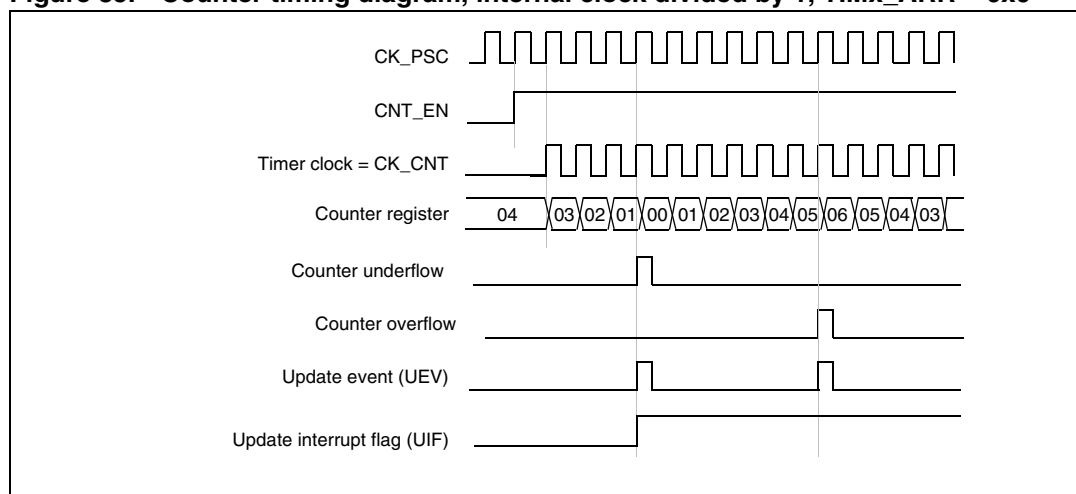
Figure 85. Counter timing diagram, internal clock divided by 1, TIMx_ARR = 0x6
