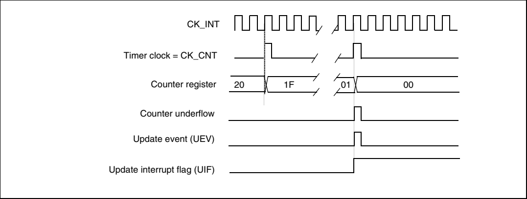
Figure 136. Counter timing diagram, internal clock divided by N
