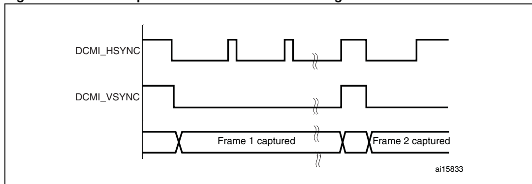
Figure 67. Frame capture waveforms in continuous grab mode
