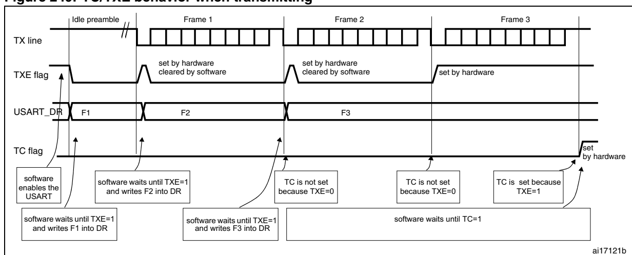
Figure 249. TC/TXE behavior when transmitting
