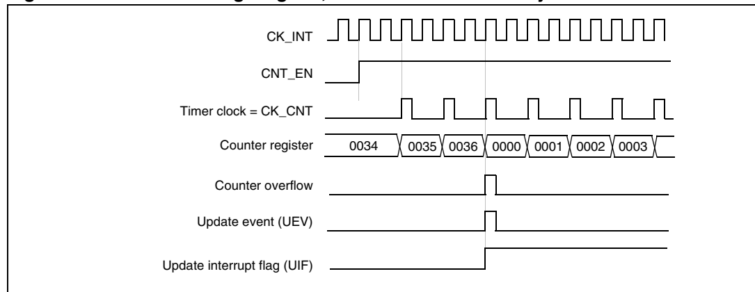
Figure 192. Counter timing diagram, internal clock divided by 2
