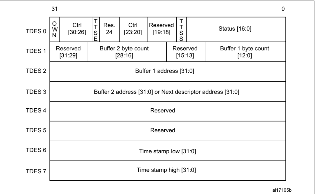
Figure 351. Enhanced transmit descriptor
