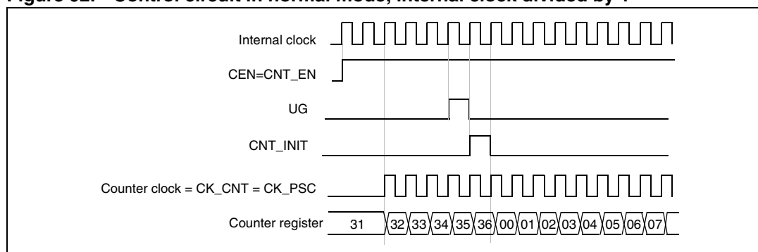
Figure 92. Control circuit in normal mode, internal clock divided by 1
