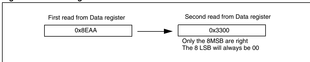
Figure 292. Receiving 0x8EAA33
