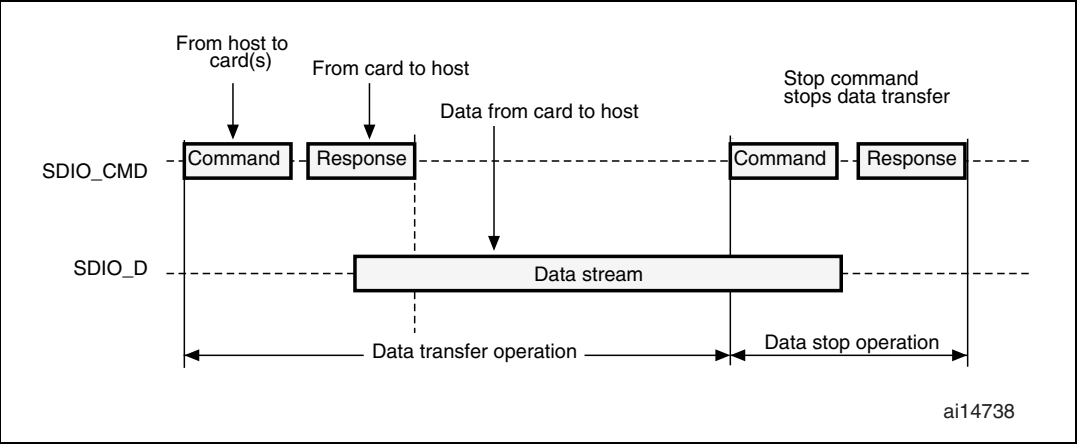
Figure 311. SDIO sequential read operation
