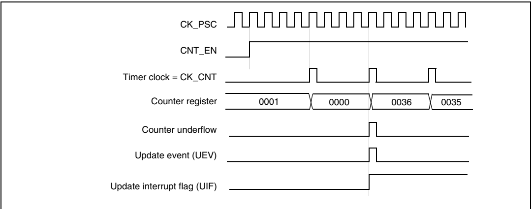
Figure 82. Counter timing diagram, internal clock divided by 4
