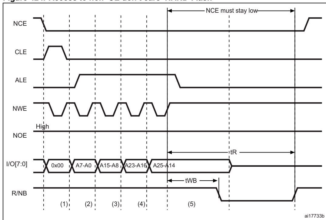
Figure 424. Access to non ‘CE don’t care’ NAND-Flash
