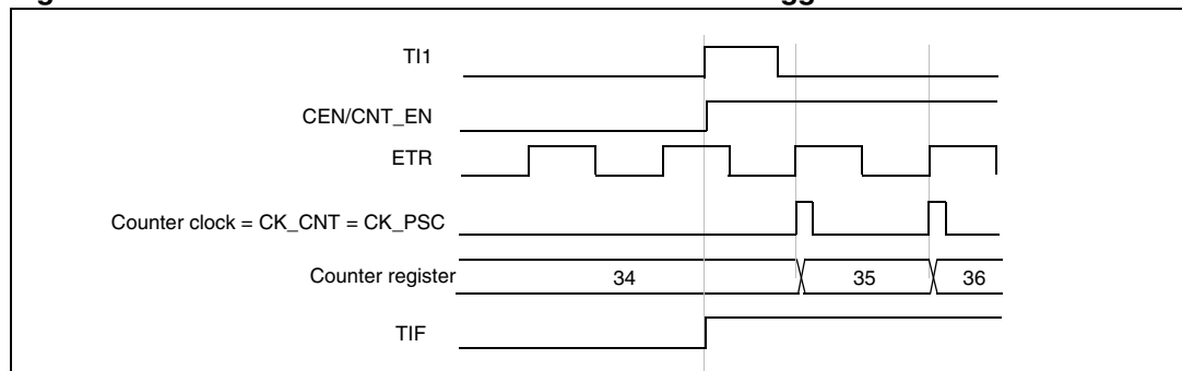
Figure 158. Control circuit in external clock mode 2 + trigger mode
