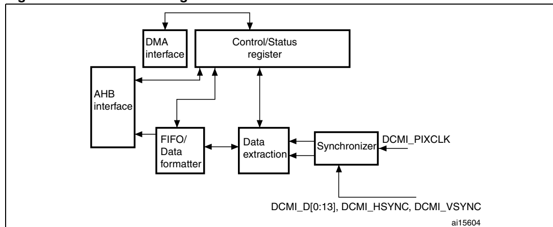
Figure 63. Top-level block diagram
