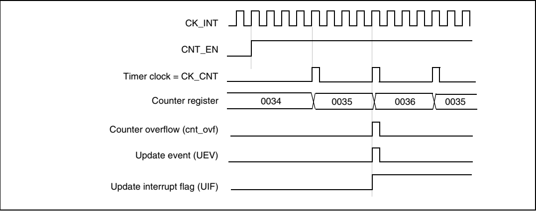
Figure 135. Counter timing diagram, internal clock divided by 4, TIMx_ARR=0x36
