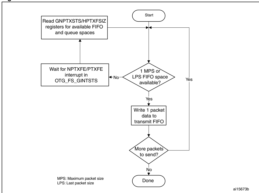
Figure 367. Transmit FIFO write task
