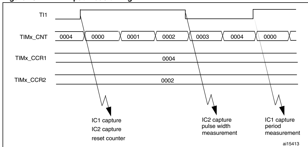
Figure 181. PWM input mode timing
