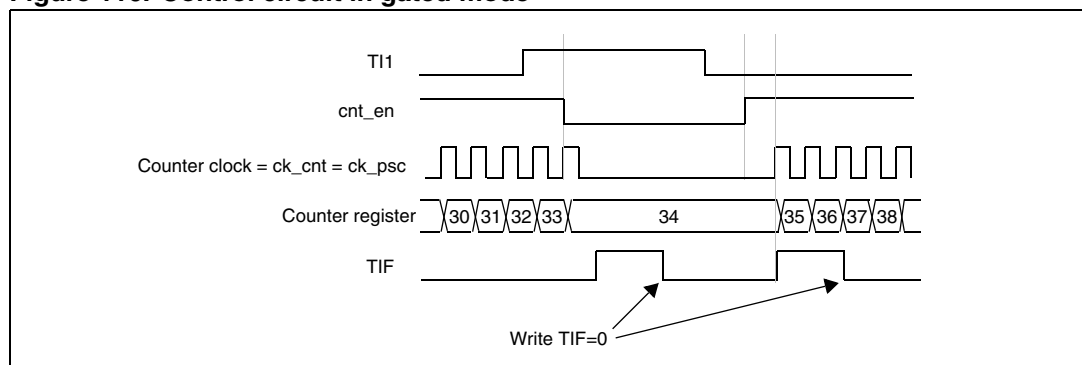
Figure 116. Control circuit in gated mode
