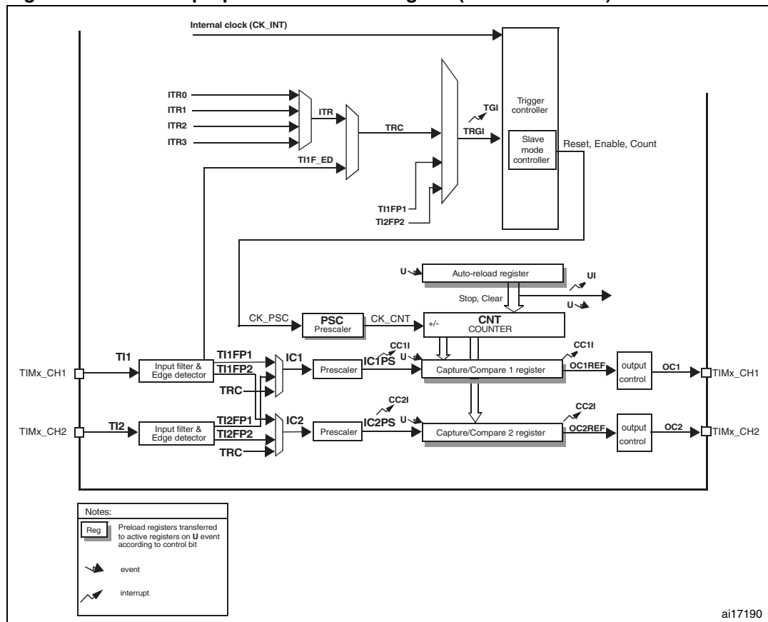
Figure 165. General-purpose timer block diagram (TIM9 and TIM12)
