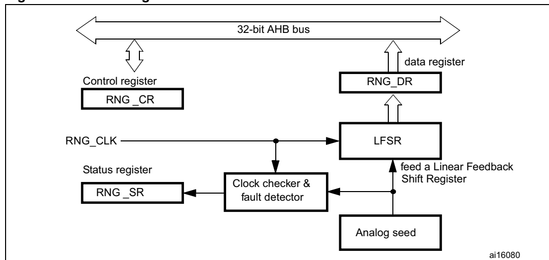
Figure 217. Block diagram
