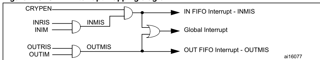
Figure 216. CRYP interrupt mapping diagram
