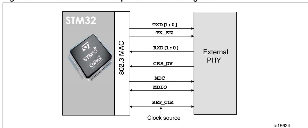
Figure 327. Reduced media-independent interface signals
