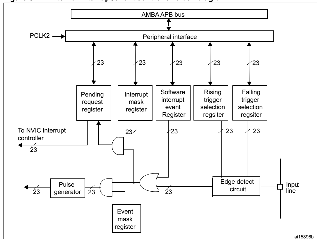
Figure 32. External interrupt/event controller block diagram
