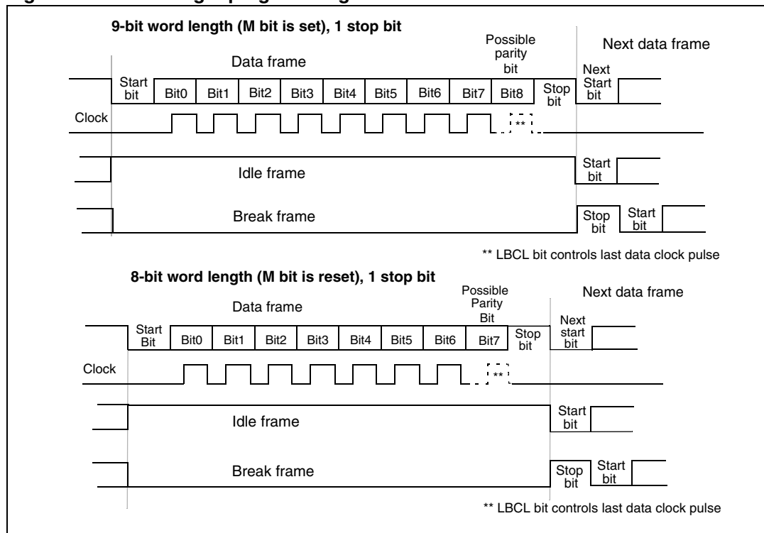
Figure 247. Word length programming
