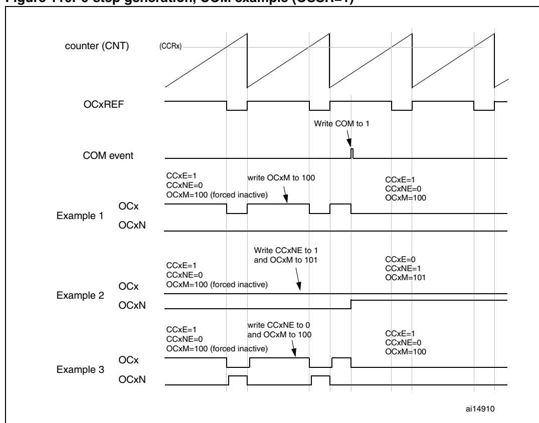
Figure 110. 6-step generation, COM example (OSSR=1)
