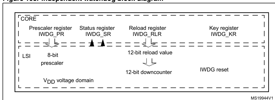
Figure 198. Independent watchdog block diagram
