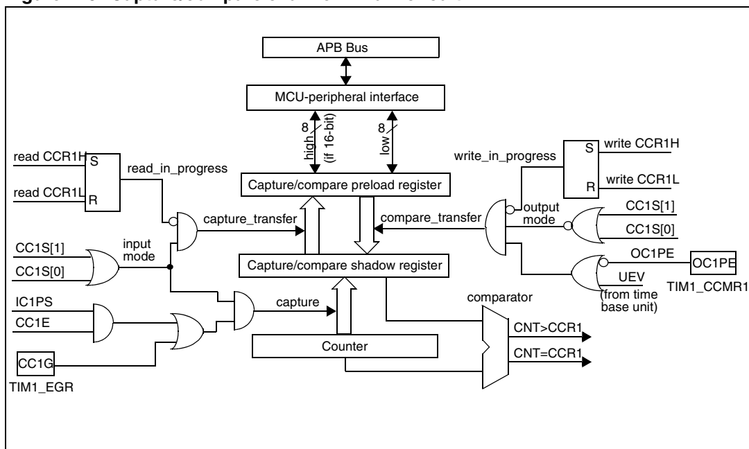
Figure 179. Capture/compare channel 1 main circuit
