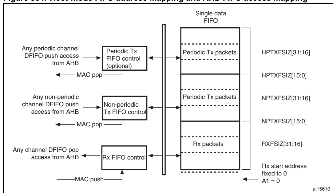
Figure 364. Host-mode FIFO address mapping and AHB FIFO access mapping
