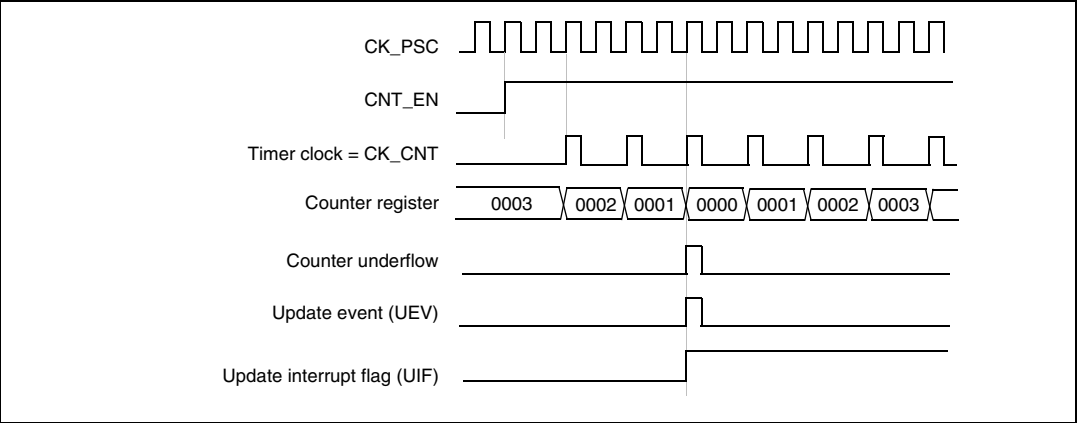
Figure 86. Counter timing diagram, internal clock divided by 2
