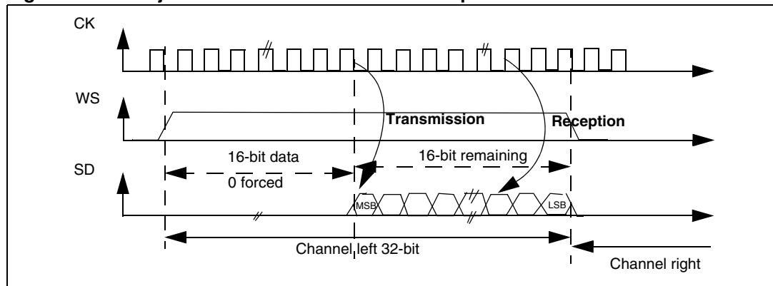
Figure 302. LSB justified 16-bit extended to 32-bit packet frame with CPOL = 0
