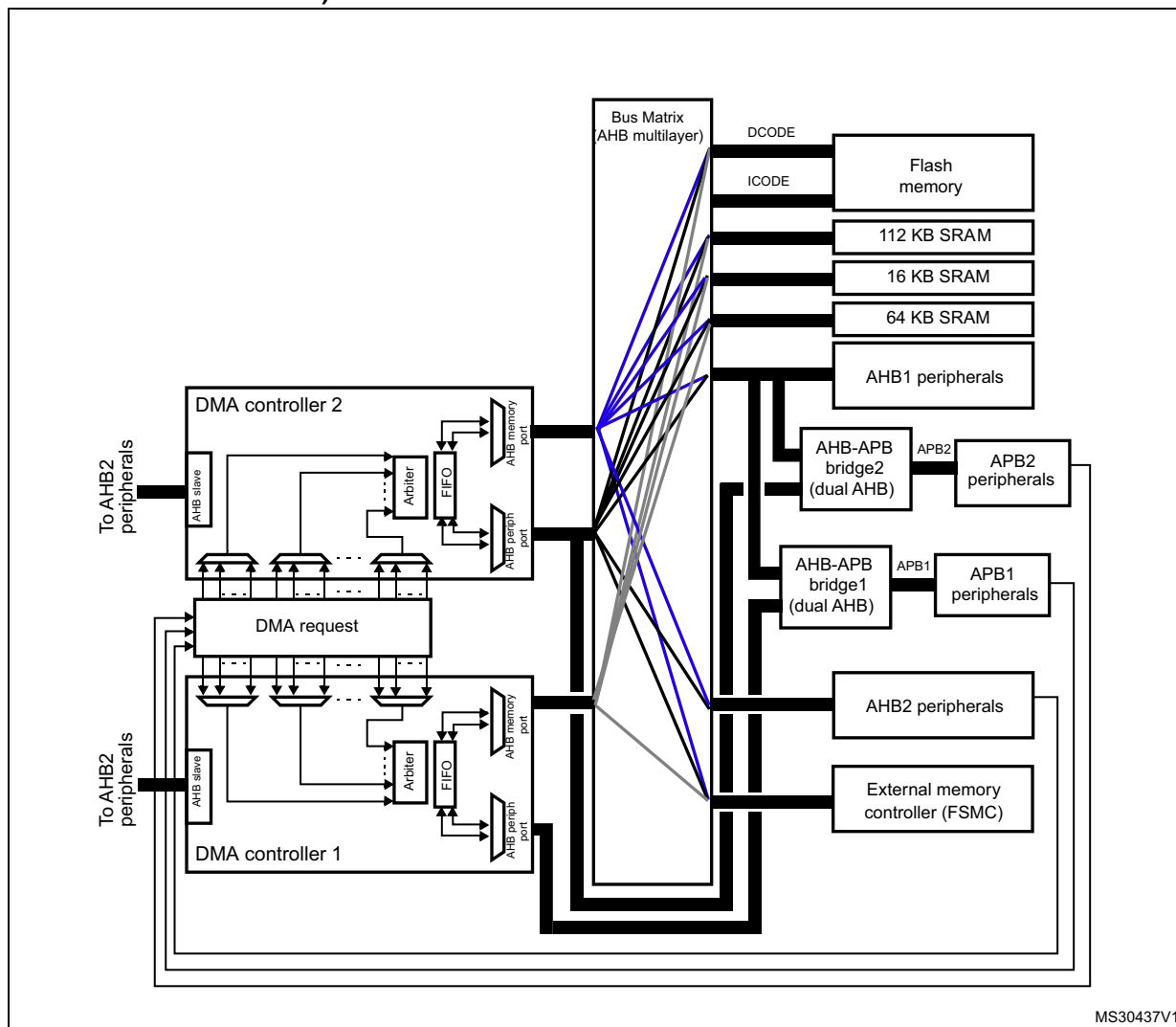
Figure 26. System implementation of the two DMA controllers (STM32F42xxx and STM32F43xxx)
