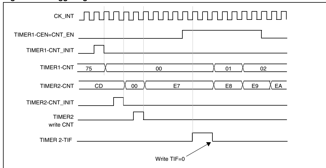
Figure 163. Triggering timer 2 with Enable of timer 1
