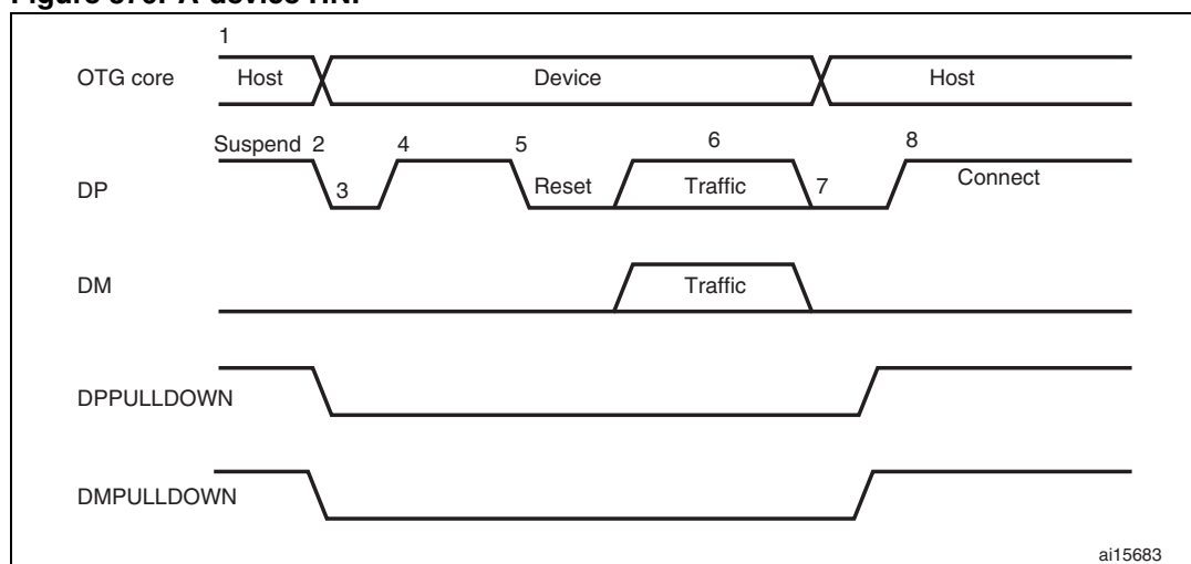
Figure 379. A-device HNP
