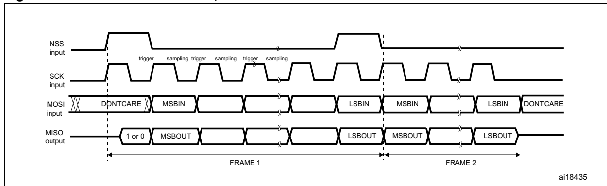
Figure 275. TI mode - Slave mode, continuous transfer
