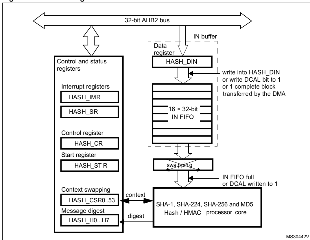
Figure 219. Block diagram for STM32F42xxx and STM32F43xxx
