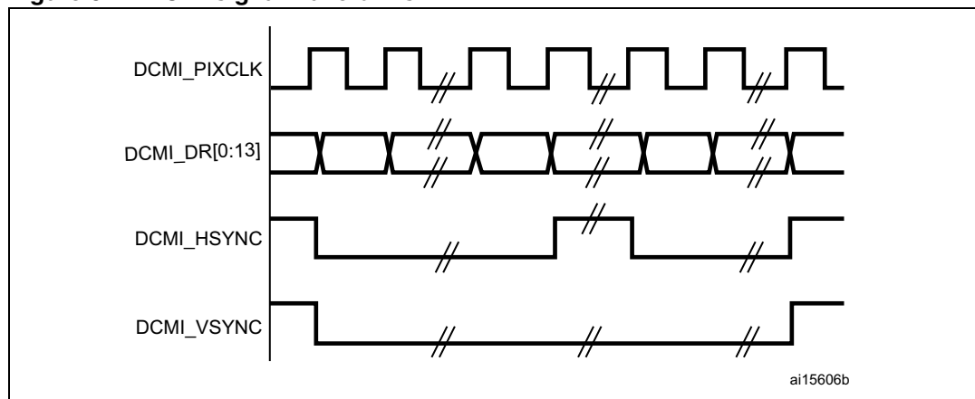
Figure 64. DCMI signal waveforms
