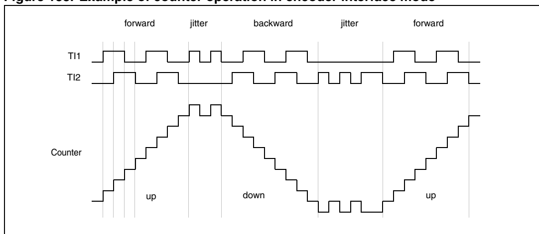
Figure 153. Example of counter operation in encoder interface mode
