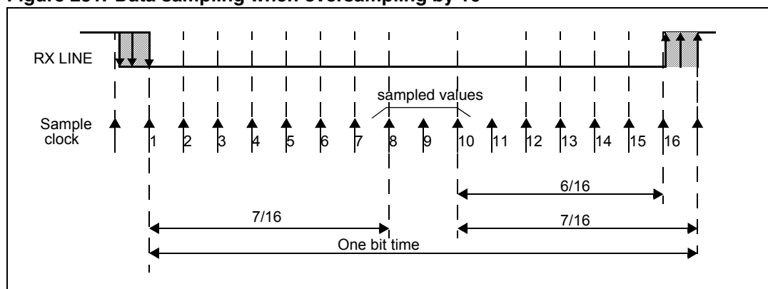
Figure 251. Data sampling when oversampling by 16
