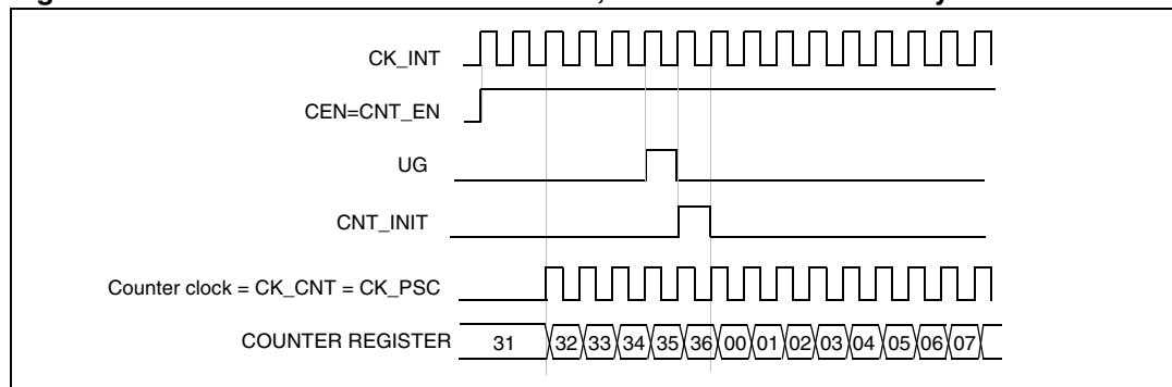
Figure 139. Control circuit in normal mode, internal clock divided by 1
