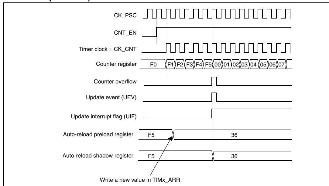
Figure 127. Counter timing diagram, Update event when ARPE=1 (TIMx_ARR preloaded)
