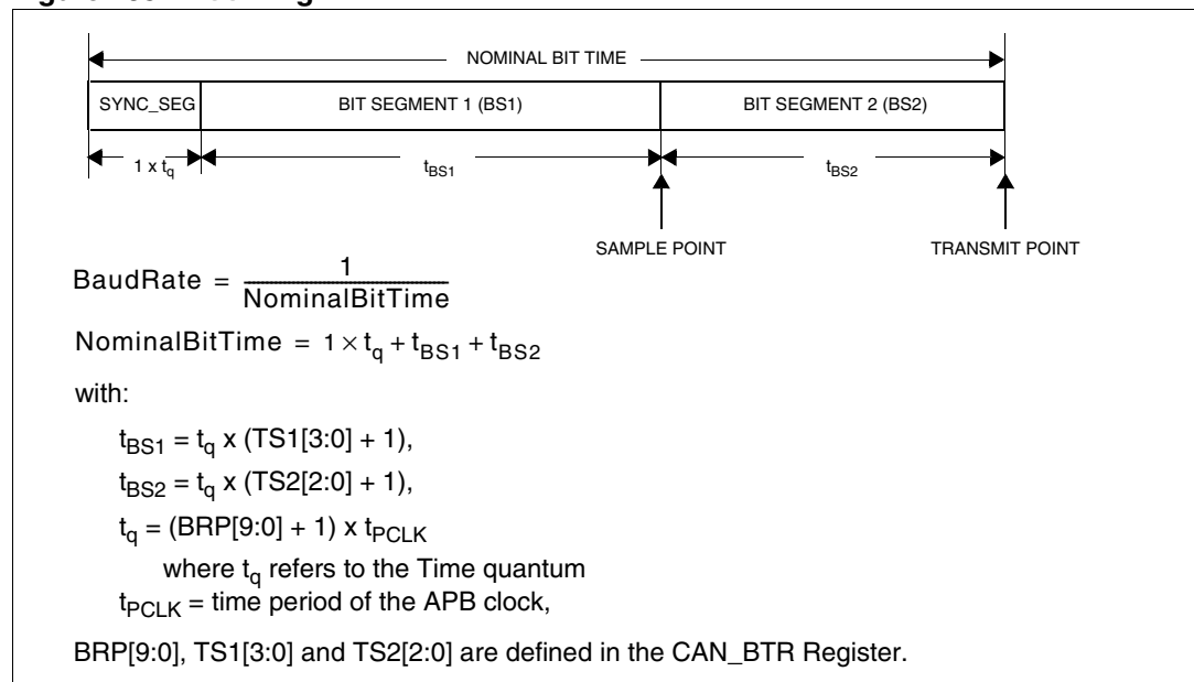
Figure 235. Bit timing
