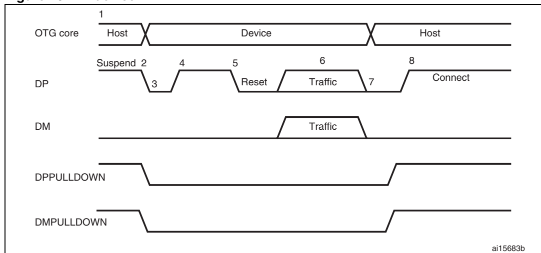
Figure 401. A-device HNP
