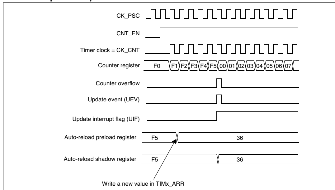
Figure 196. Counter timing diagram, update event when ARPE=1 (TIMx_ARR preloaded)
