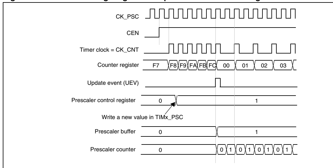
Figure 72. Counter timing diagram with prescaler division change from 1 to 2
