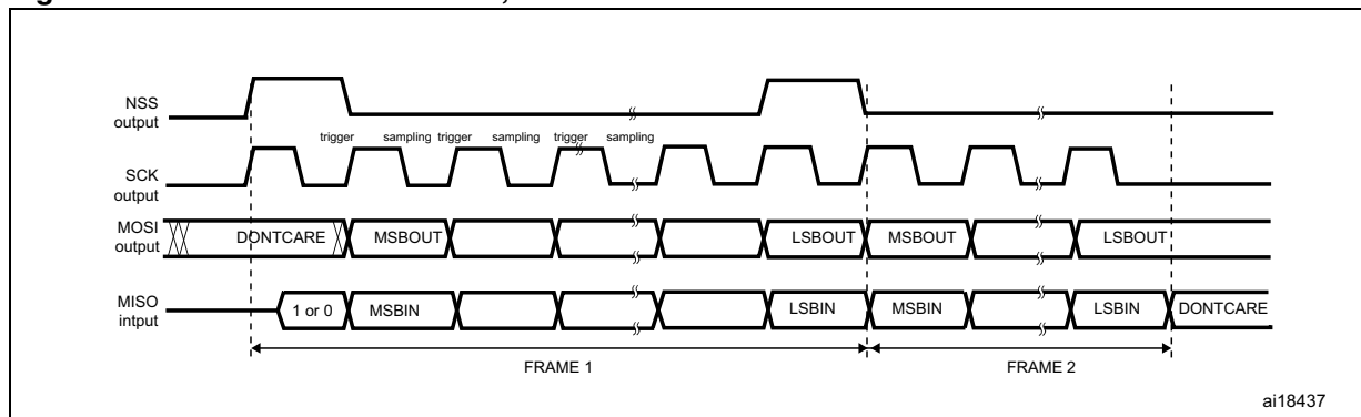
Figure 277. TI mode - master mode, continuous transfer
