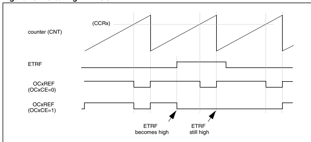
Figure 152. Clearing TIMx OCxREF
