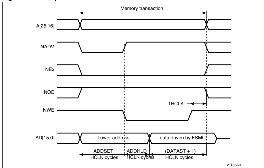
Figure 417. Multiplexed write accesses
