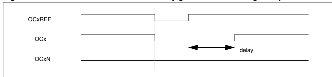
Figure 106. Dead-time waveforms with delay greater than the negative pulse.
