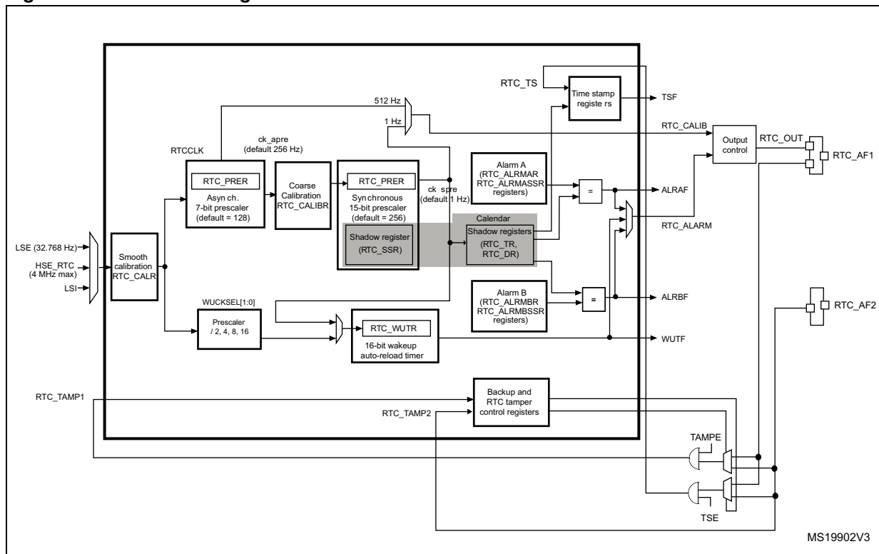
Figure 222. RTC block diagram
