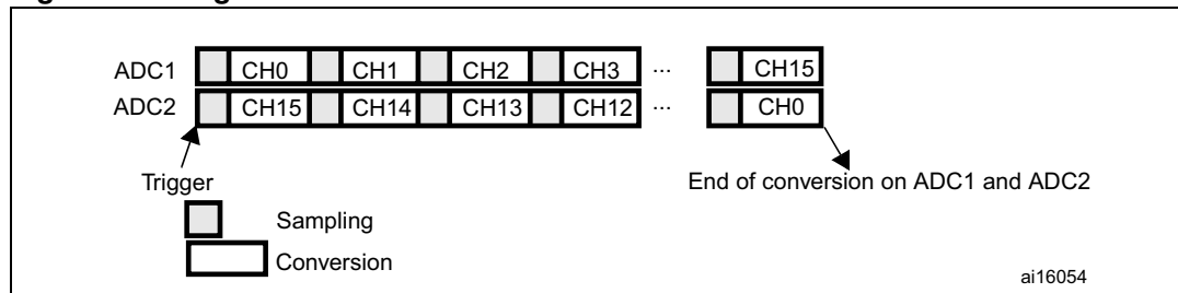
Figure 44. Regular simultaneous mode on 16 channels: dual ADC mode
