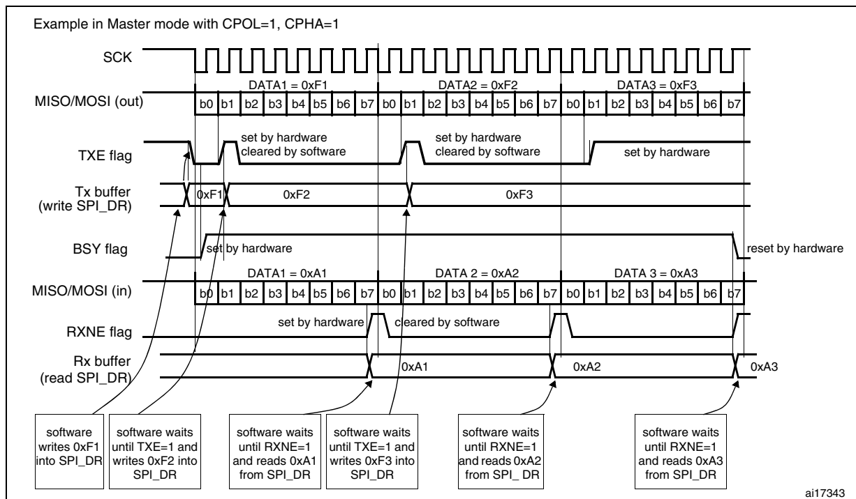
Figure 278. TXE/RXNE/BSY behavior in Master / full-duplex mode (BIDIMODE=0 and RXONLY=0) in the case of continuous transfers
