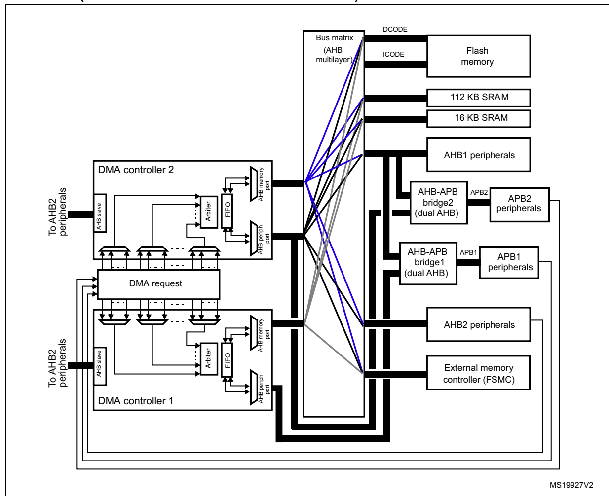
Figure 25. System implementation of the two DMA controllers (STM32F405xx/07xx and STM32F415xx/17xx)
