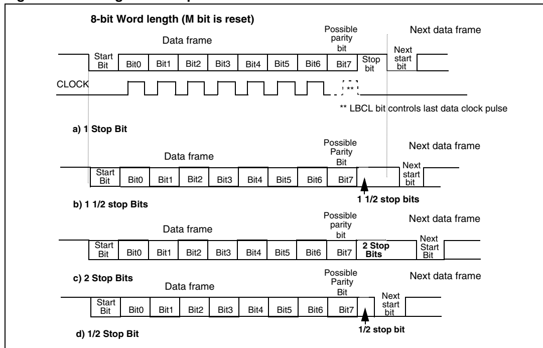
Figure 248. Configurable stop bits
