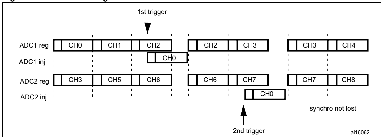
Figure 51. Alternate + regular simultaneous
