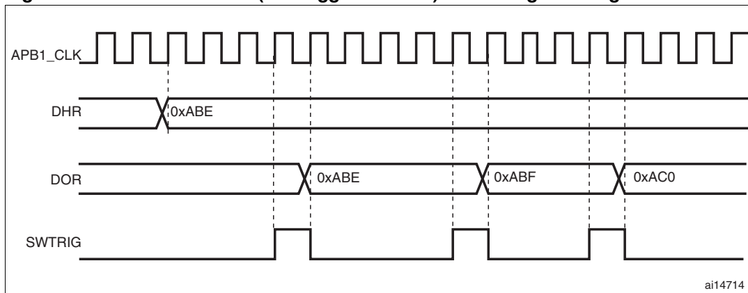
Figure 61. DAC conversion (SW trigger enabled) with triangle wave generation
