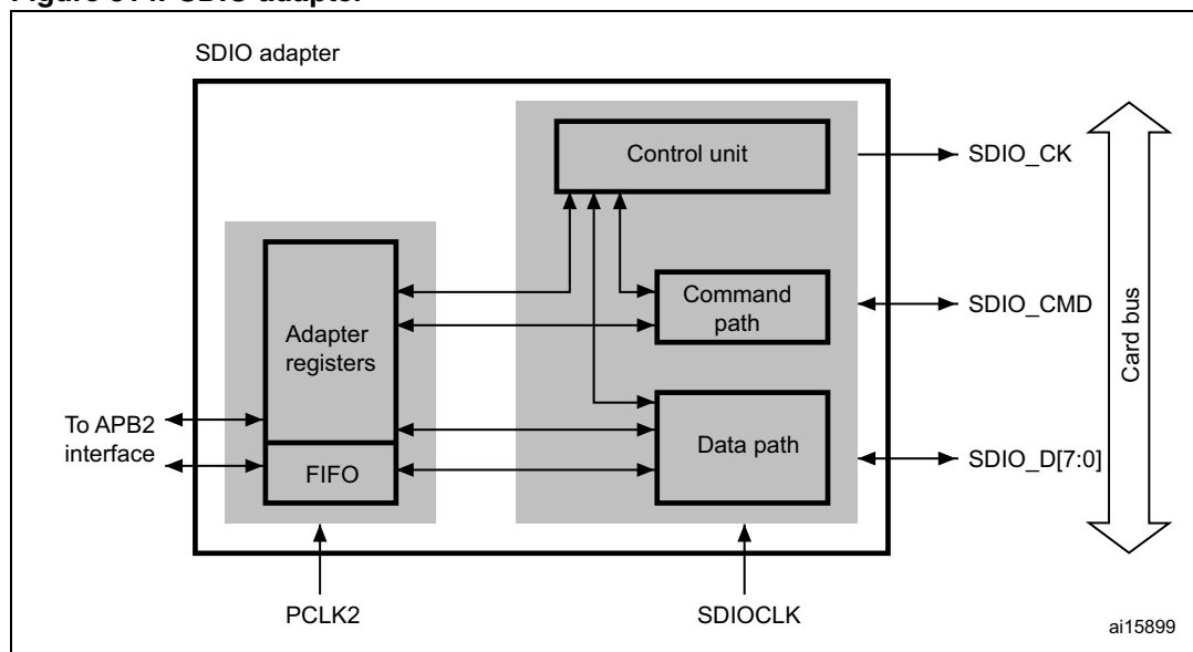
Figure 314. SDIO adapter
