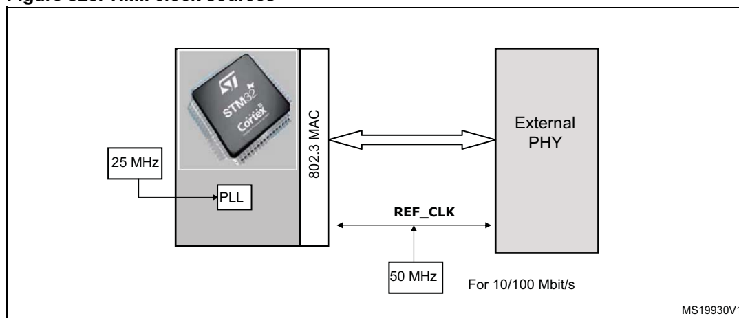
Figure 328. RMII clock sources
