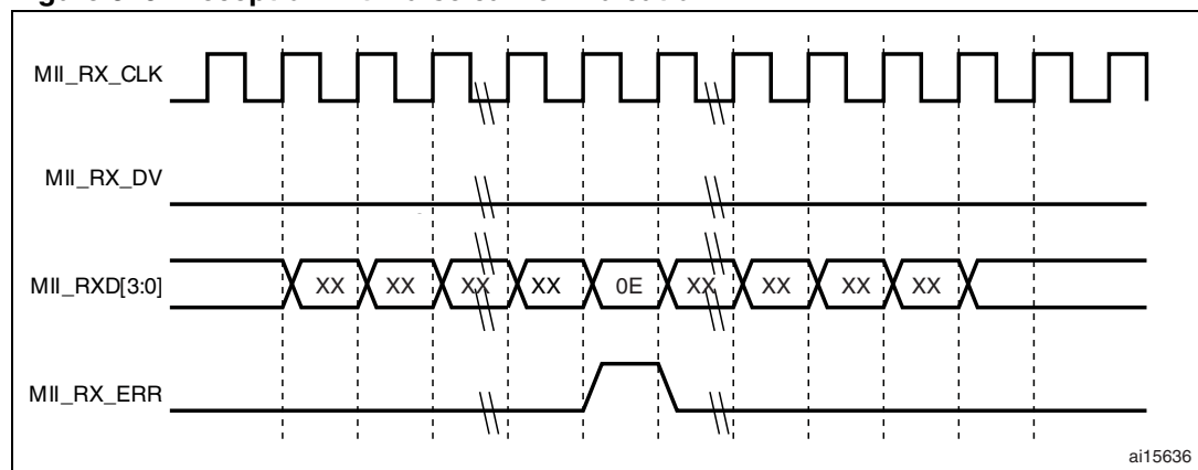
Figure 340. Reception with false carrier indication
