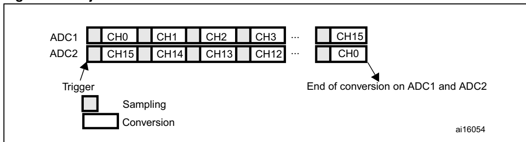
Figure 42. Injected simultaneous mode on 4 channels: dual ADC mode
