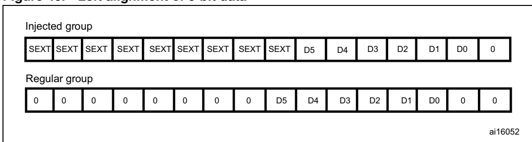
Figure 40. Left alignment of 6-bit data
