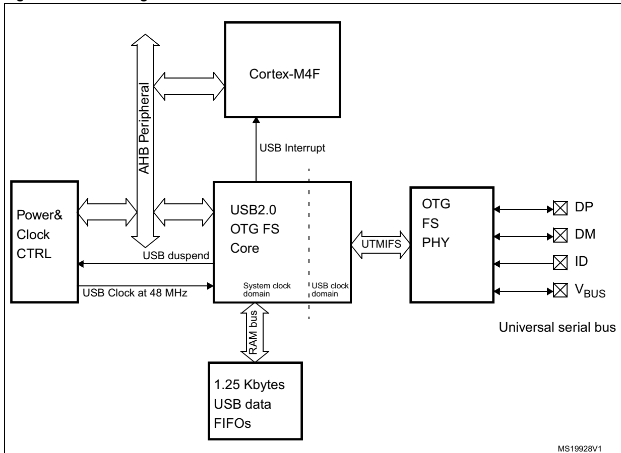
Figure 357. Block diagram
