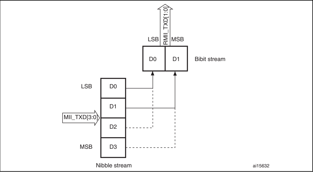
Figure 333. Transmission bit order
