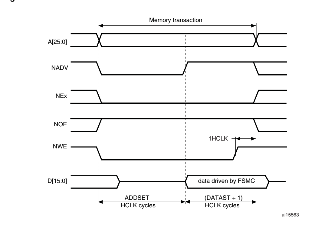
Figure 411. ModeB write accesses
