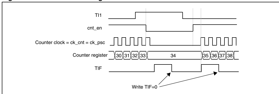
Figure 186. Control circuit in gated mode
