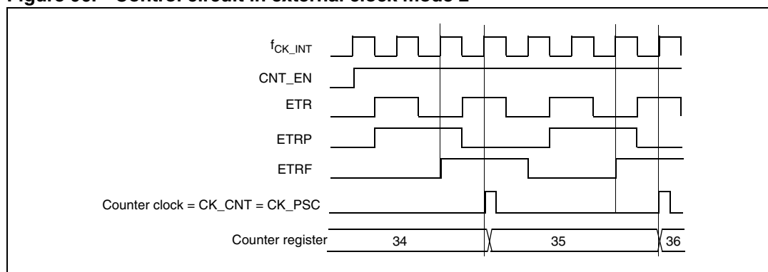
Figure 96. Control circuit in external clock mode 2
