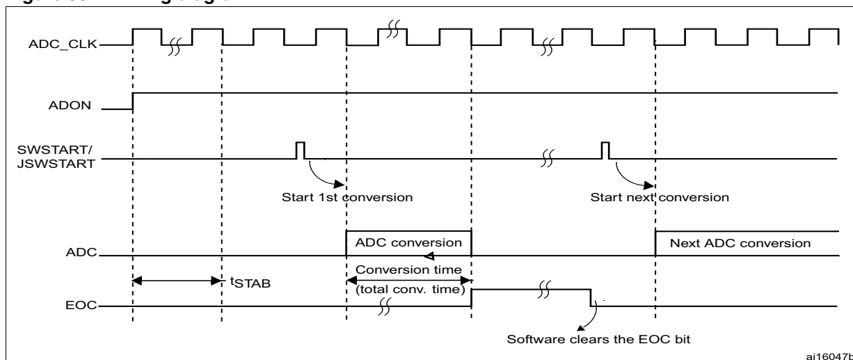
Figure 35. Timing diagram
