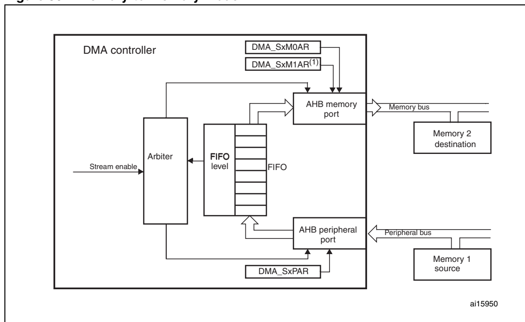
Figure 30. Memory-to-memory mode
