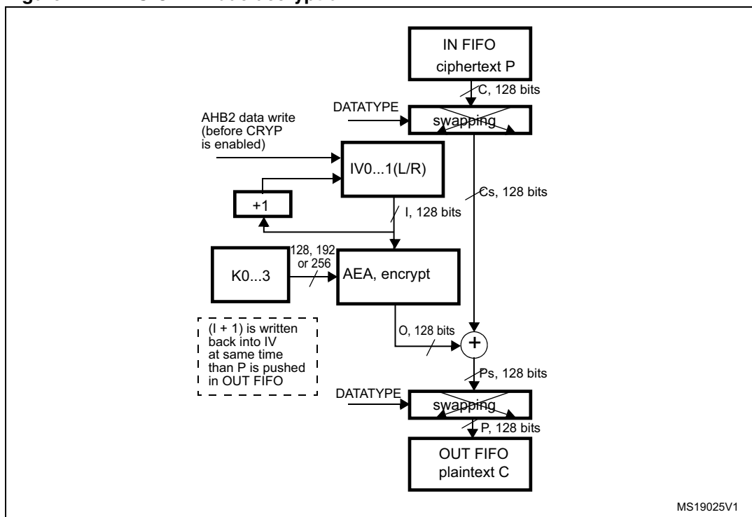
Figure 212. AES-CTR mode decryption
