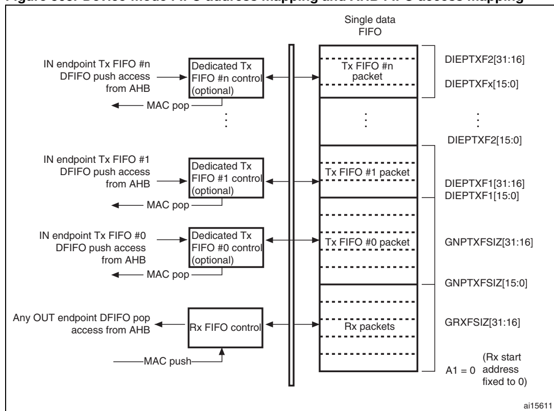
Figure 363. Device-mode FIFO address mapping and AHB FIFO access mapping
