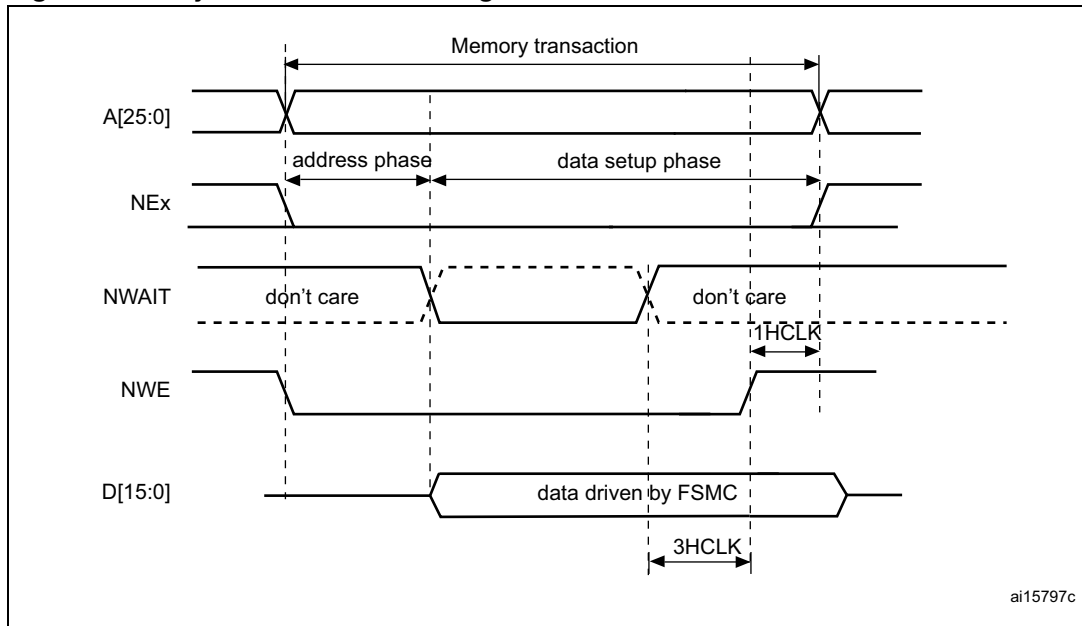
Figure 419. Asynchronous wait during a write access
