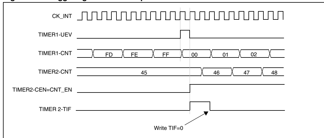
Figure 162. Triggering timer 2 with update of timer 1
