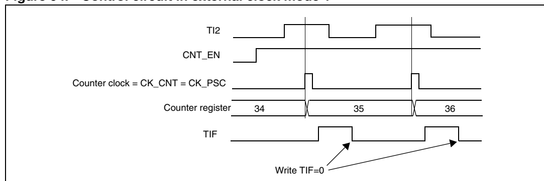
Figure 94. Control circuit in external clock mode 1
