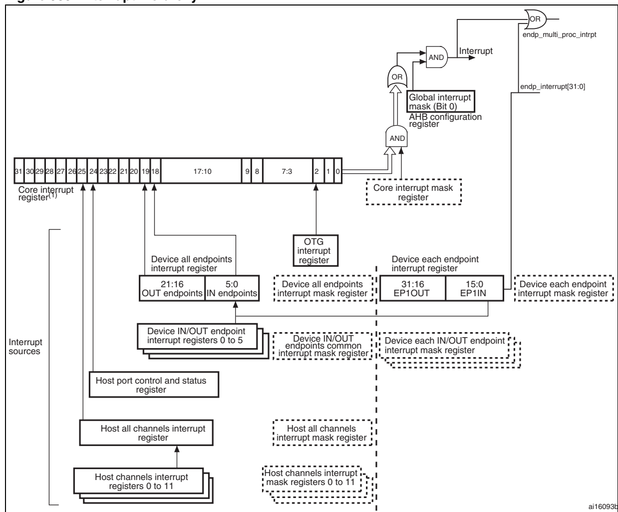
Figure 383. Interrupt hierarchy
