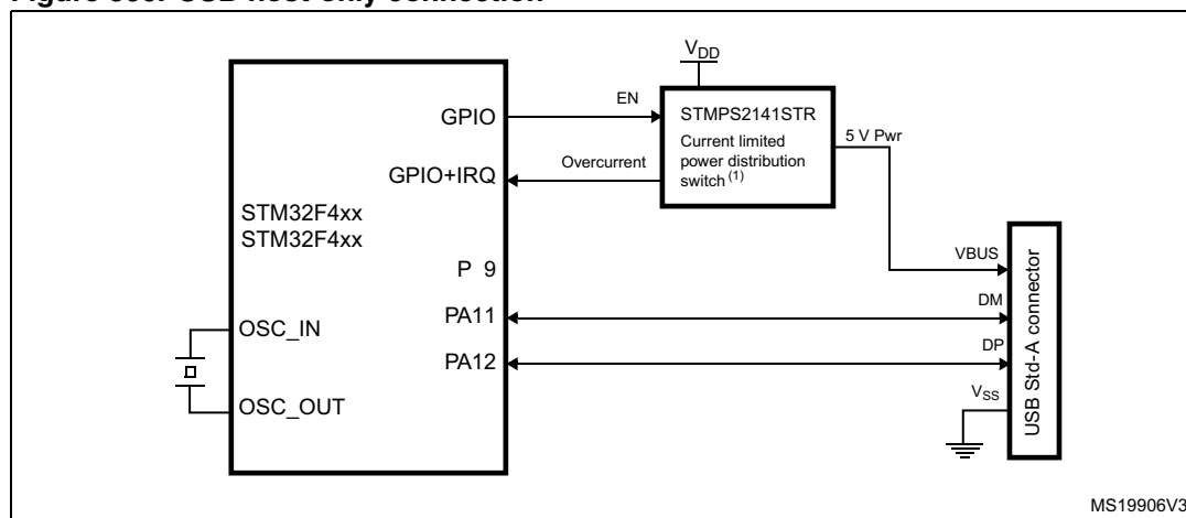
Figure 360. USB host-only connection
