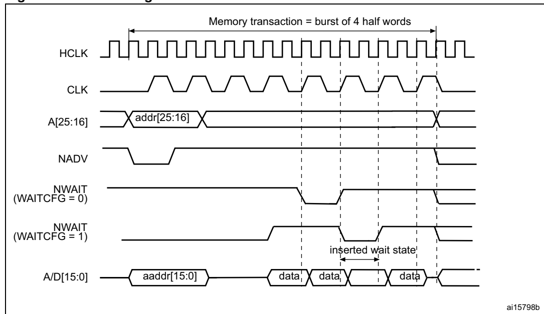
Figure 420. Wait configurations
