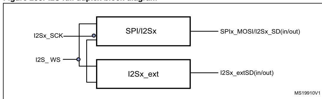
Figure 288. I2S full duplex block diagram
