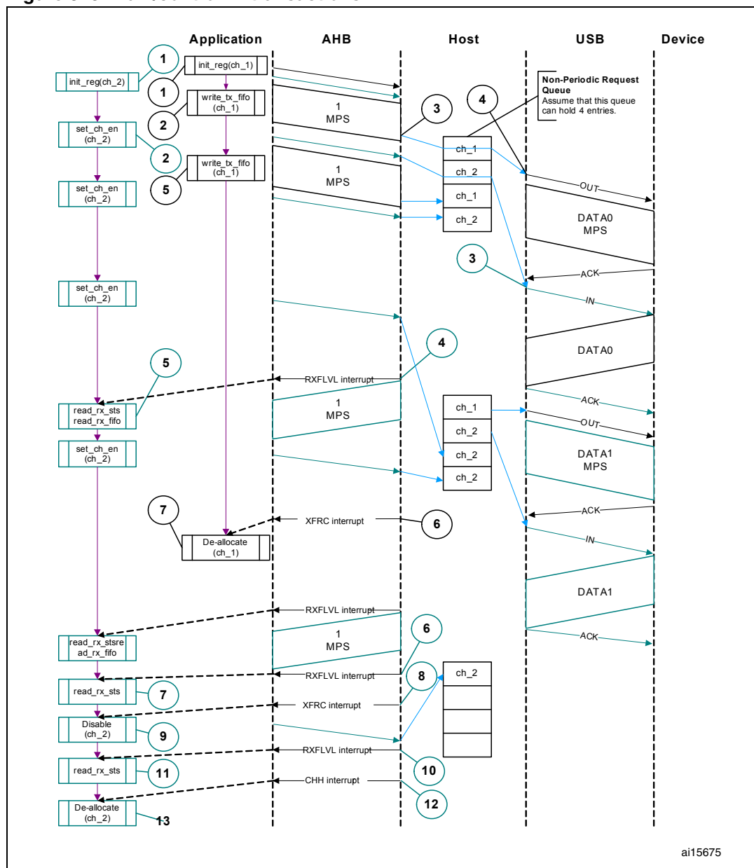
Figure 370. Bulk/control IN transactions
