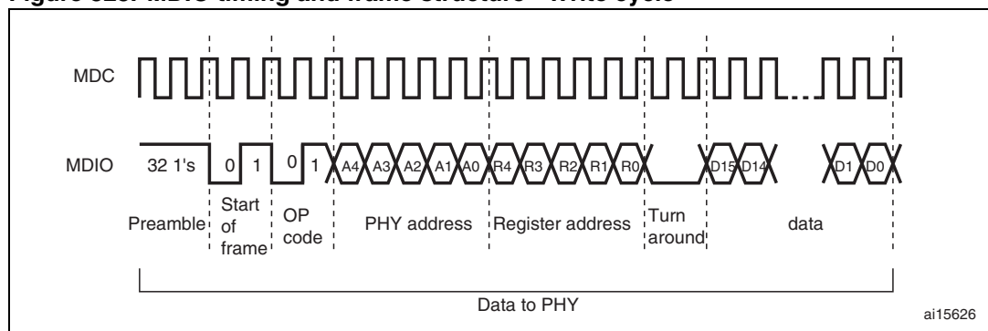
Figure 323. MDIO timing and frame structure - Write cycle
