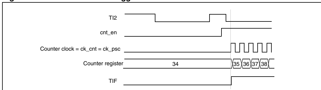
Figure 187. Control circuit in trigger mode
