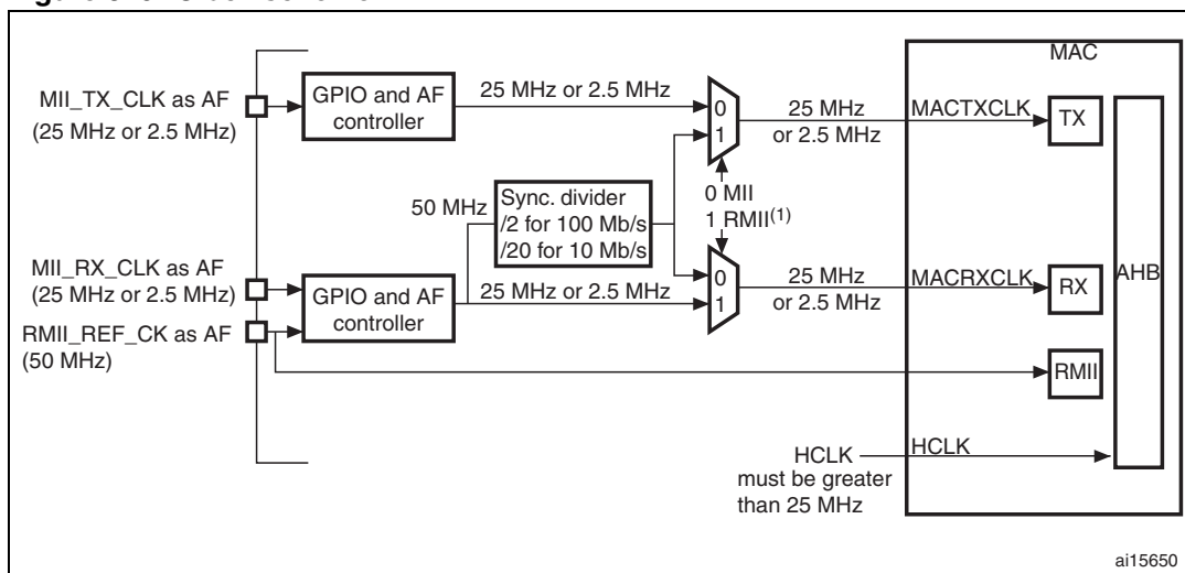
Figure 329. Clock scheme
