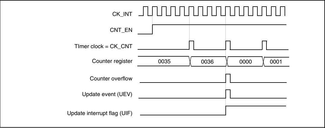
Figure 193. Counter timing diagram, internal clock divided by 4
