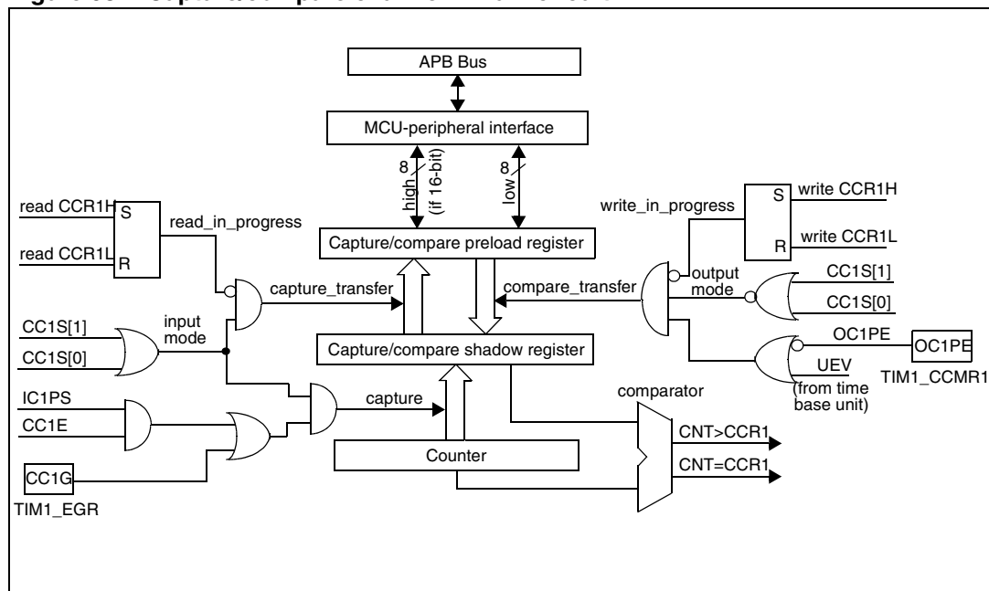
Figure 98. Capture/compare channel 1 main circuit
