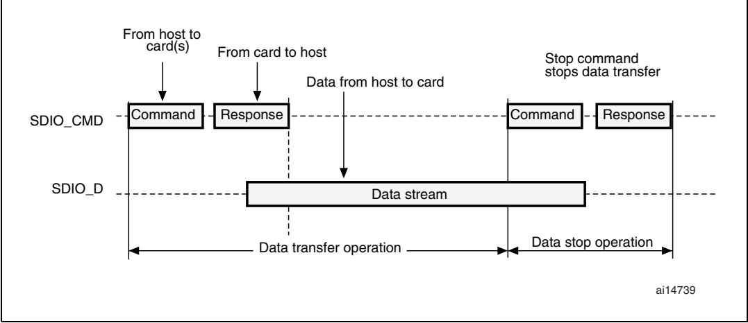
Figure 312. SDIO sequential write operation
