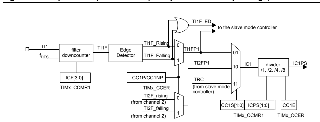
Figure 178. Capture/compare channel (example: channel 1 input stage)
