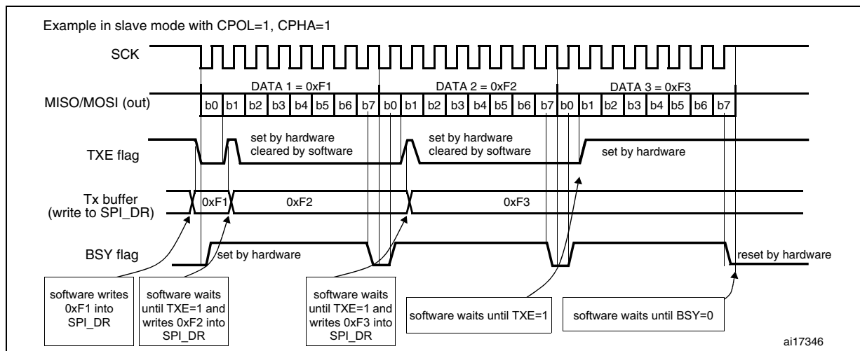
Figure 281. TXE/BSY in Slave transmit-only mode (BIDIMODE=0 and RXONLY=0) in the case of continuous transfers
