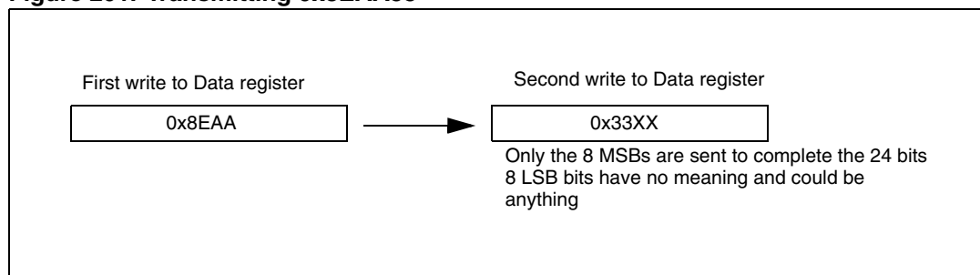
Figure 291. Transmitting 0x8EAA33
