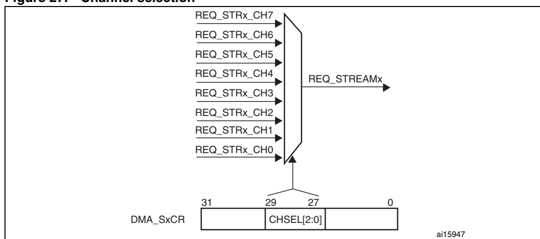
Figure 27. Channel selection
