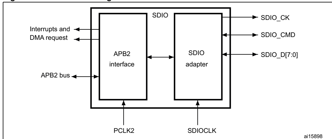
Figure 313. SDIO block diagram
