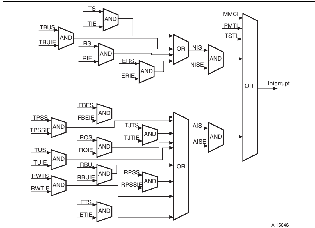
Figure 355. Interrupt scheme
