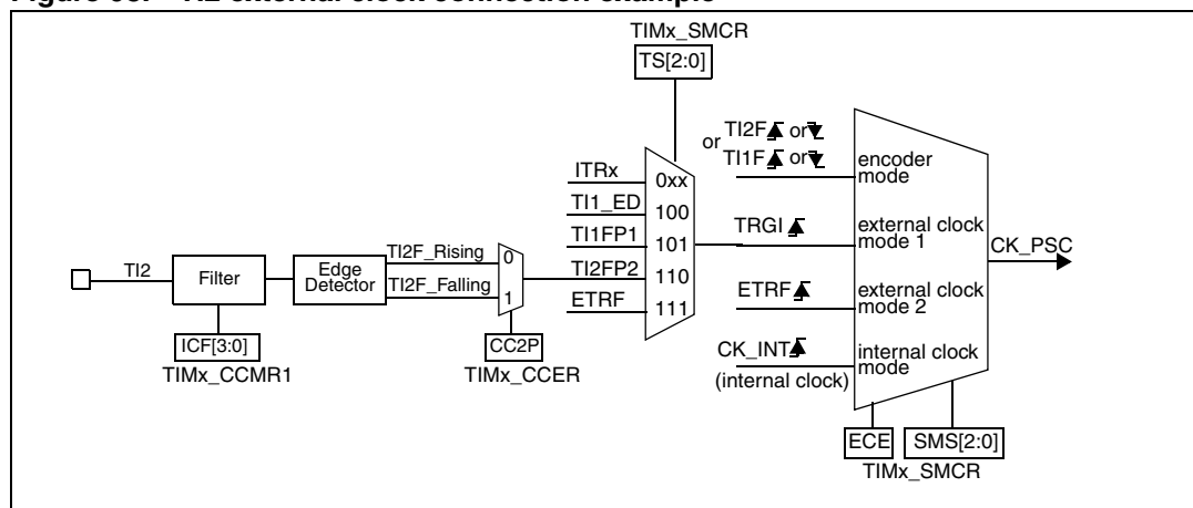
Figure 93. TI2 external clock connection example
