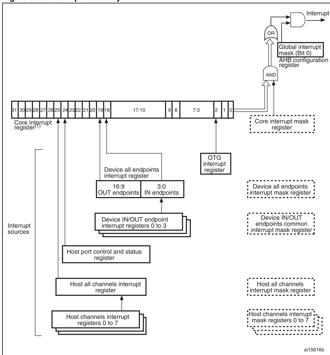
Figure 365. Interrupt hierarchy
