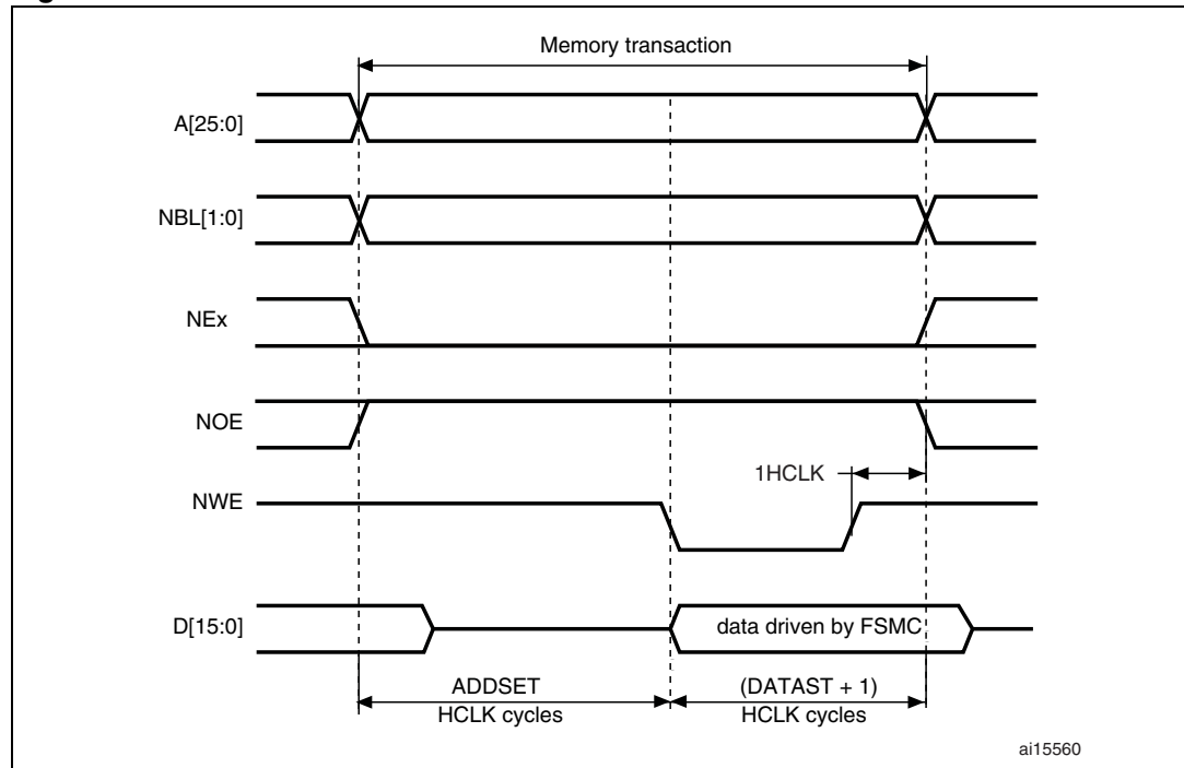
Figure 408. ModeA write accesses
