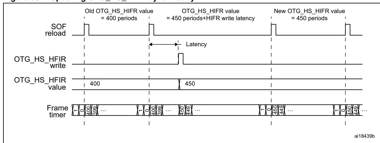
Figure 382. Updating OTG_HS_HFIR dynamically
