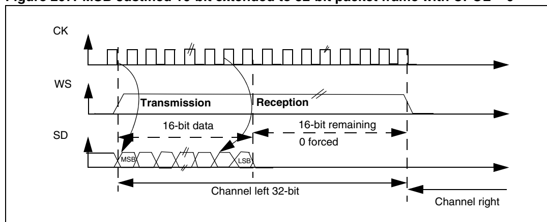
Figure 297. MSB Justified 16-bit extended to 32-bit packet frame with CPOL = 0
