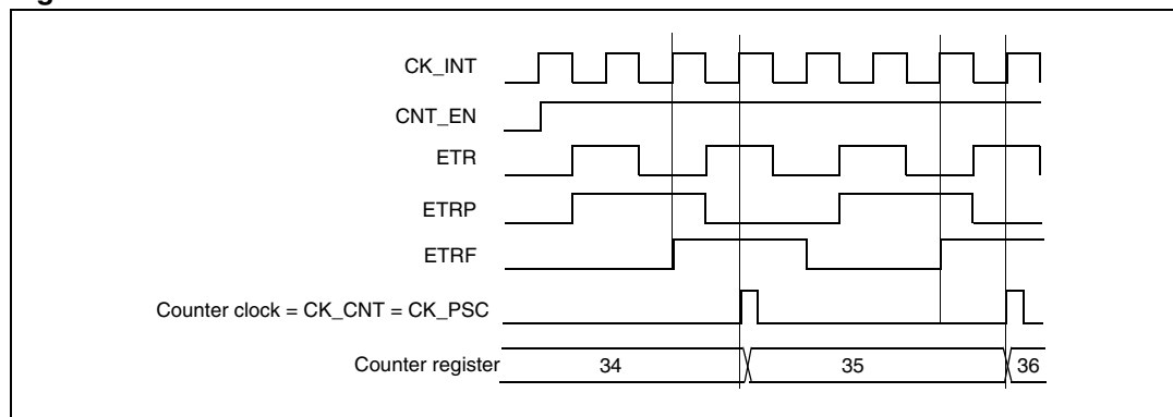
Figure 143. Control circuit in external clock mode 2
