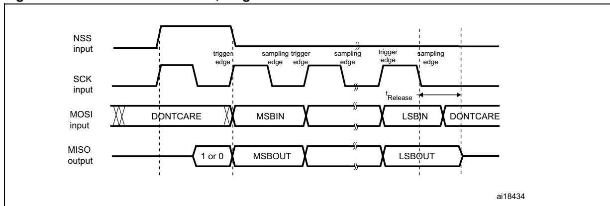
Figure 274. TI mode - Slave mode, single transfer
