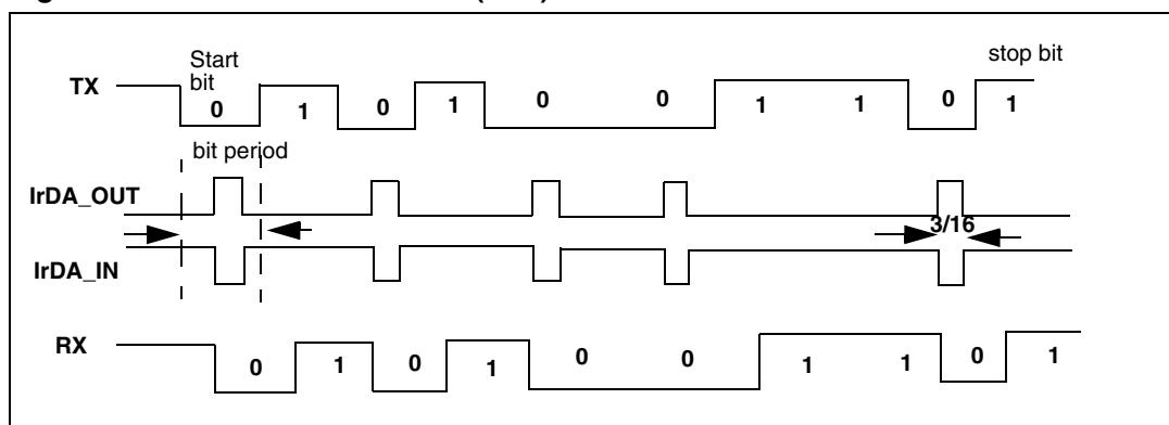
Figure 264. IrDA data modulation (3/16) -Normal mode
