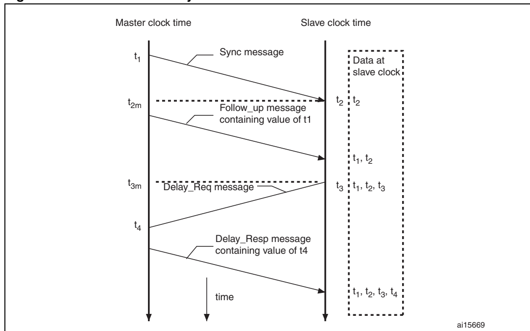
Figure 343. Networked time synchronization
