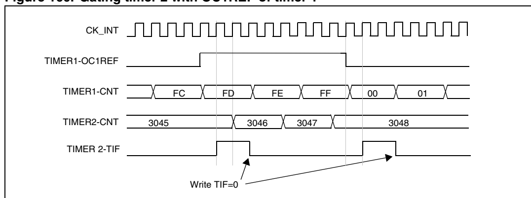
Figure 160. Gating timer 2 with OC1REF of timer 1
