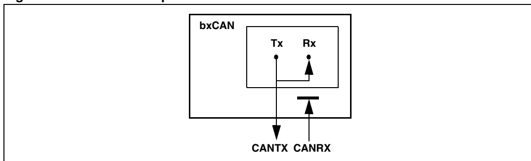
Figure 227. bxCAN in loop back mode
