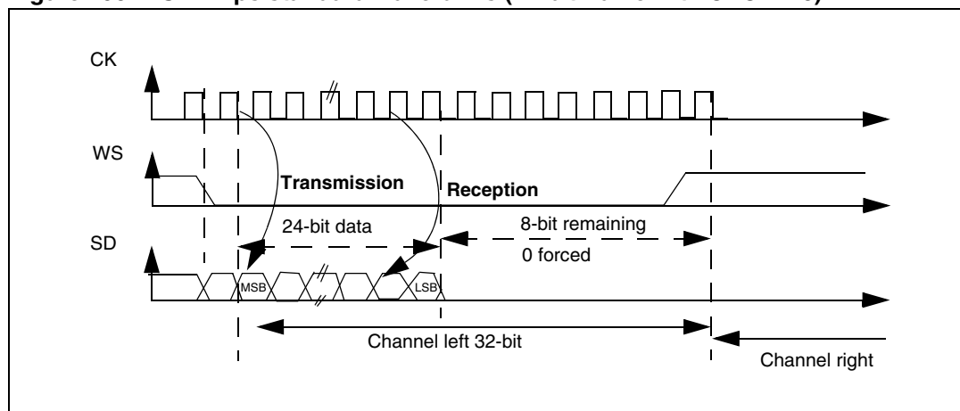
Figure 290. I 2 S Philips standard waveforms (24-bit frame with CPOL = 0)
