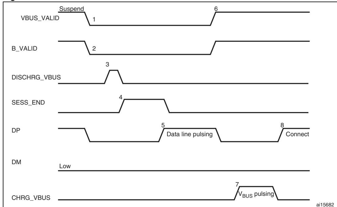
Figure 378. B-device SRP
