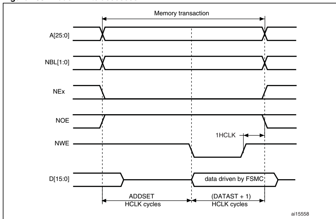
Figure 406. Mode1 write accesses
