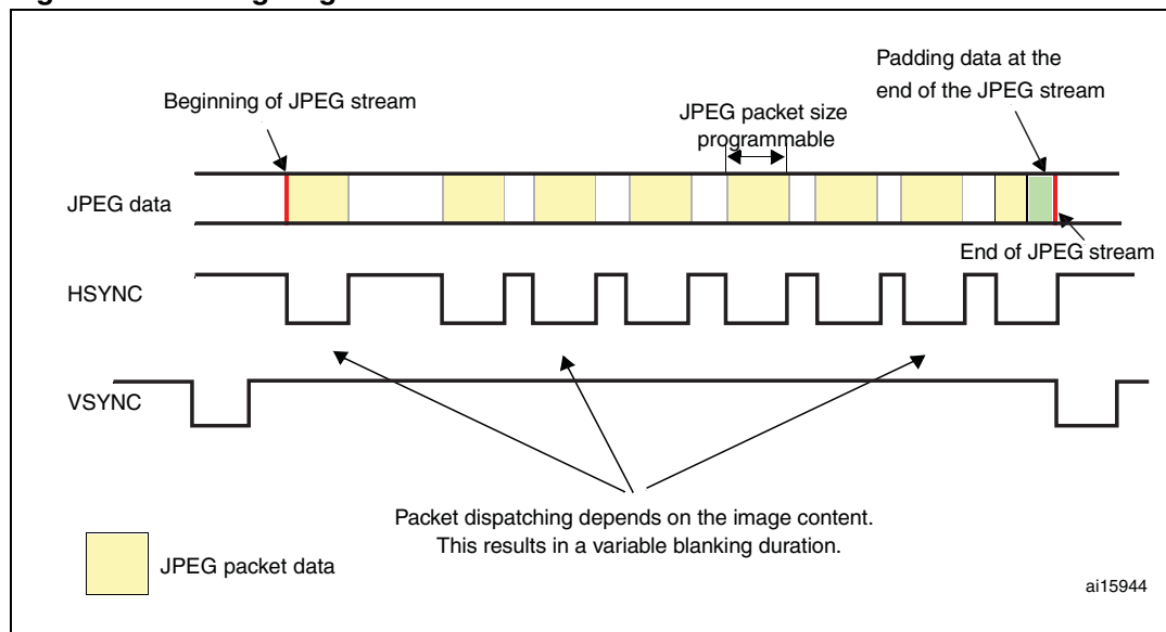
Figure 65. Timing diagram
