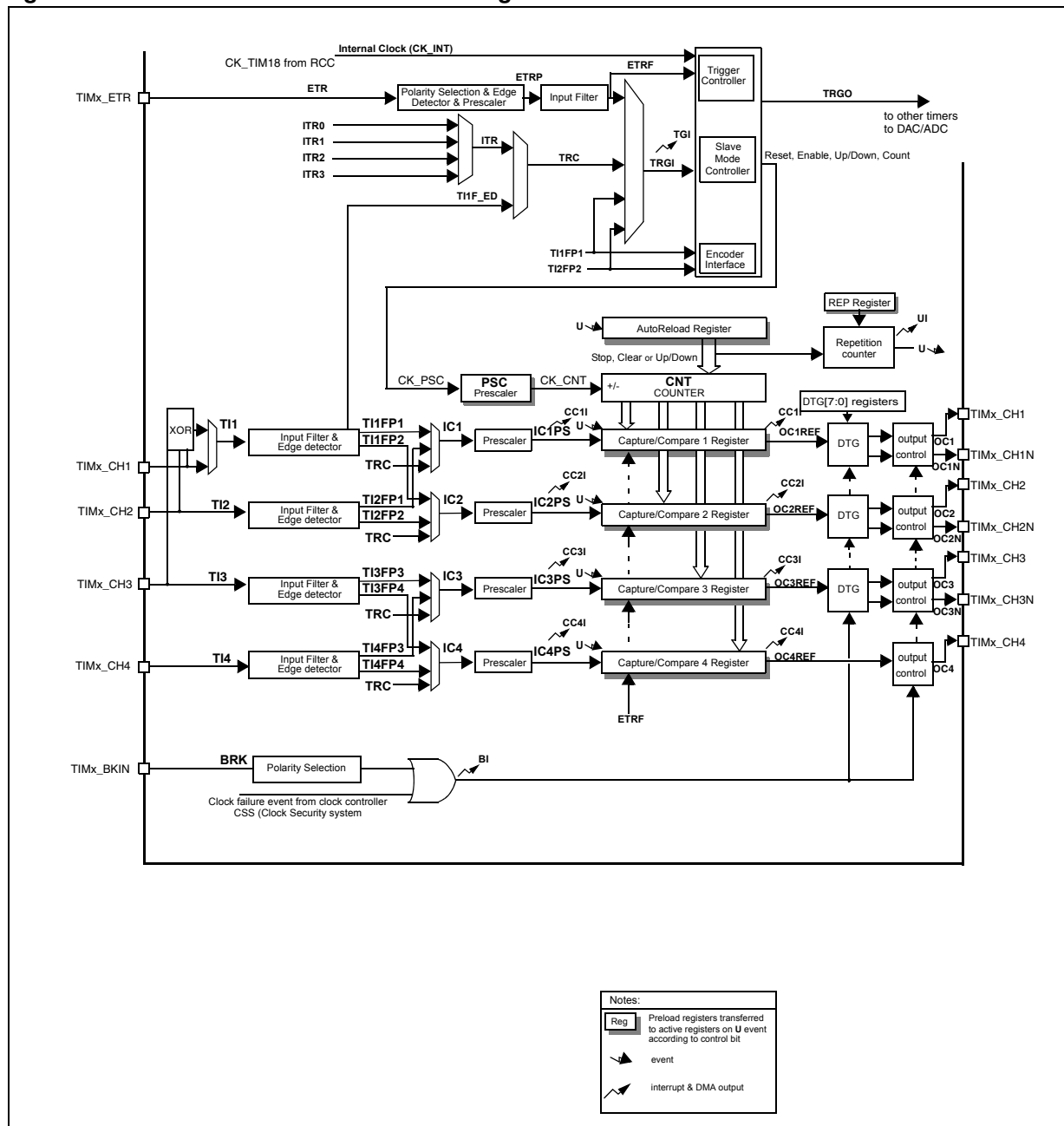
Figure 71. Advanced-control timer block diagram
