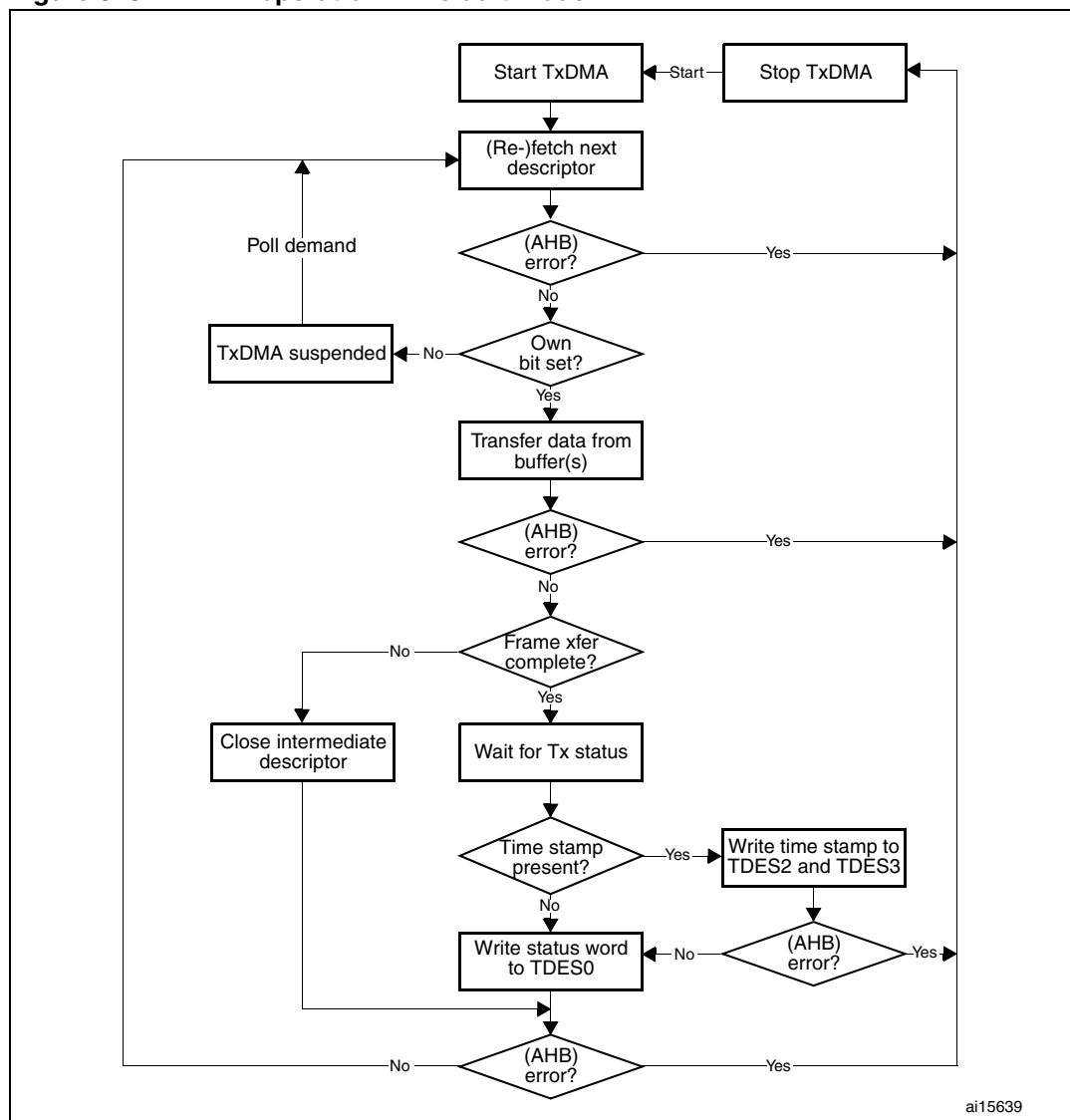
Figure 348. TxDMA operation in Default mode
