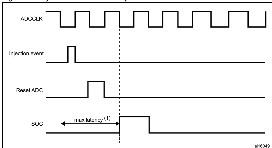
Figure 37. Injected conversion latency
