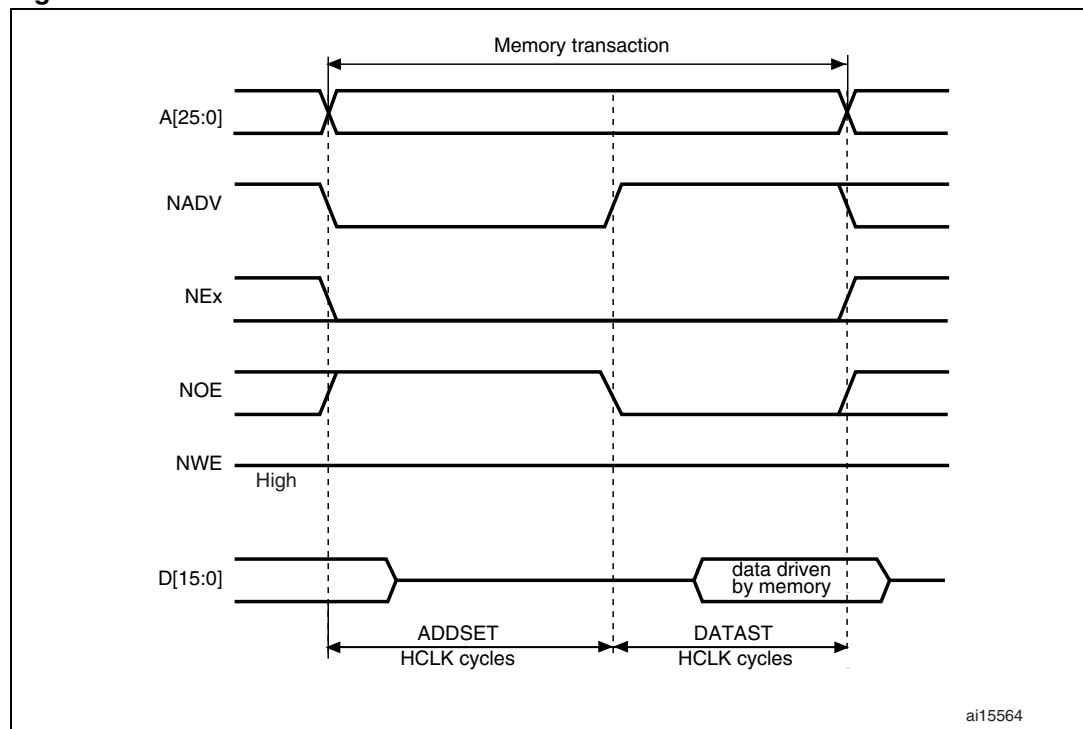
Figure 412. Mode C read accesses
