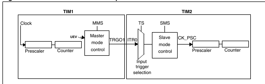
Figure 159. Master/Slave timer example
