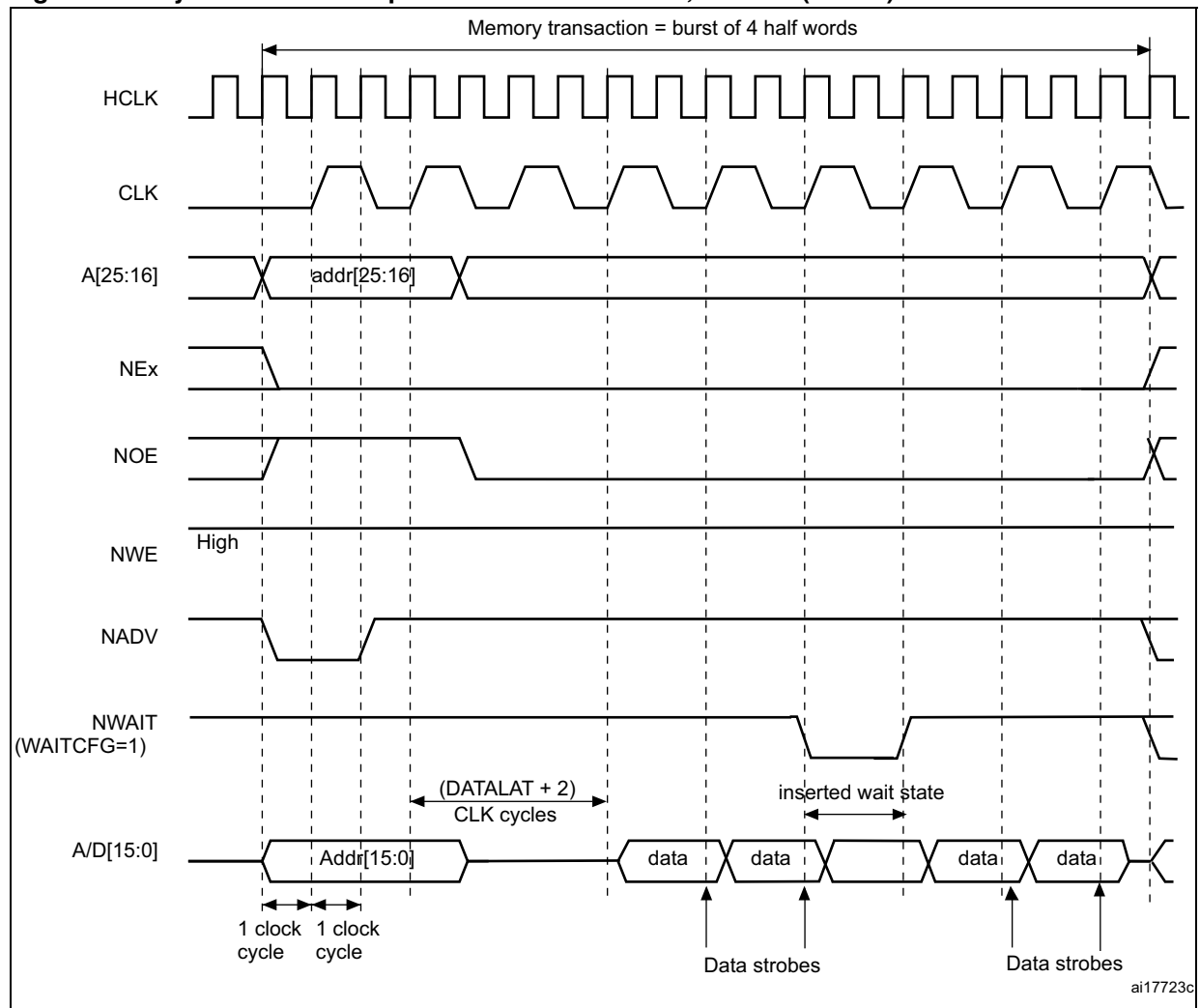
Figure 421. Synchronous multiplexed read mode - NOR, PSRAM (CRAM)
