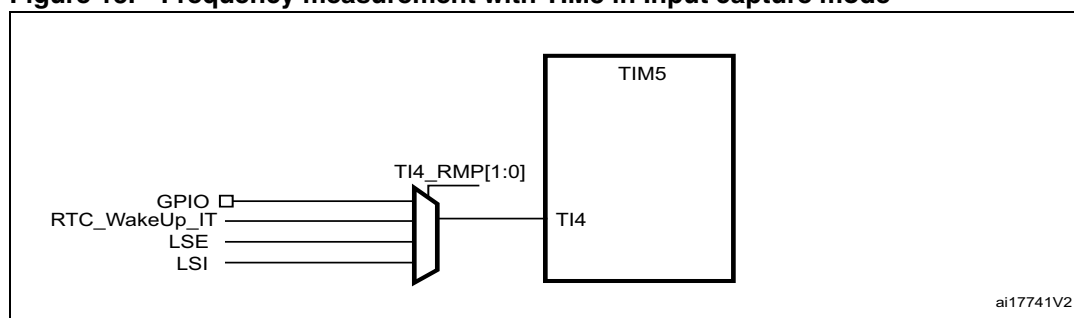
Figure 15. Frequency measurement with TIM5 in Input capture mode
