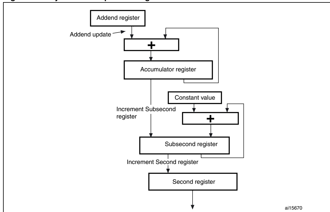
Figure 344. System time update using the Fine correction method
