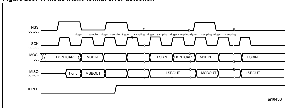
Figure 286. TI mode frame format error detection
