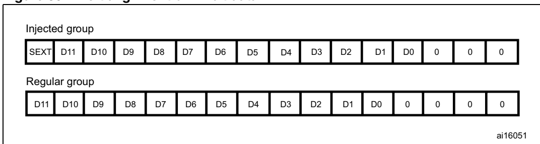
Figure 39. Left alignment of 12-bit data
