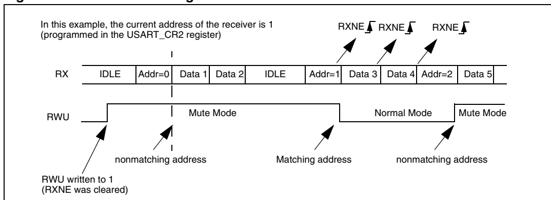
Figure 254. Mute mode using address mark detection
