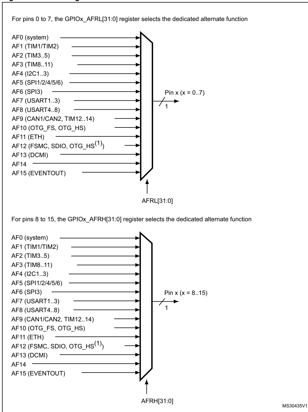
Figure 19. Selecting an alternate function on STM32F42xxx and STM32F43xxx
