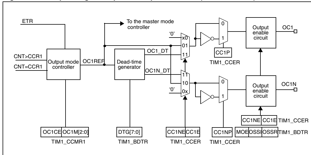
Figure 99. Output stage of capture/compare channel (channel 1 to 3)
