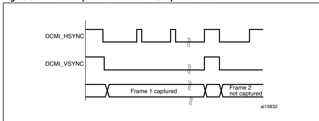
Figure 66. Frame capture waveforms in Snapshot mode
