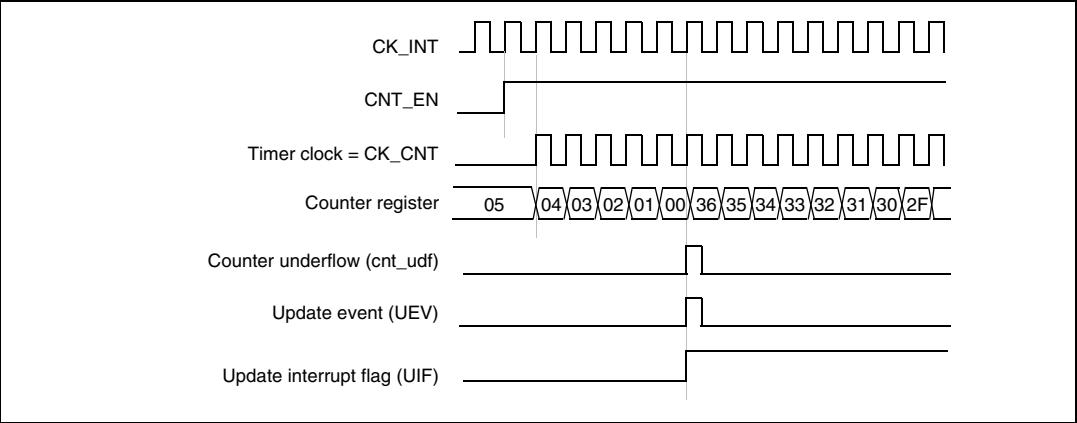
Figure 128. Counter timing diagram, internal clock divided by 1
