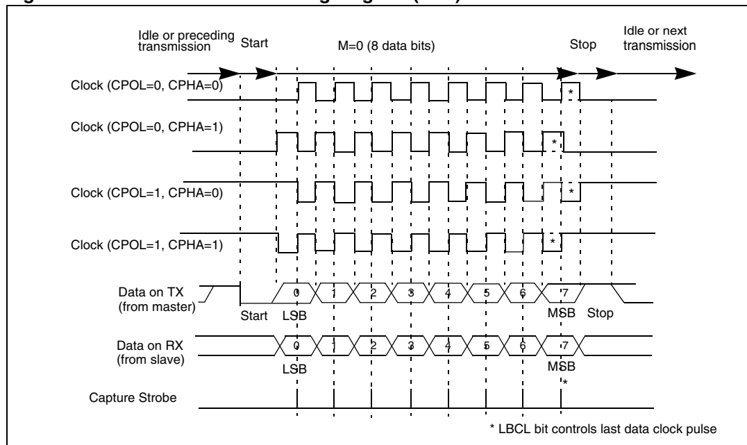
Figure 258. USART data clock timing diagram (M=0)
