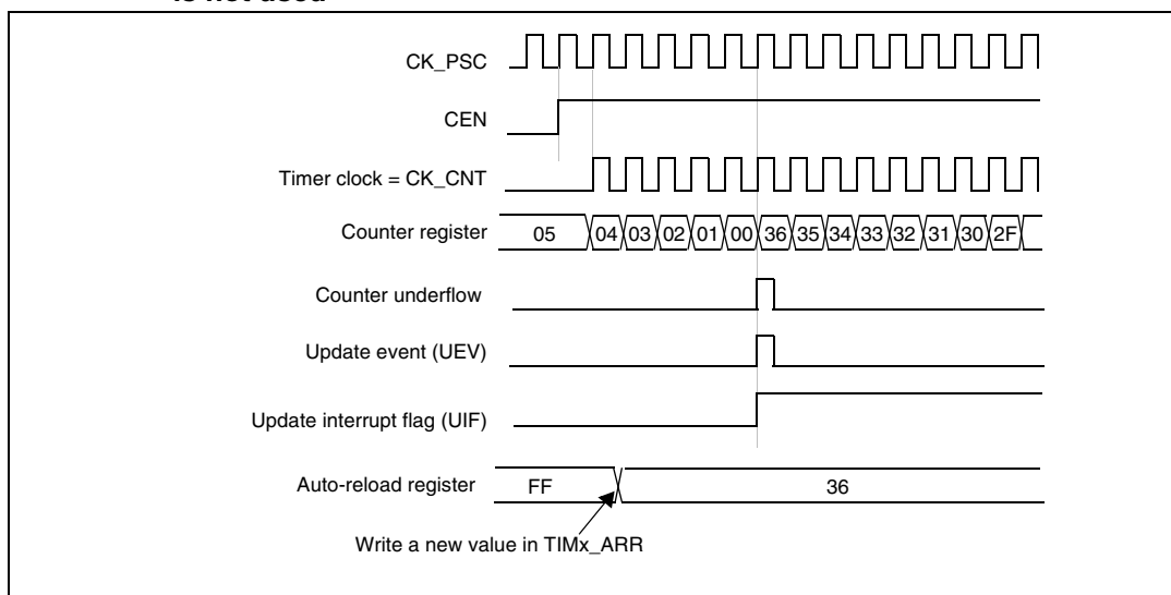
Figure 84. Counter timing diagram, update event when repetition counter is not used
