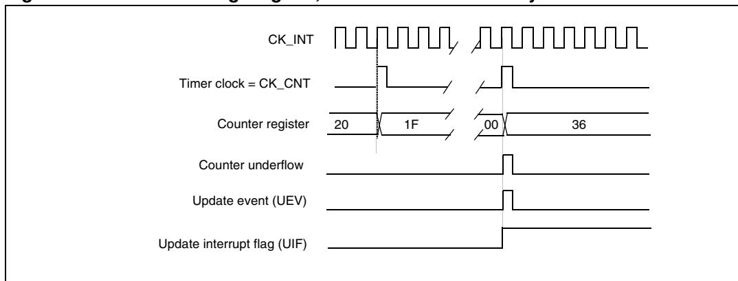
Figure 131. Counter timing diagram, internal clock divided by N
