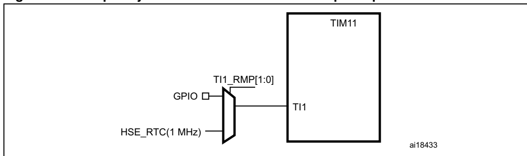
Figure 16. Frequency measurement with TIM11 in Input capture mode
