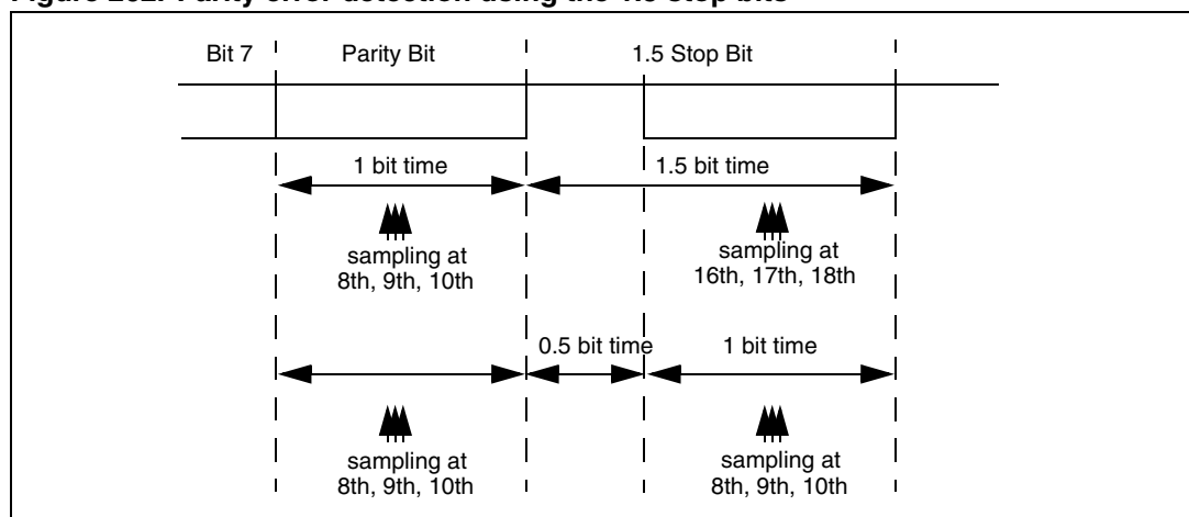
Figure 262. Parity error detection using the 1.5 stop bits
