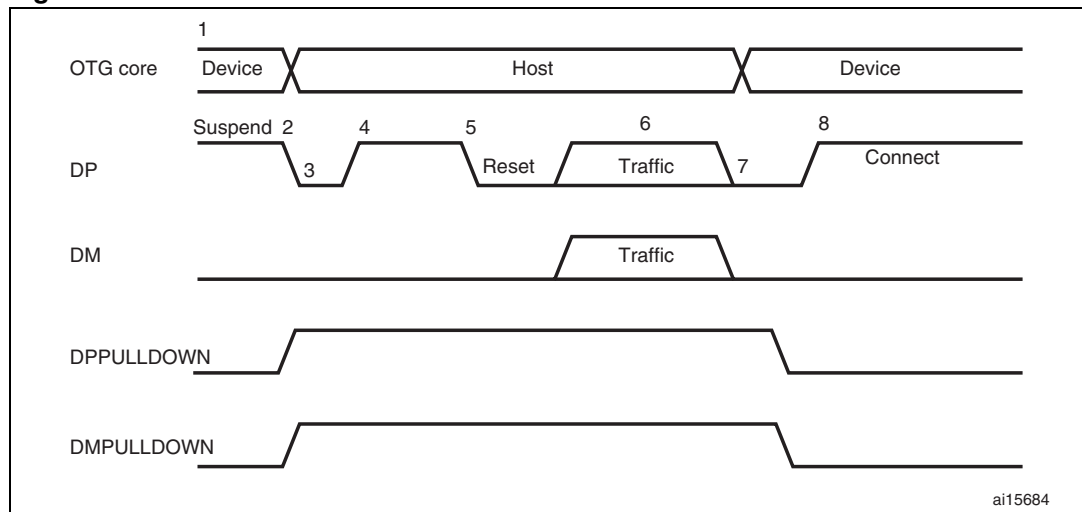
Figure 380. B-device HNP
