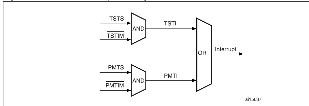
Figure 341. MAC core interrupt masking scheme
