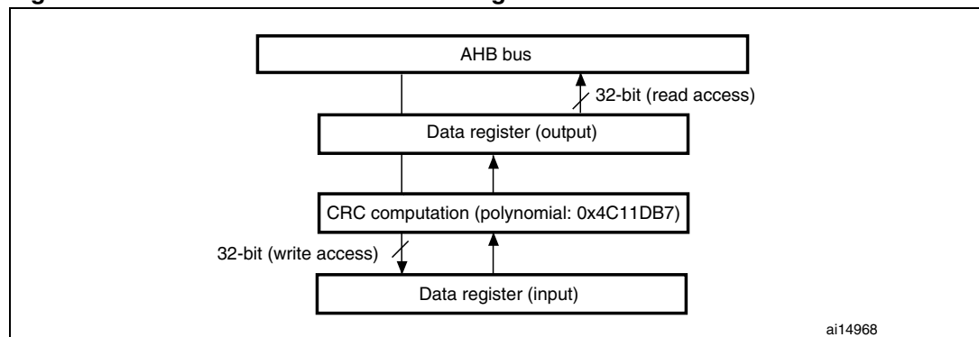
Figure 6. CRC calculation unit block diagram
