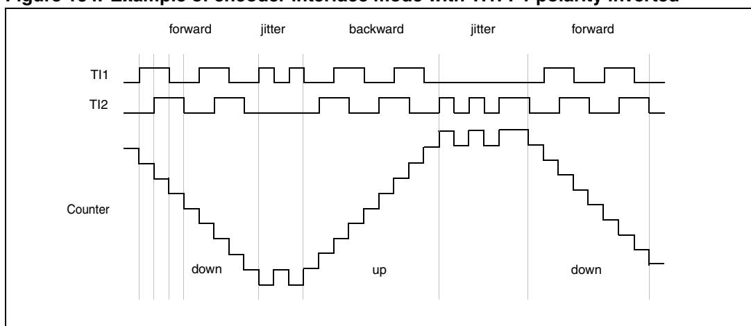
Figure 154. Example of encoder interface mode with TI1FP1 polarity inverted
