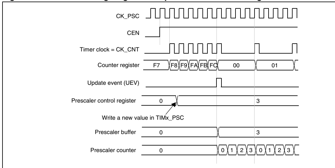
Figure 168. Counter timing diagram with prescaler division change from 1 to 4
