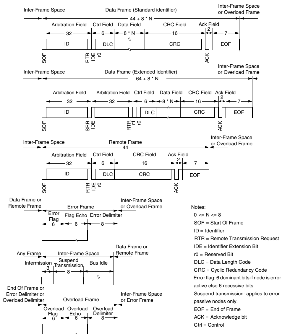
Figure 236. CAN frames
