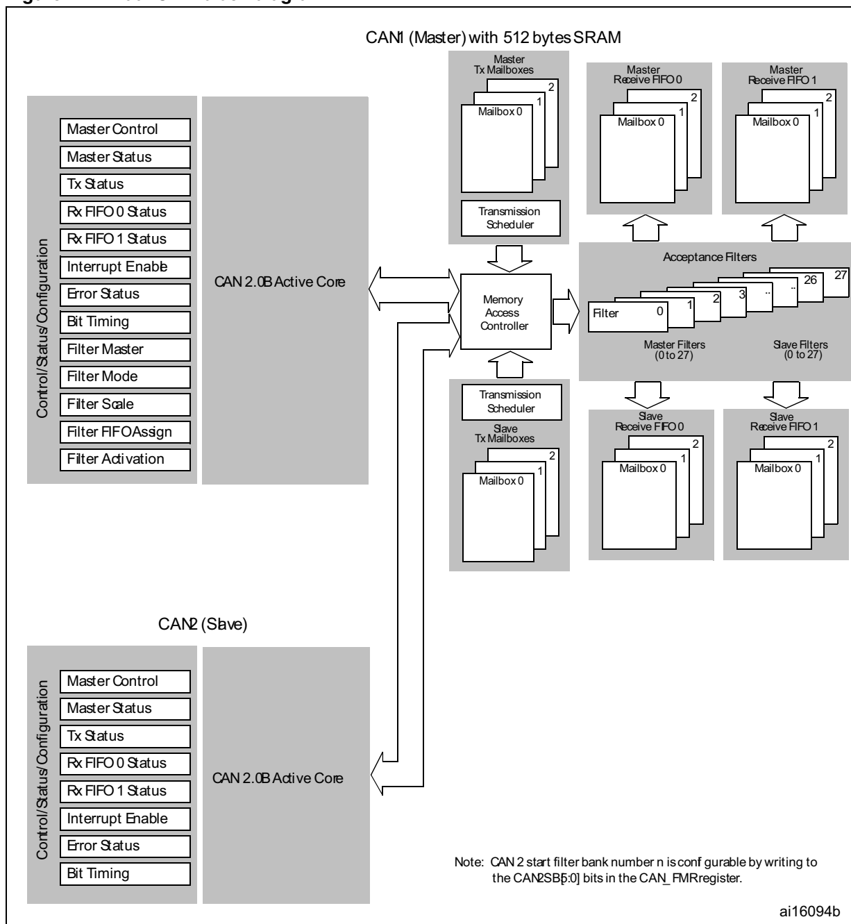
Figure 224. Dual CAN block diagram
