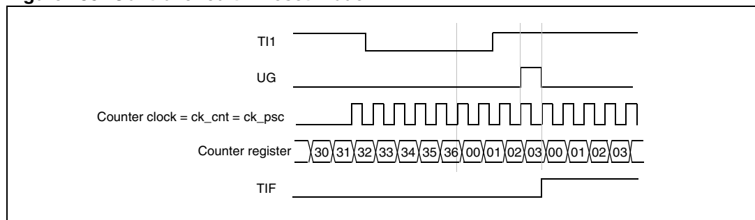
Figure 185. Control circuit in reset mode
