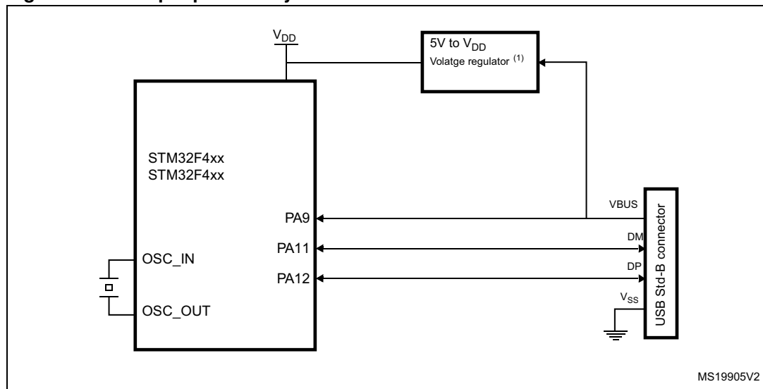
Figure 359. USB peripheral-only connection
