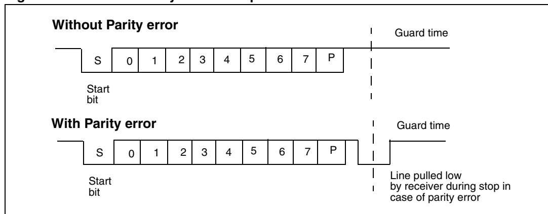
Figure 261. ISO 7816-3 asynchronous protocol
