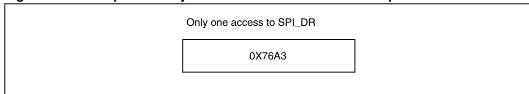
Figure 303. Example of LSB justified 16-bit extended to 32-bit packet frame
