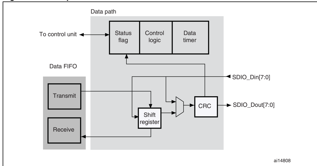
Figure 319. Data path
