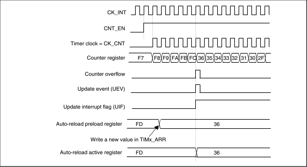
Figure 138. Counter timing diagram, Update event with ARPE=1 (counter overflow)
