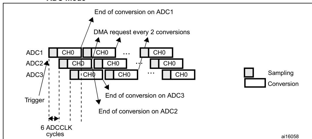
Figure 47. Interleaved mode on 1 channel in continuous conversion mode: triple ADC mode
