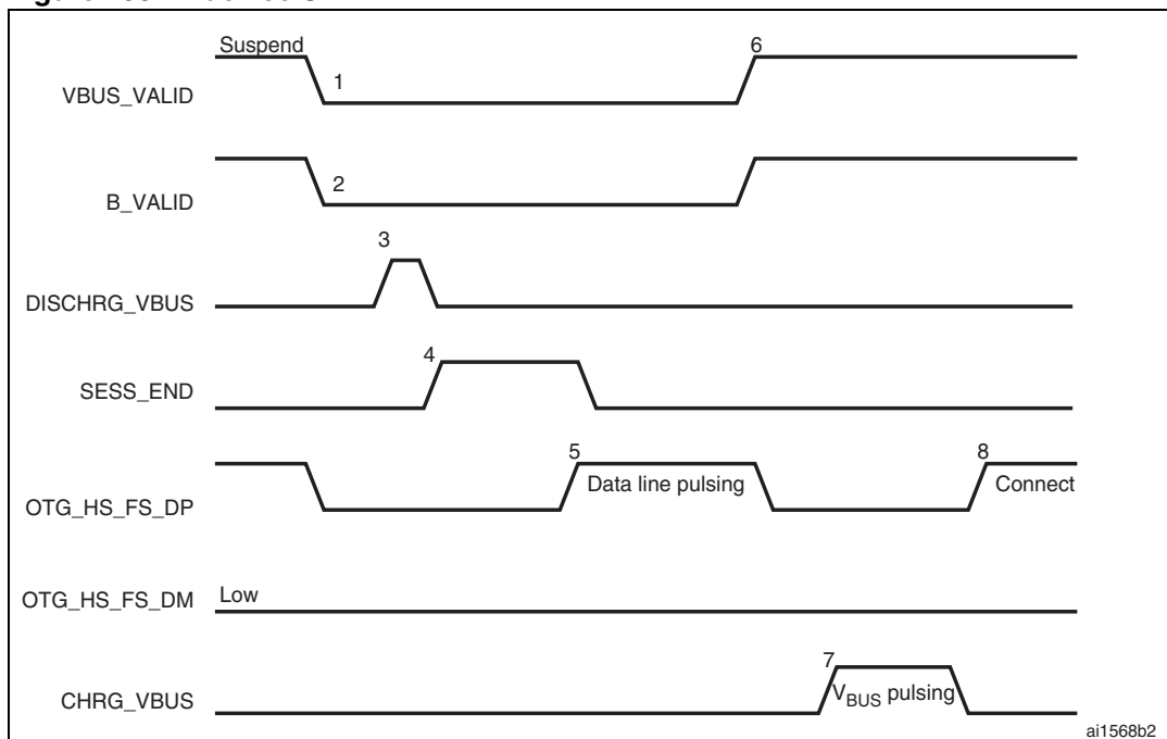
Figure 400. B-device SRP
