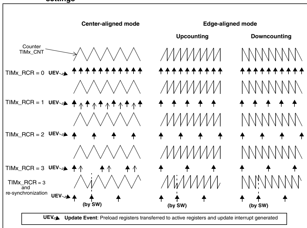
Figure 91. Update rate examples depending on mode and TIMx_RCR register settings
