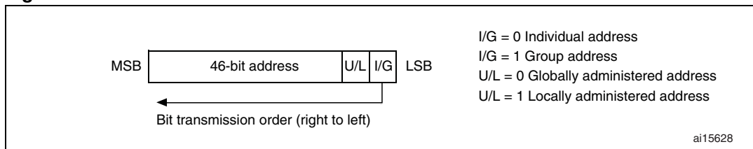
Figure 330. Address field format
