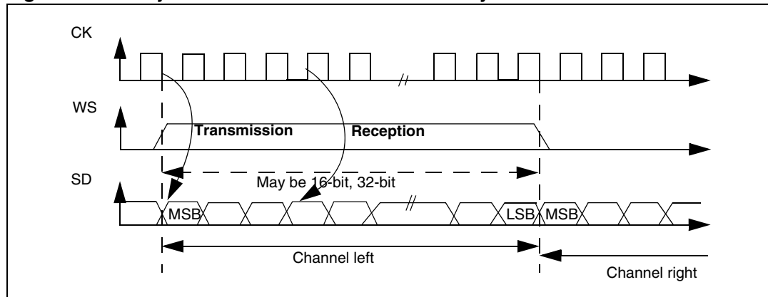
Figure 298. LSB justified 16-bit or 32-bit full-accuracy with CPOL = 0
