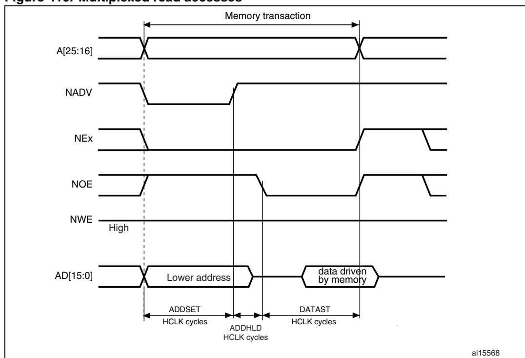
Figure 416. Multiplexed read accesses
