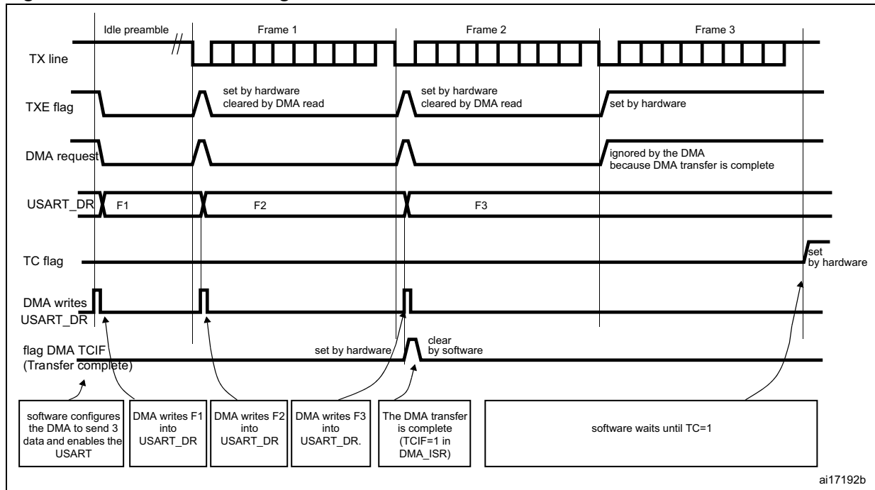
Figure 265. Transmission using DMA
