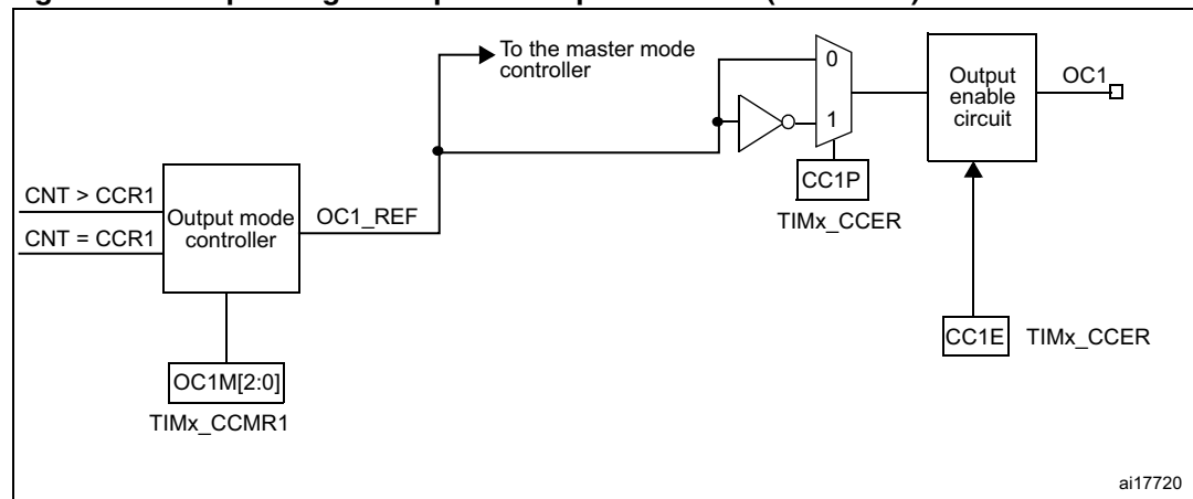
Figure 180. Output stage of capture/compare channel (channel 1)
