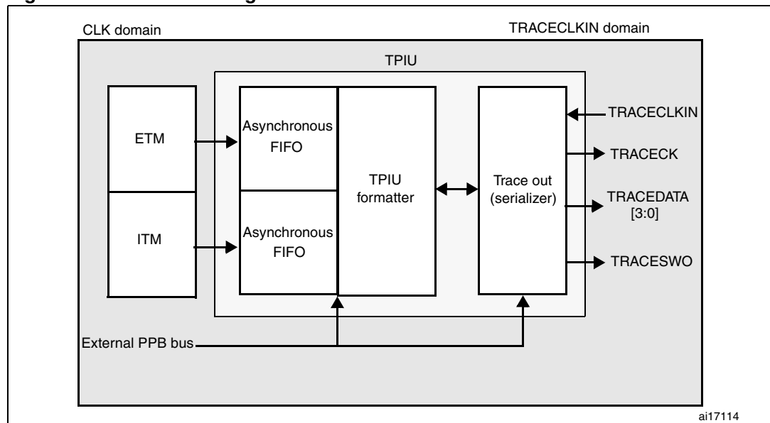
Figure 428. TPIU block diagram
