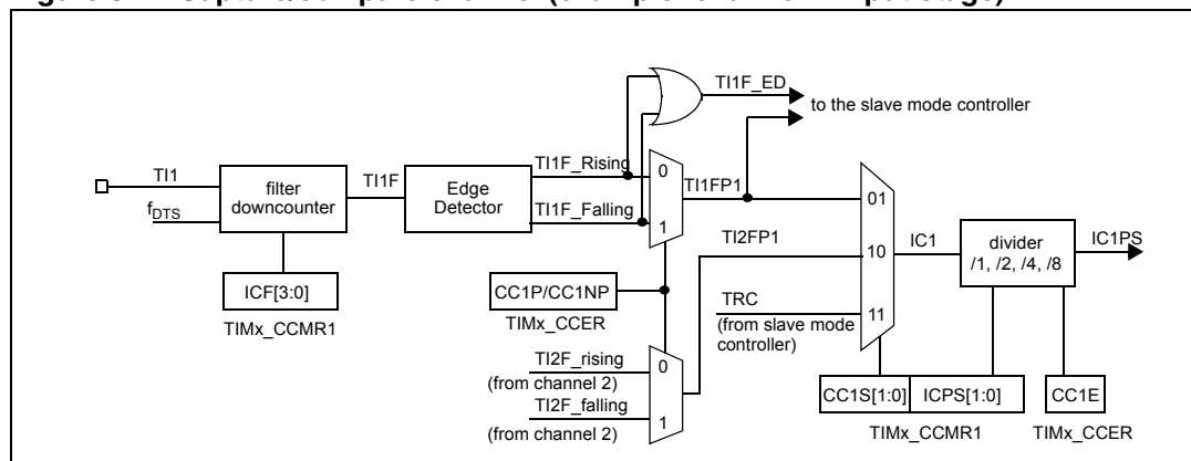
Figure 97. Capture/compare channel (example: channel 1 input stage)
