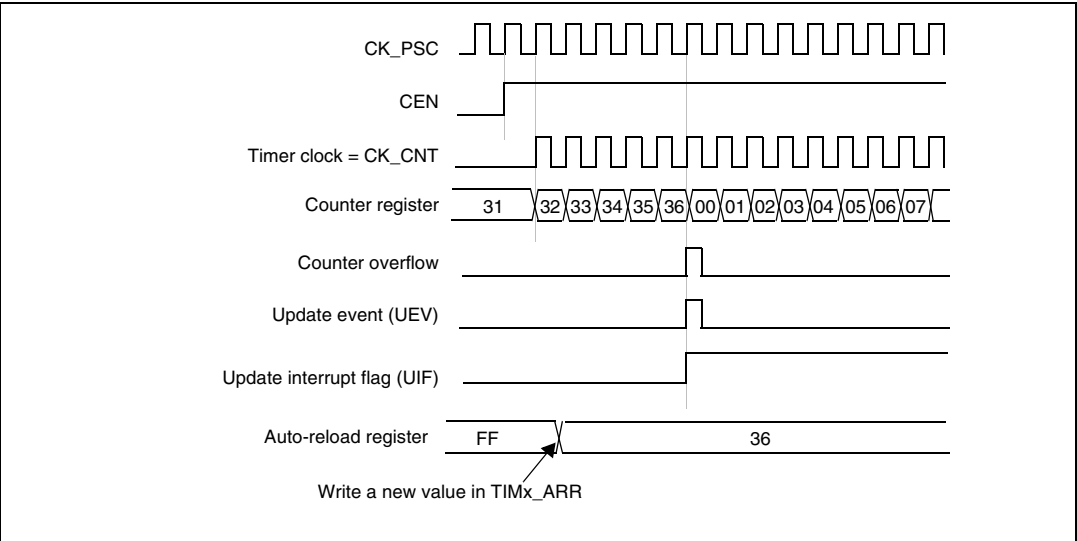
Figure 173. Counter timing diagram, update event when ARPE=0 (TIMx_ARR not preloaded)
