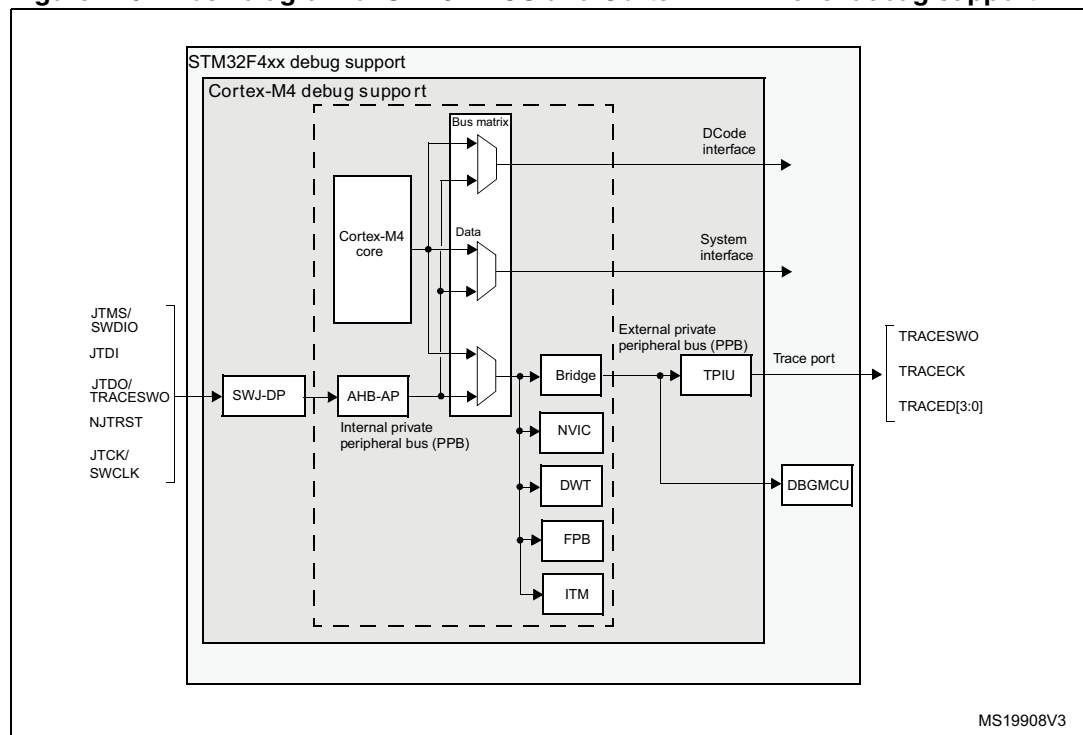
Figure 425. Block diagram of STM32 MCU and Cortex™-M4F-level debug support
