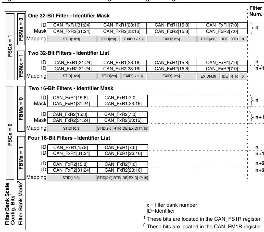
Figure 231. Filter bank scale configuration - register organization
