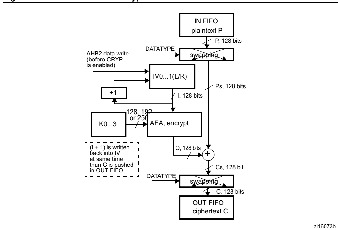
Figure 211. AES-CTR mode encryption
