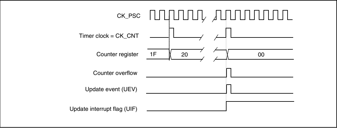
Figure 78. Counter timing diagram, update event when ARPE=0 (TIMx_ARR not preloaded)
