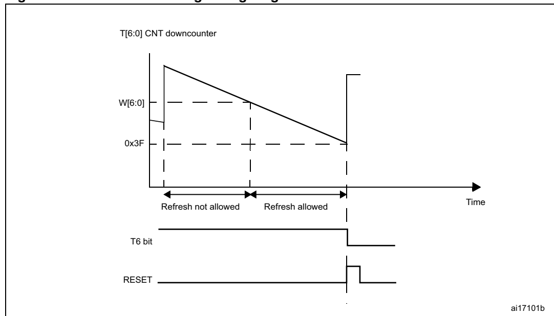
Figure 200. Window watchdog timing diagram
