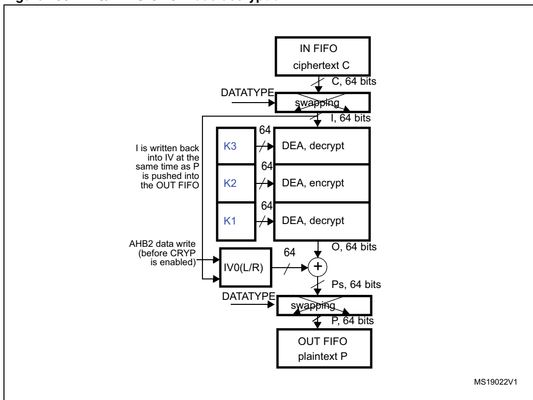
Figure 206. DES/TDES-CBC mode decryption
