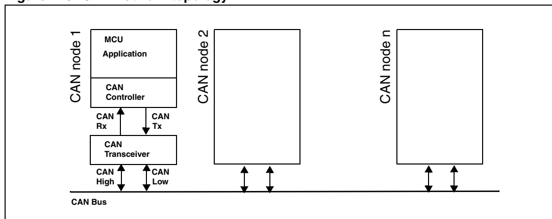
Figure 223. CAN network topology
