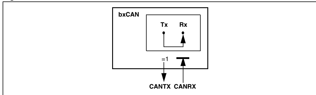
Figure 228. bxCAN in combined mode
