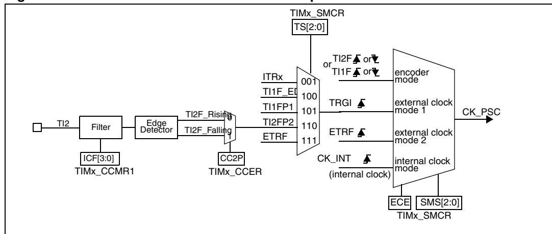
Figure 140. TI2 external clock connection example
