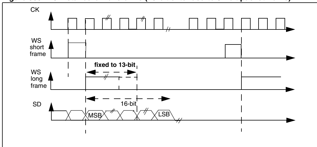
Figure 305. PCM standard waveforms (16-bit extended to 32-bit packet frame)
