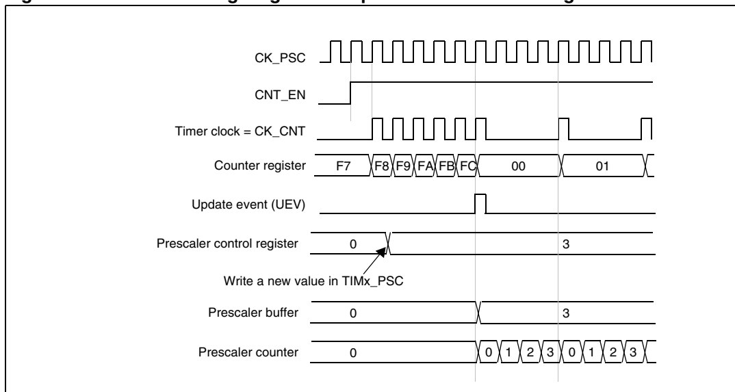
Figure 190. Counter timing diagram with prescaler division change from 1 to 4
