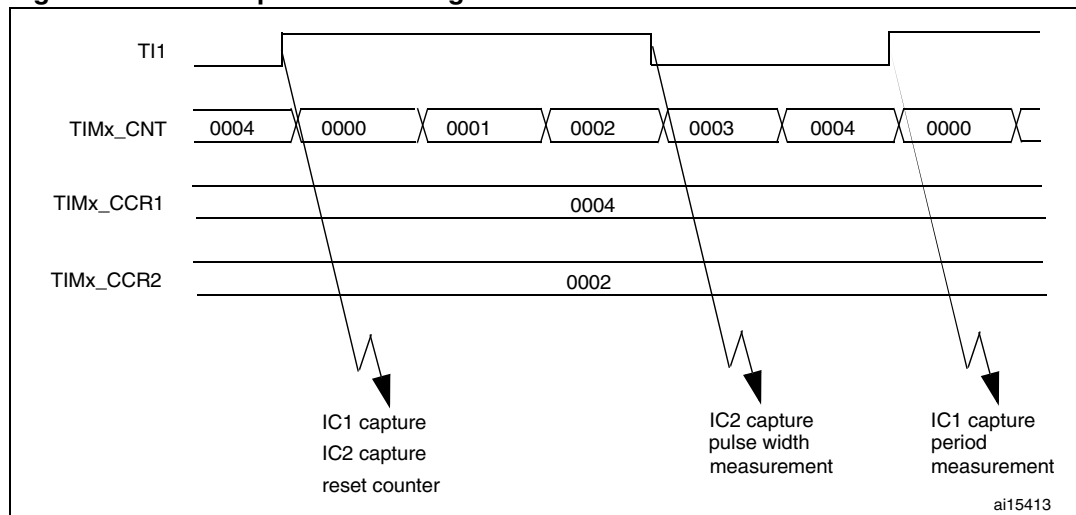
Figure 101. PWM input mode timing
