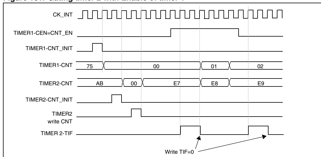
Figure 161. Gating timer 2 with Enable of timer 1
