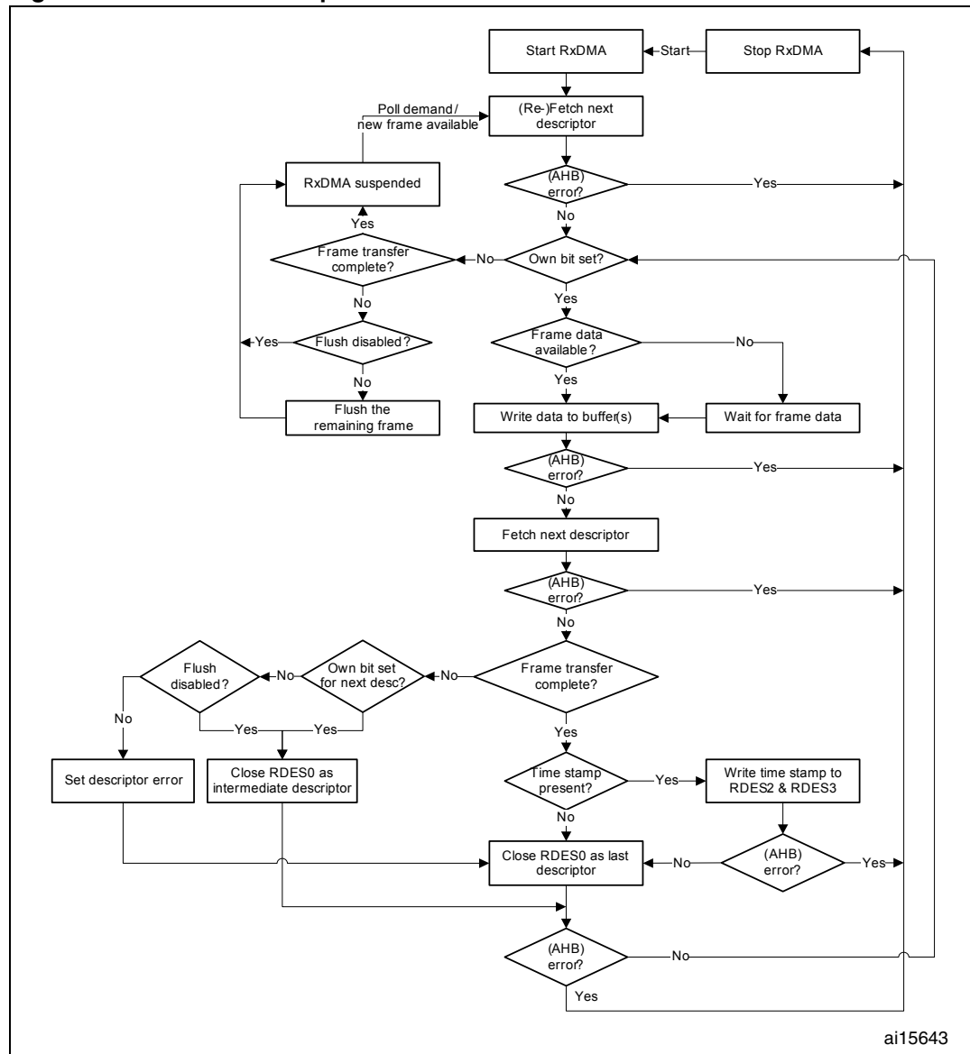
Figure 352. Receive DMA operation
