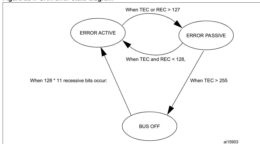
Figure 234. CAN error state diagram
