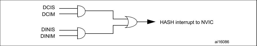
Figure 221. HASH interrupt mapping diagram
