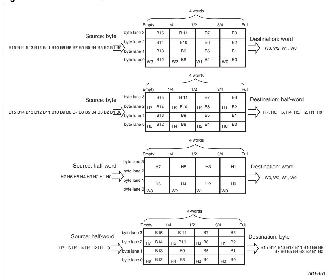
Figure 31. FIFO structure
