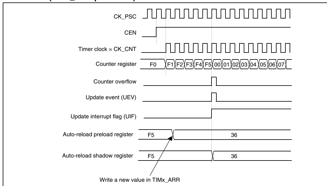
Figure 79. Counter timing diagram, update event when ARPE=1 (TIMx_ARR preloaded)
