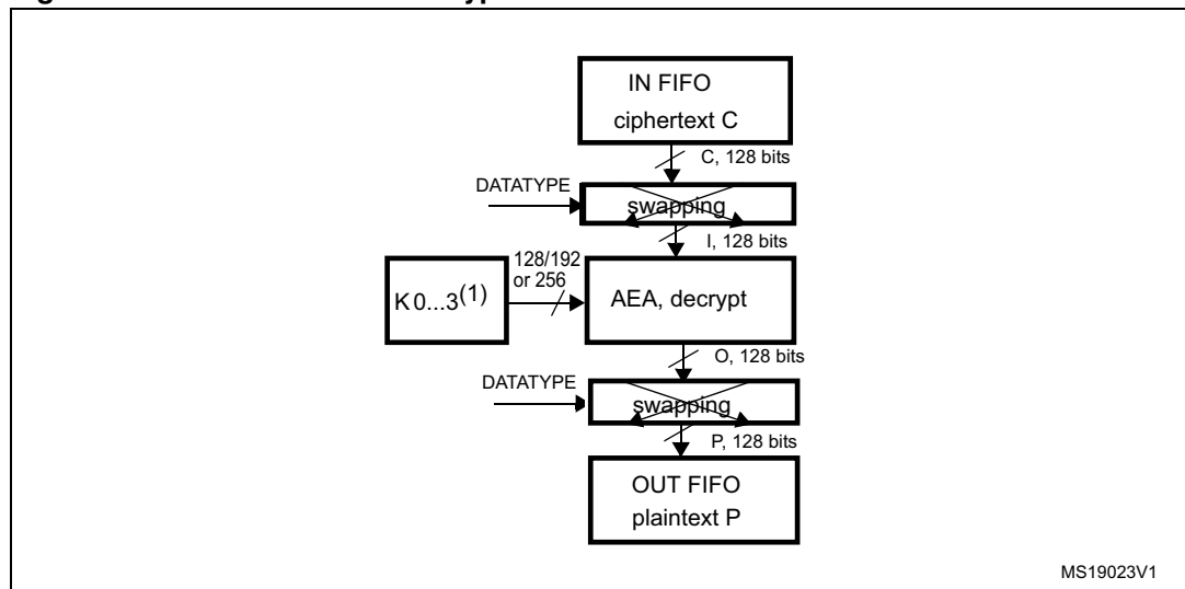
Figure 208. AES-ECB mode decryption
