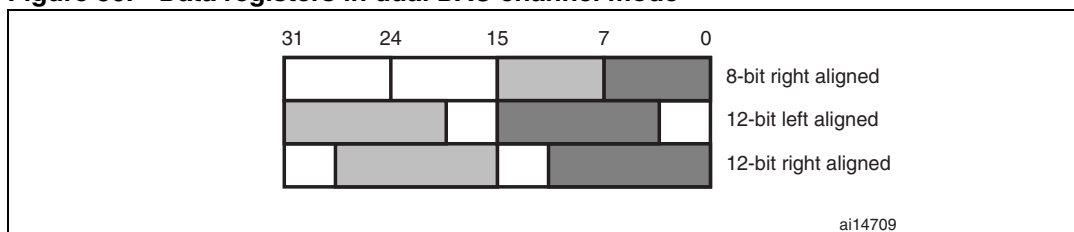
Figure 56. Data registers in dual DAC channel mode
