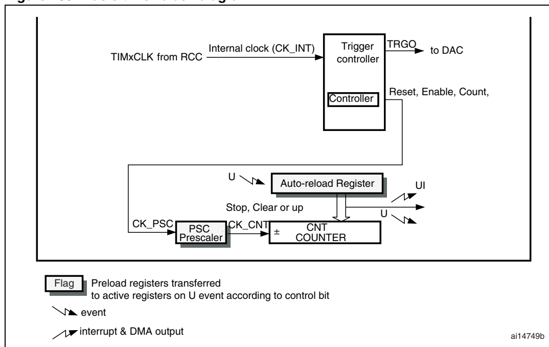
Figure 188. Basic timer block diagram
