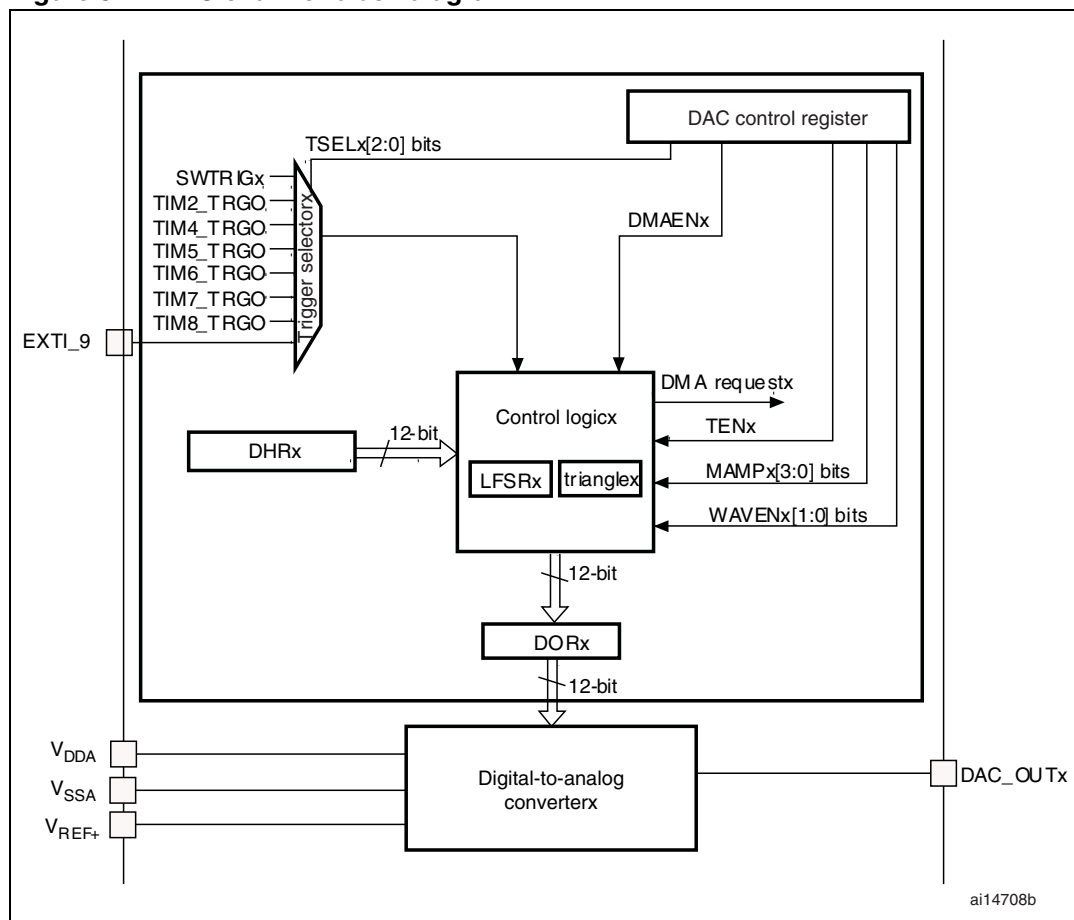
Figure 54. DAC channel block diagram
