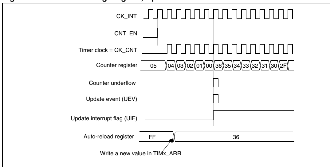
Figure 132. Counter timing diagram, Update event
