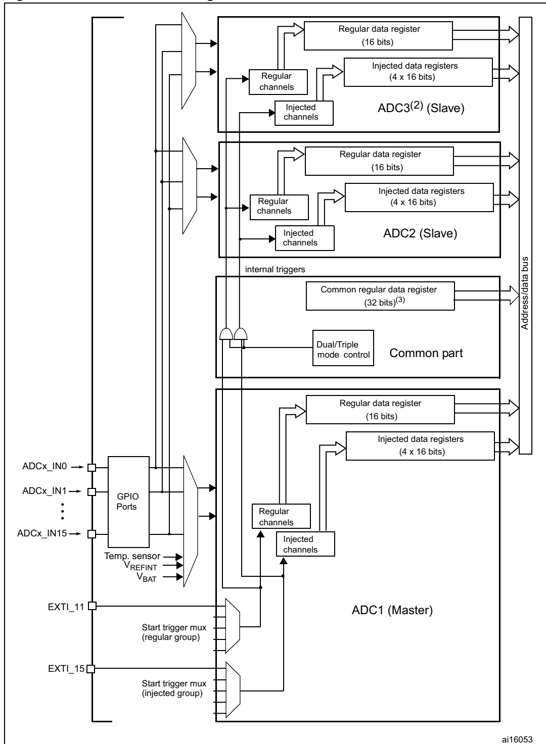
Figure 41. Multi ADC block diagram (1)
