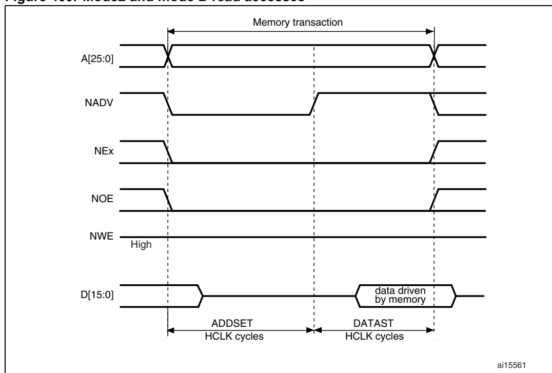
Figure 409. Mode2 and mode B read accesses
