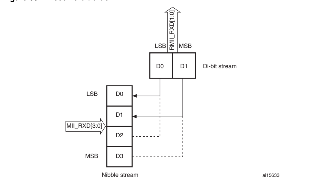
Figure 337. Receive bit order
