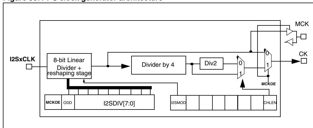
Figure 307. I 2 S clock generator architecture
