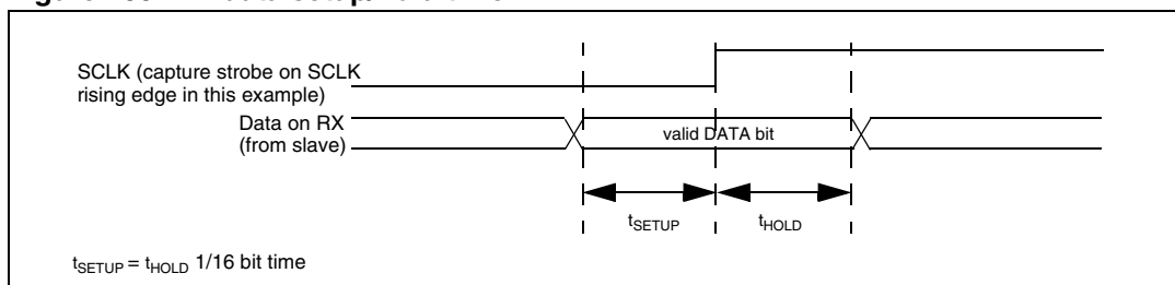
Figure 260. RX data setup/hold time
