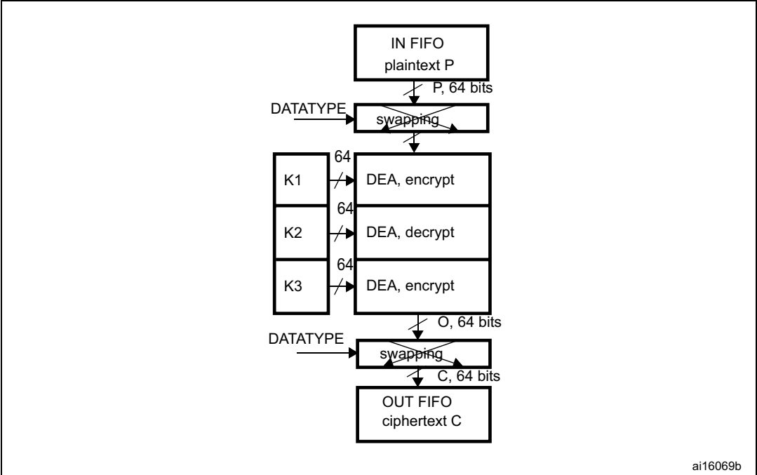
Figure 203. DES/TDES-ECB mode encryption
