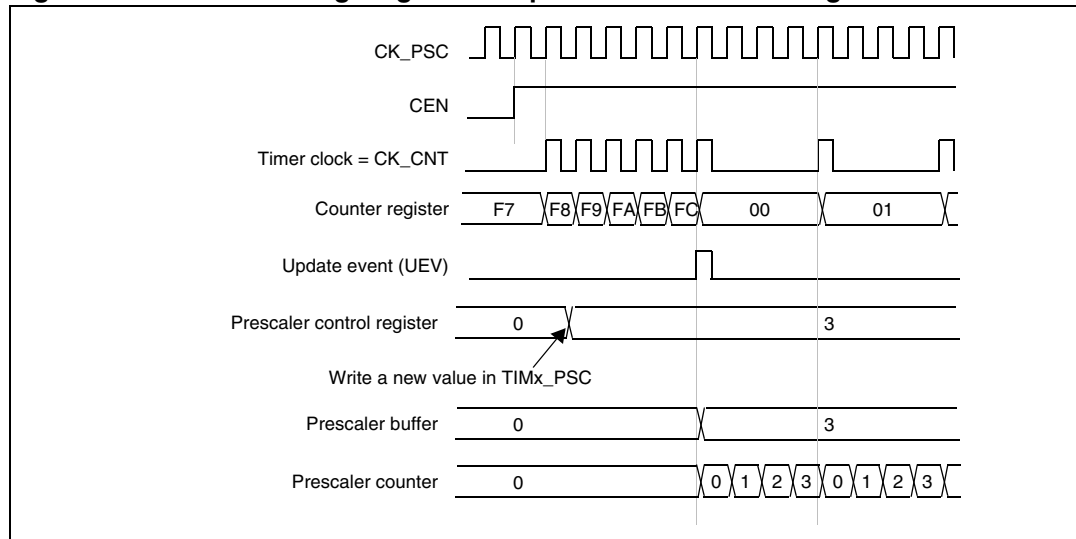
Figure 73. Counter timing diagram with prescaler division change from 1 to 4
