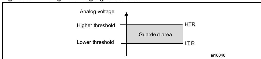
Figure 36. Analog watchdog's guarded area
