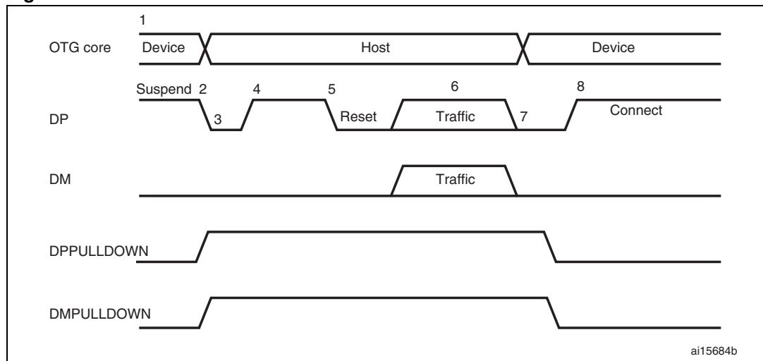
Figure 402. B-device HNP
