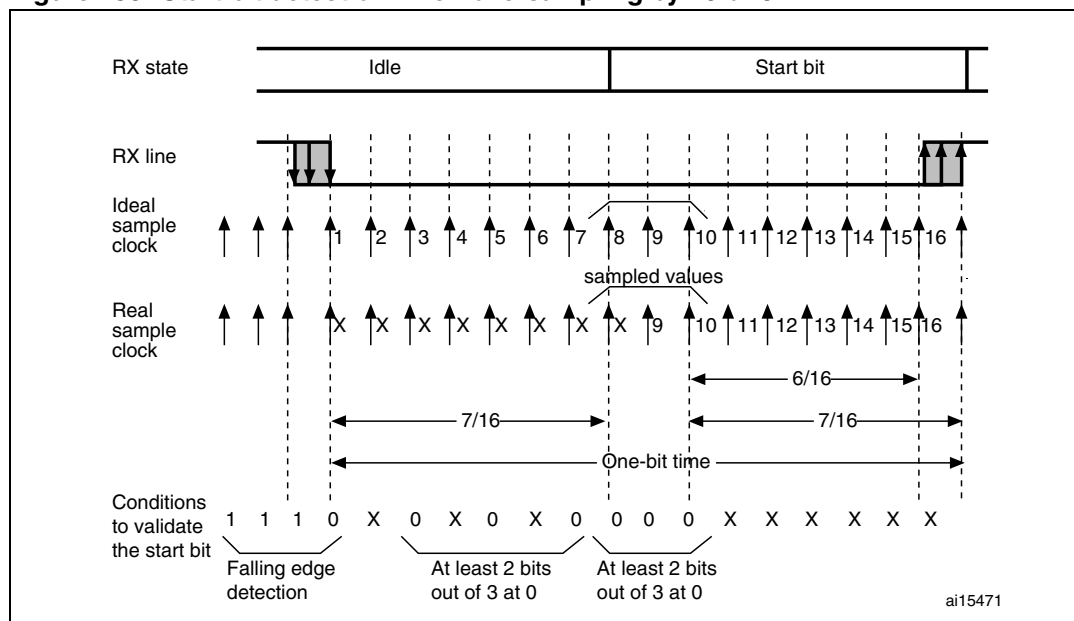
Figure 250. Start bit detection when oversampling by 16 or 8
