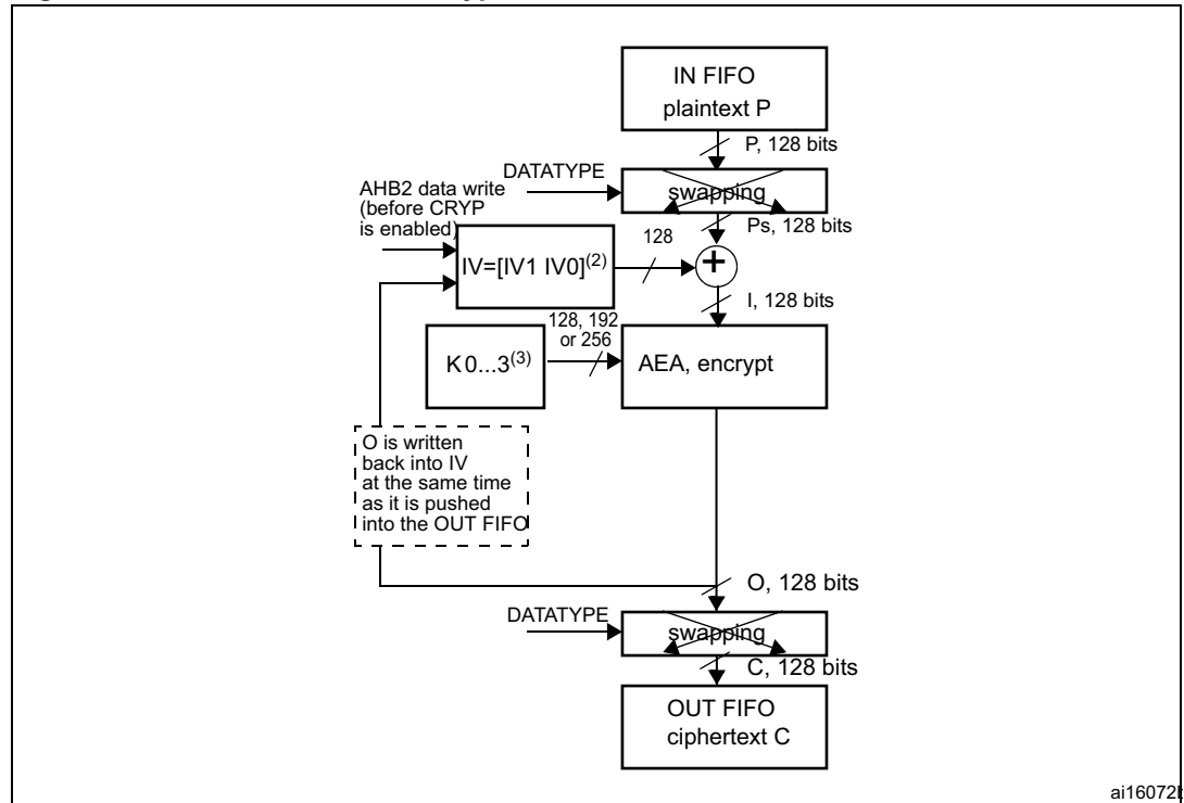
Figure 209. AES-CBC mode encryption
