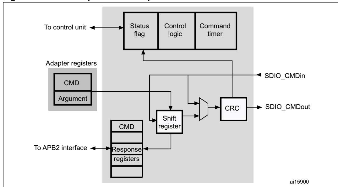
Figure 316. SDIO adapter command path
