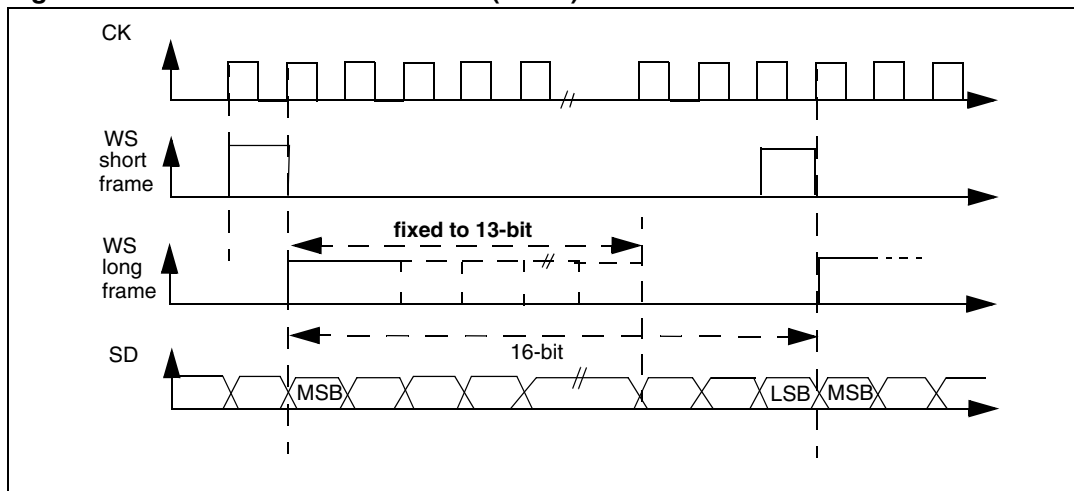
Figure 304. PCM standard waveforms (16-bit)
