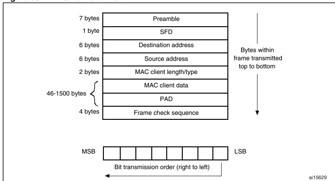
Figure 331. MAC frame format
