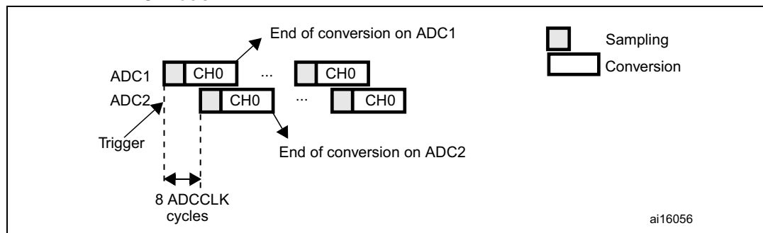
Figure 46. Interleaved mode on 1 channel in continuous conversion mode: dual ADC mode
