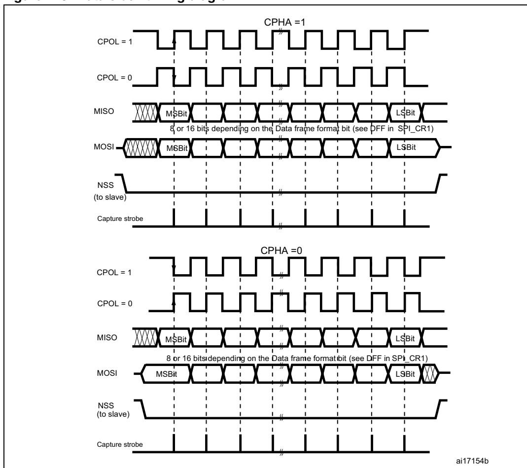
Figure 273. Data clock timing diagram
