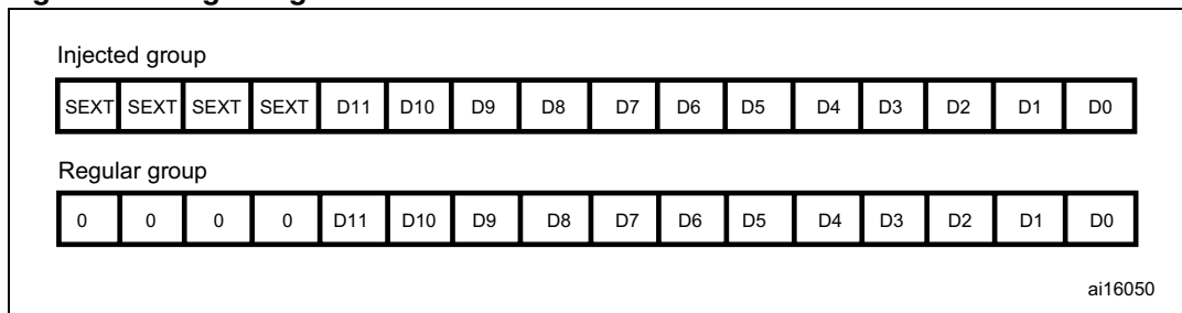
Figure 38. Right alignment of 12-bit data
