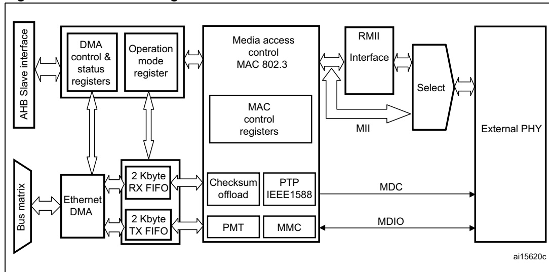
Figure 321. ETH block diagram
