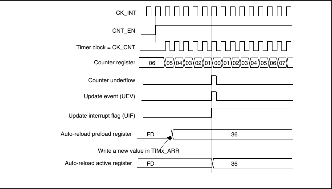
Figure 137. Counter timing diagram, Update event with ARPE=1 (counter underflow)
