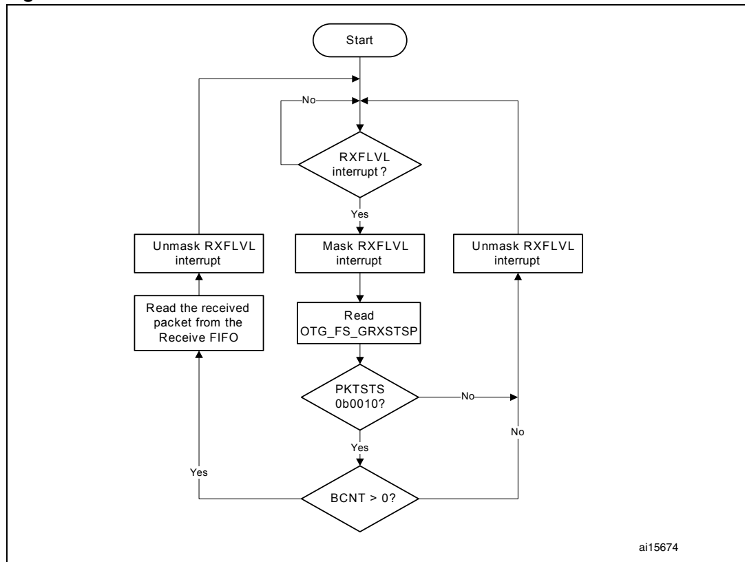
Figure 386. Receive FIFO read task
