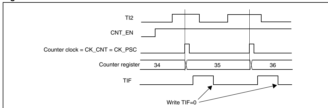
Figure 177. Control circuit in external clock mode 1
