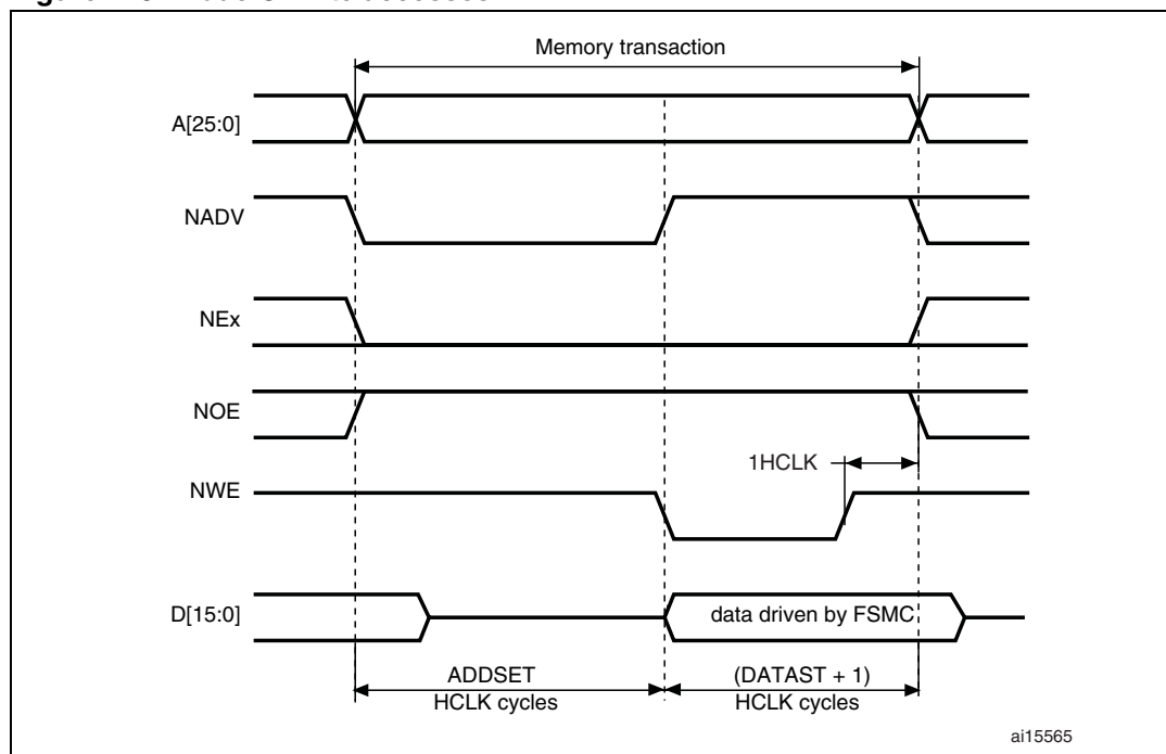
Figure 413. Mode C write accesses
