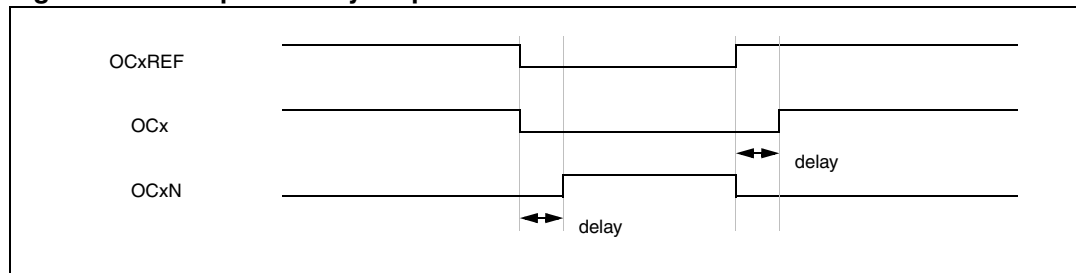
Figure 105. Complementary output with dead-time insertion.
