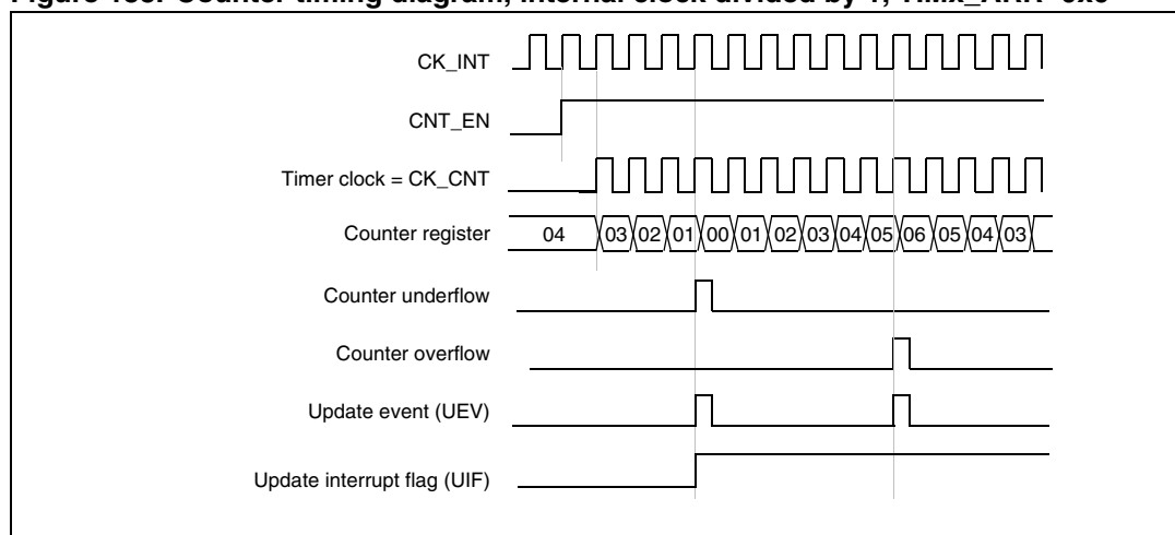
Figure 133. Counter timing diagram, internal clock divided by 1, TIMx_ARR=0x6
