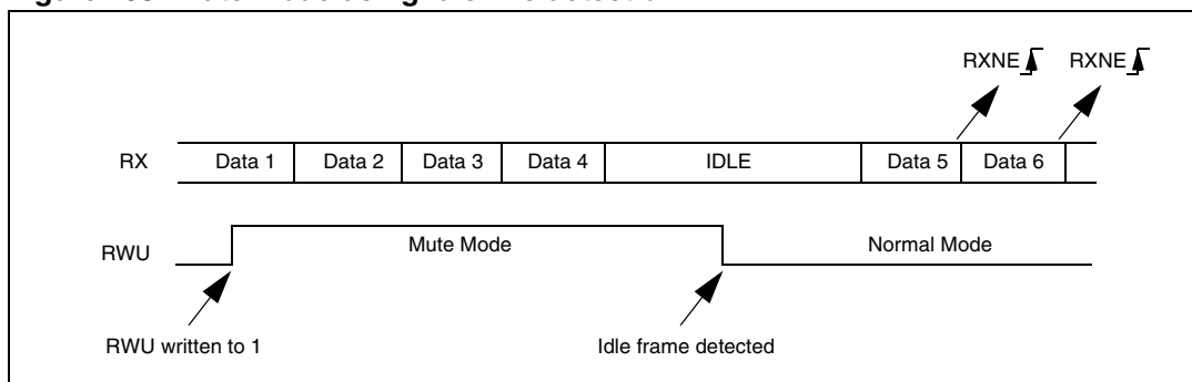
Figure 253. Mute mode using Idle line detection
