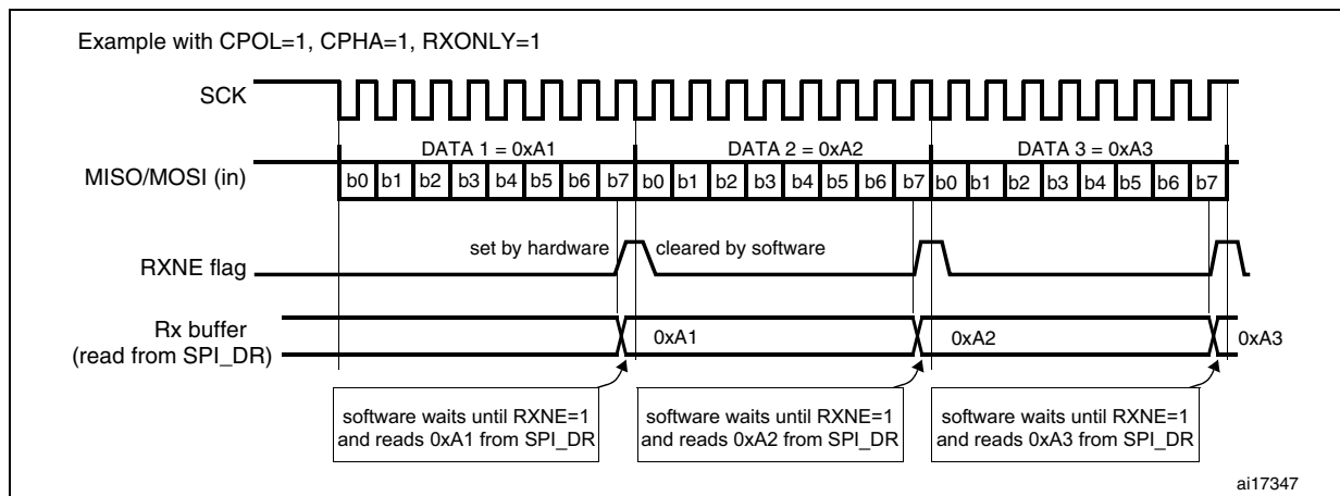
Figure 282. RXNE behavior in receive-only mode (BIDIRMODE=0 and RXONLY=1) in the case of continuous transfers
