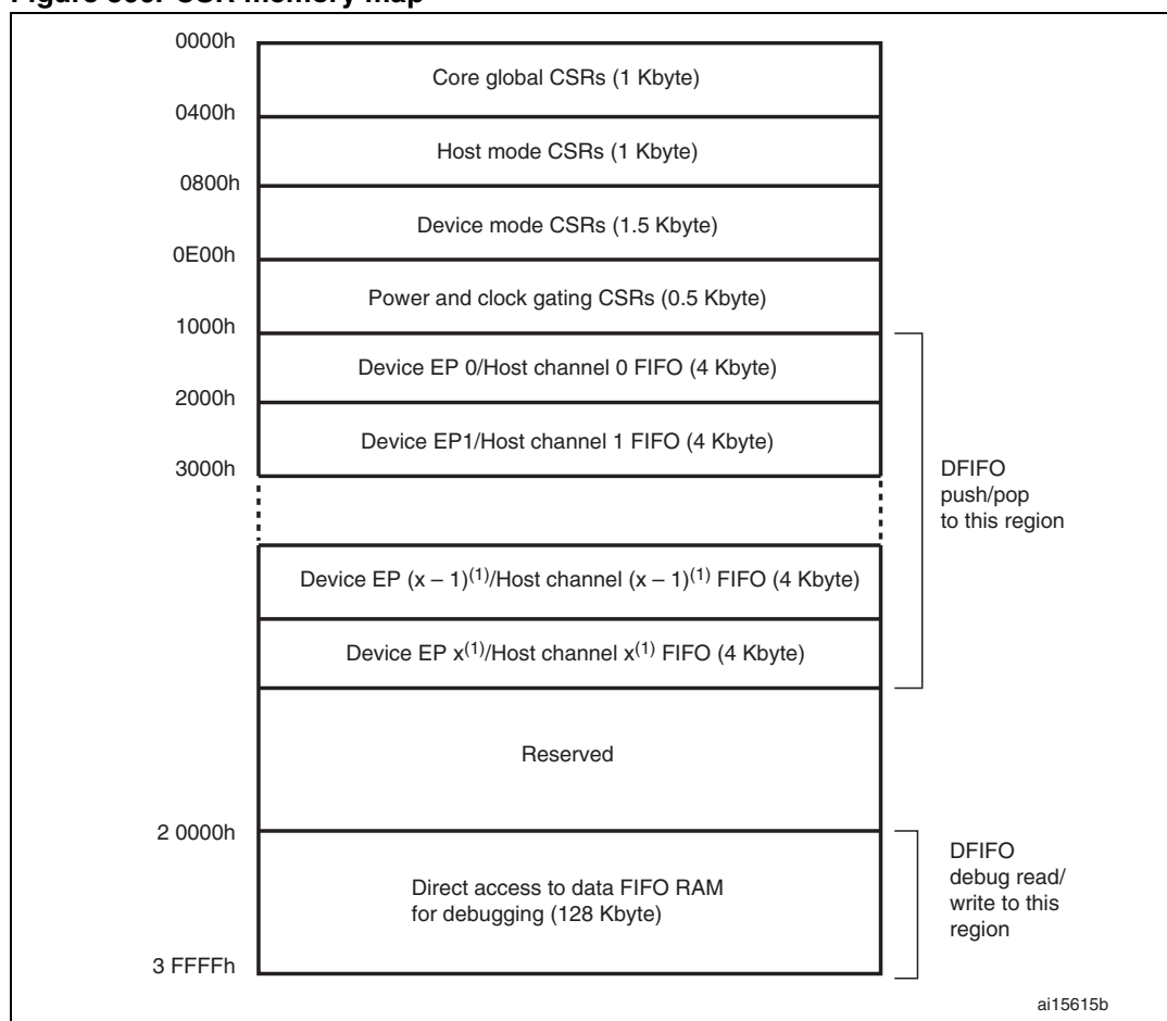
Figure 366. CSR memory map
