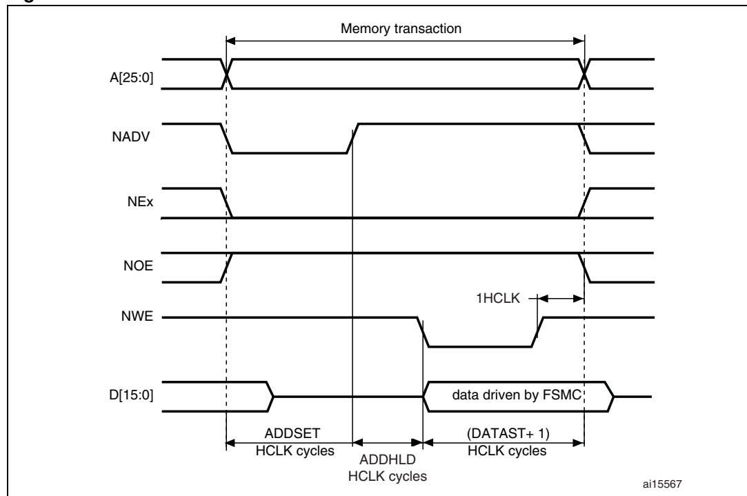
Figure 415. Mode D write accesses
