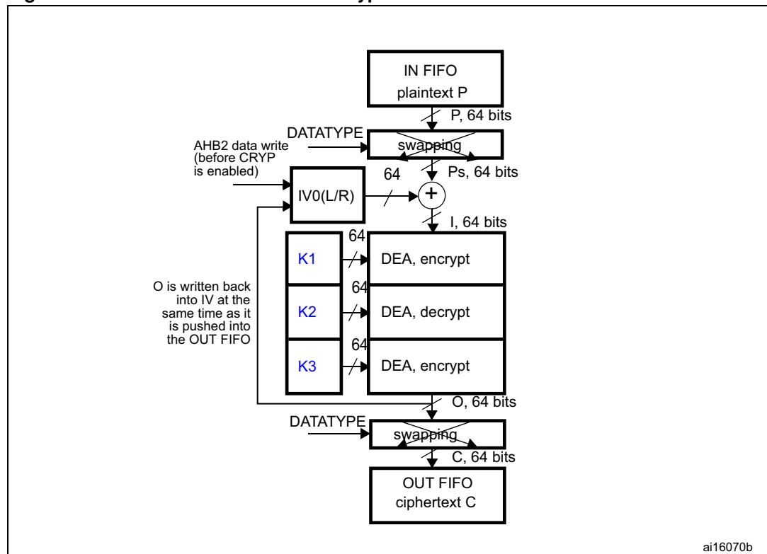
Figure 205. DES/TDES-CBC mode encryption
