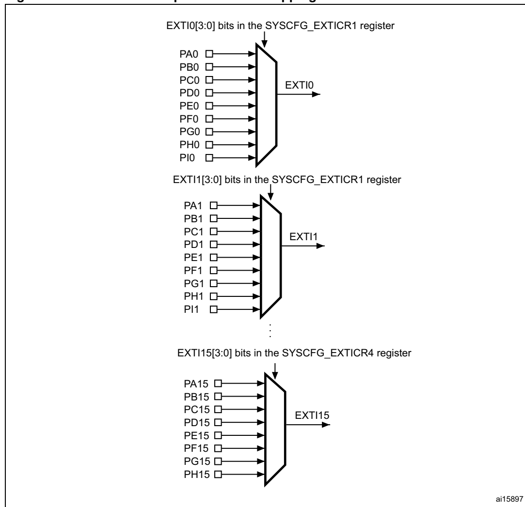
Figure 33. External interrupt/event GPIO mapping
