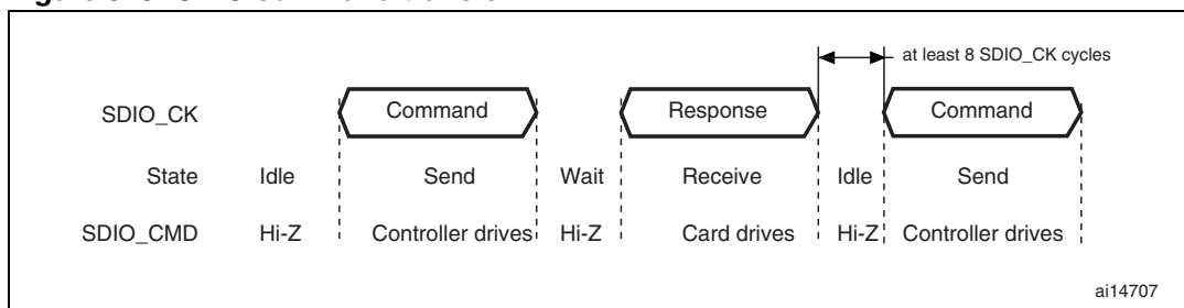
Figure 318. SDIO command transfer
