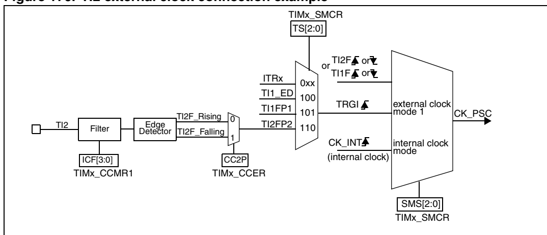
Figure 176. TI2 external clock connection example
