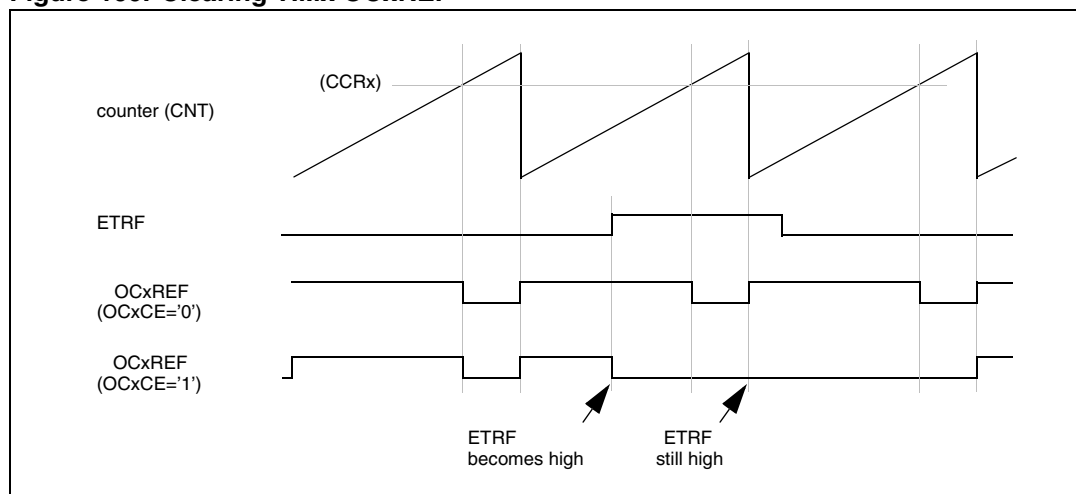
Figure 109. Clearing TIMx OCxREF
