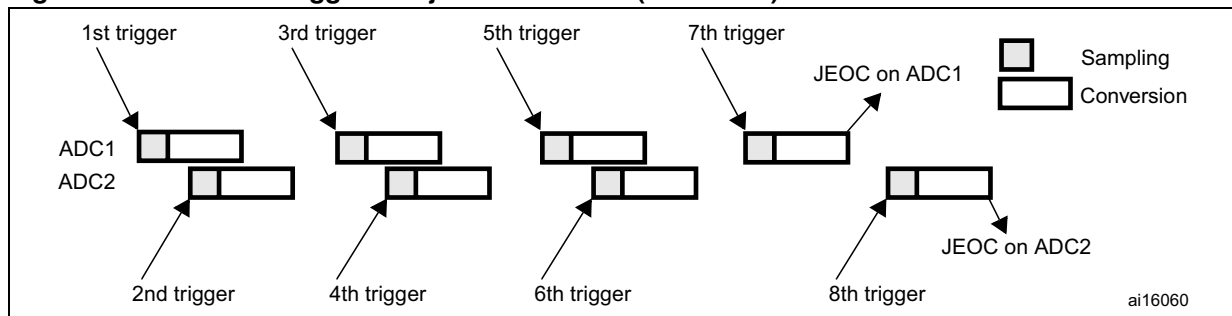
Figure 49. Alternate trigger: 4 injected channels (each ADC) in discontinuous mode
