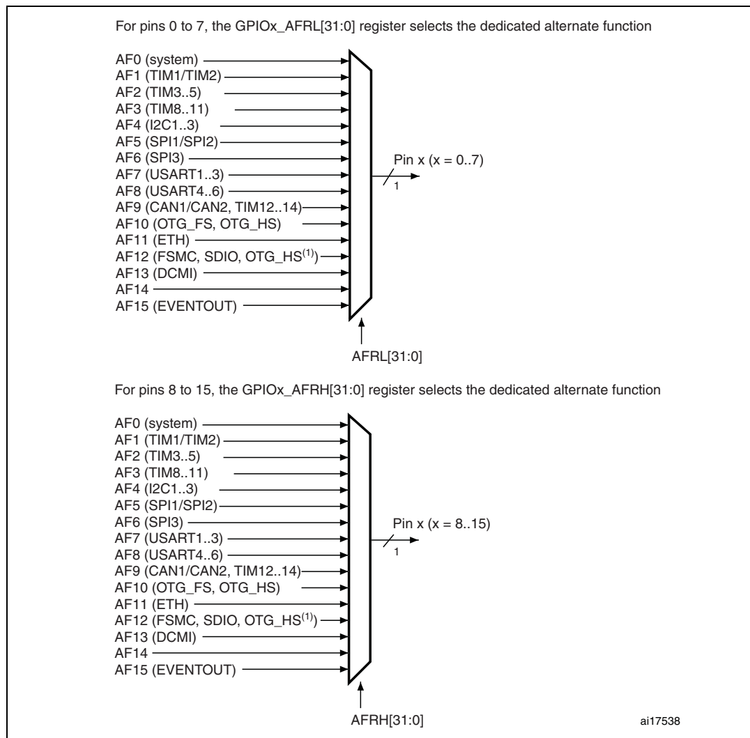
Figure 18. Selecting an alternate function on STM32F405xx/07xx and STM32F415xx/17xx
