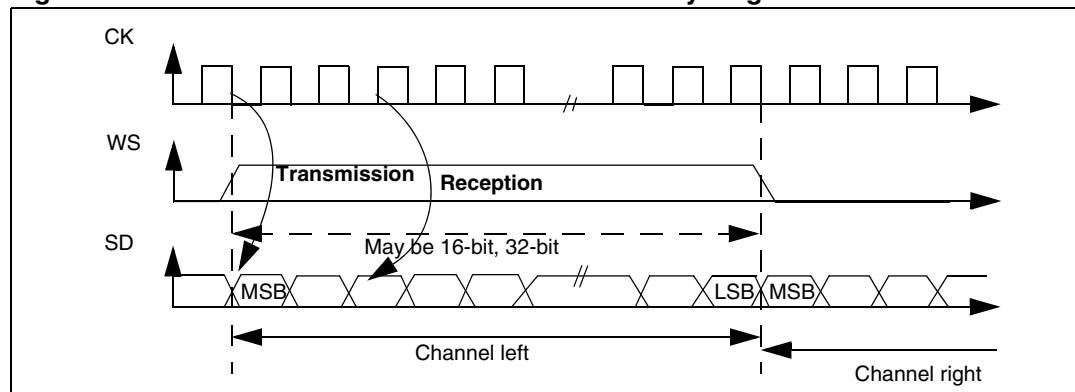
Figure 295. MSB Justified 16-bit or 32-bit full-accuracy length with CPOL = 0
