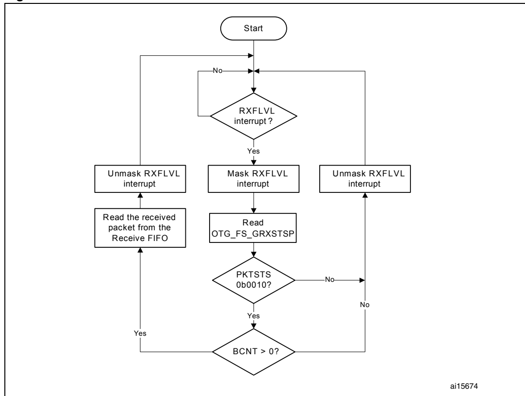
Figure 368. Receive FIFO read task
