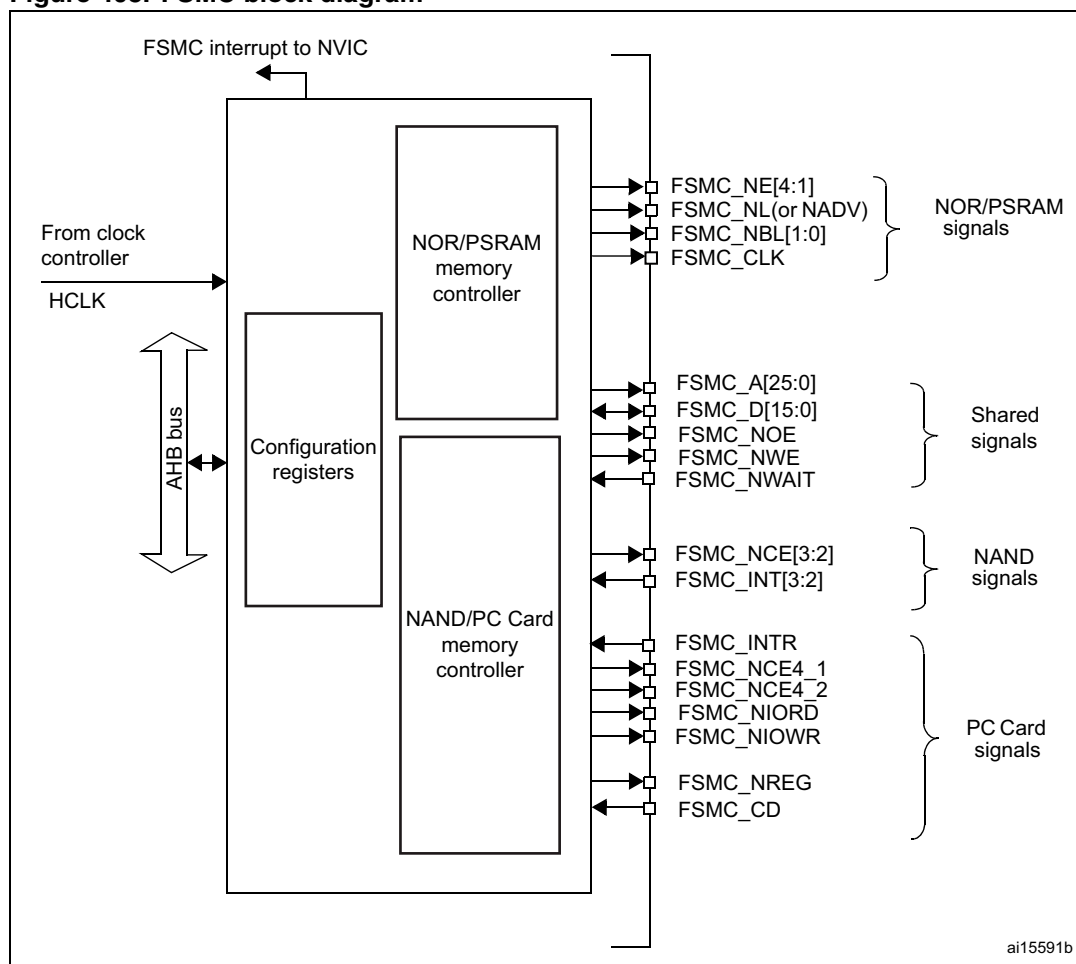
Figure 403. FSMC block diagram
