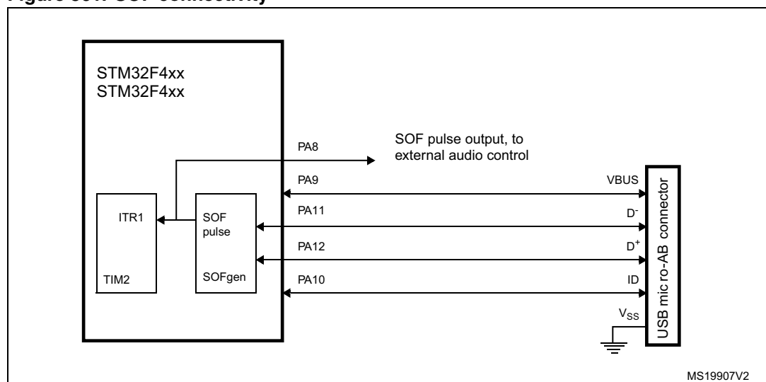
Figure 361. SOF connectivity
