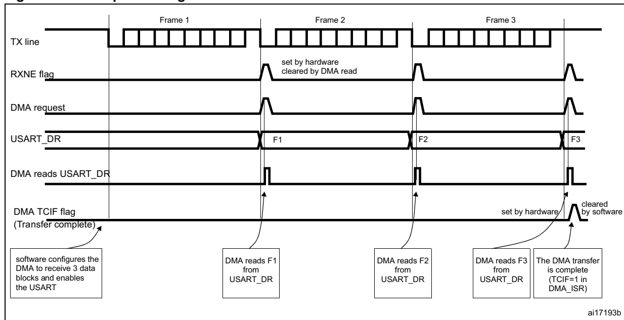
Figure 266. Reception using DMA
