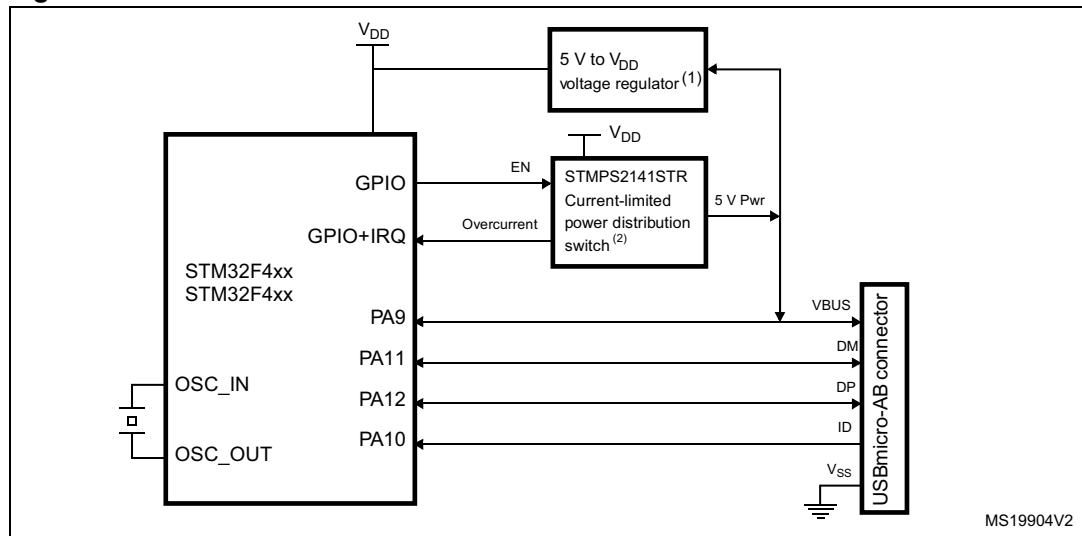
Figure 358. OTG A-B device connection
