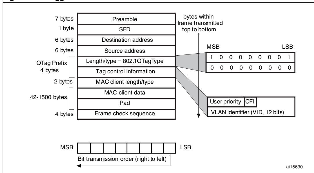
Figure 332. Tagged MAC frame format
