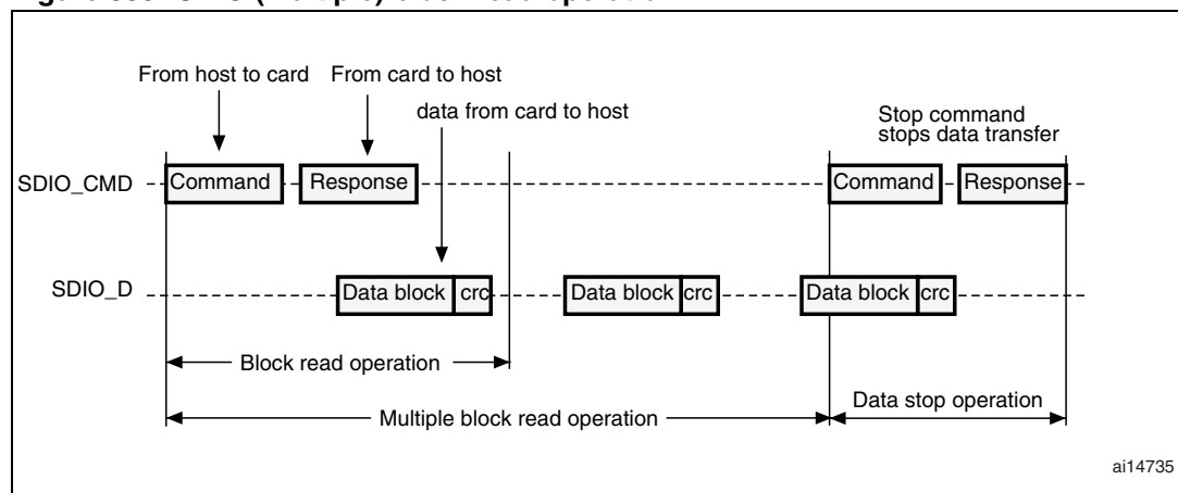
Figure 309. SDIO (multiple) block read operation
