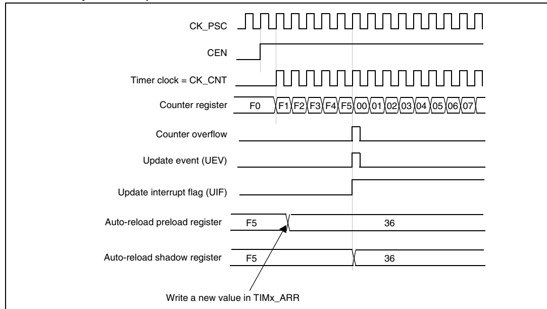
Figure 174. Counter timing diagram, update event when ARPE=1 (TIMx_ARR preloaded)
