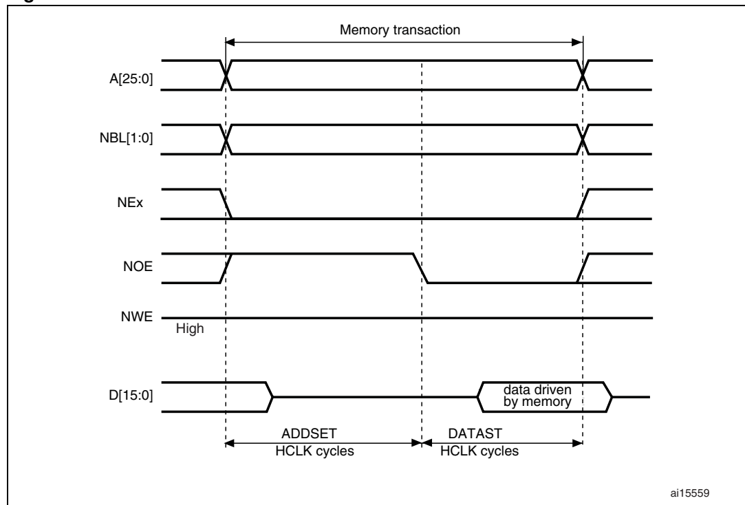
Figure 407. ModeA read accesses
