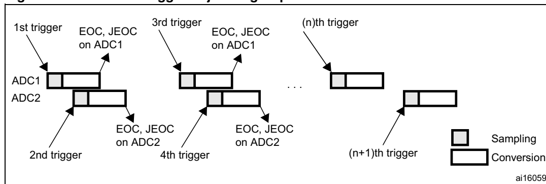
Figure 48. Alternate trigger: injected group of each ADC
