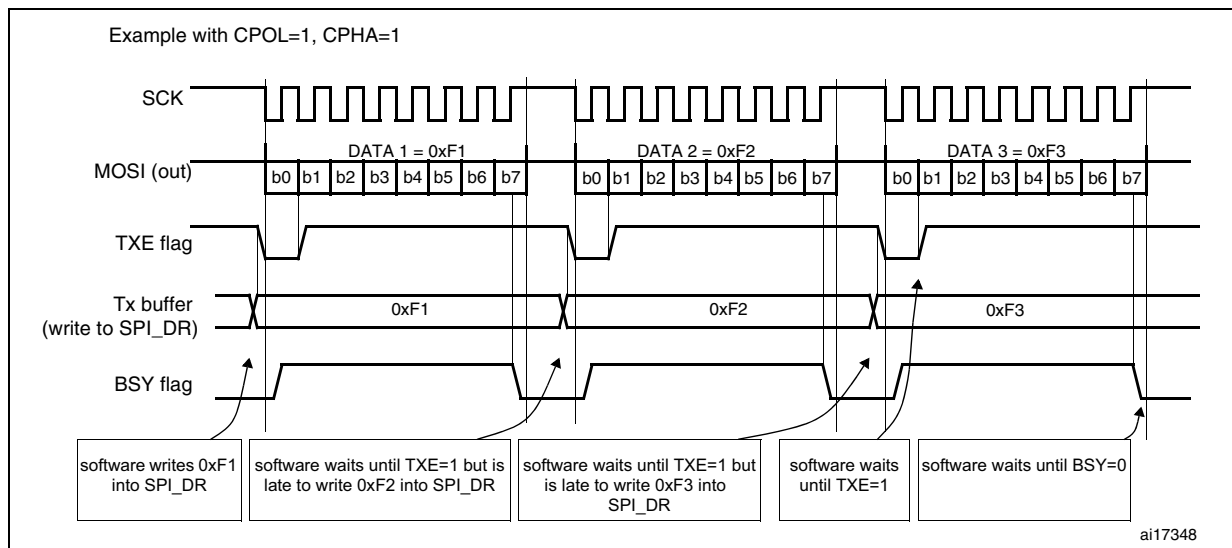
Figure 283. TXE/BSY behavior when transmitting (BIDIRMODE=0 and RXONLY=0) in the case of discontinuous transfers
