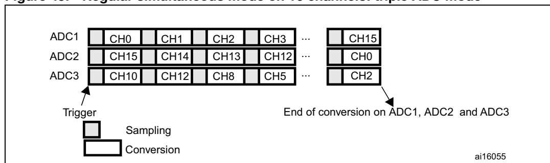
Figure 45. Regular simultaneous mode on 16 channels: triple ADC mode
