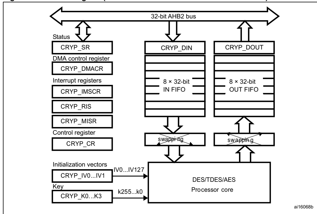
Figure 201. Block diagram (STM32F405xx/07xx and STM32F415xx/17xx)
