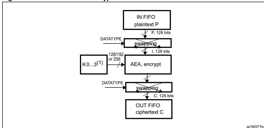
Figure 207. AES-ECB mode encryption
