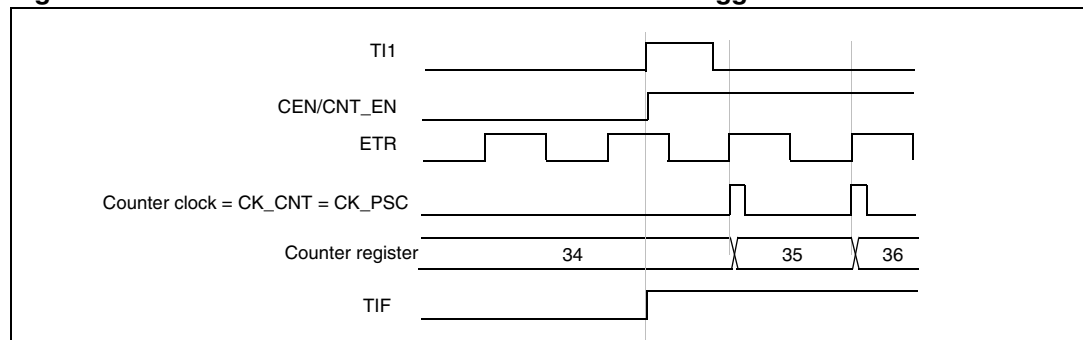
Figure 118. Control circuit in external clock mode 2 + trigger mode
