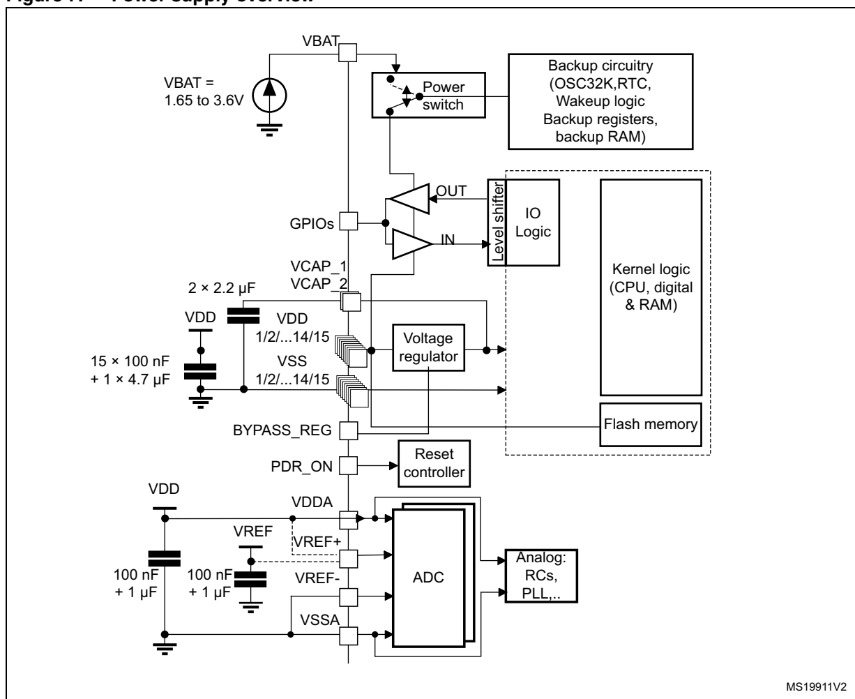
Figure 7. Power supply overview
