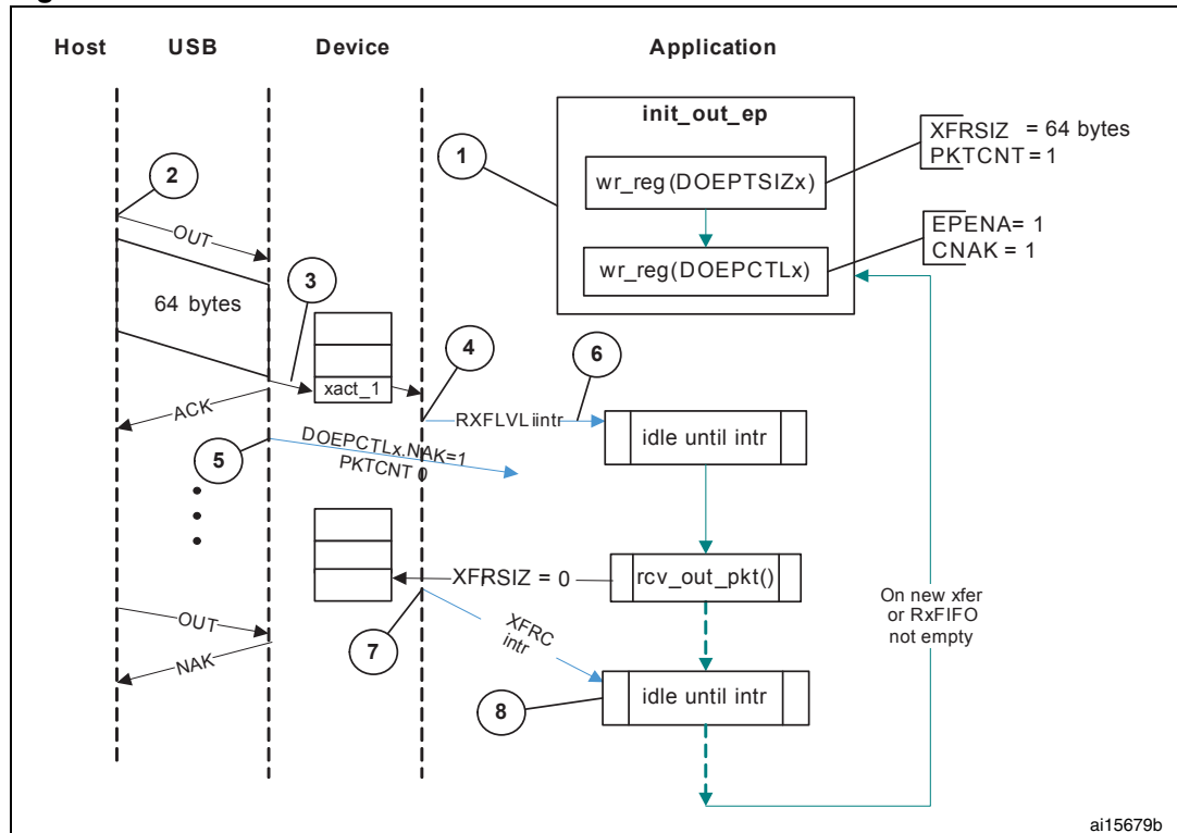
Figure 375. Bulk OUT transaction
