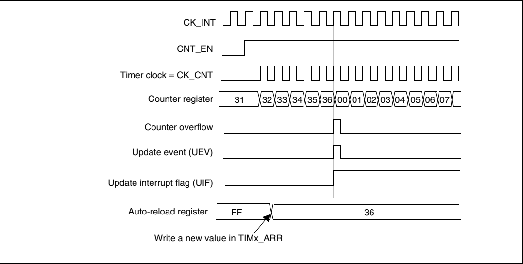
Figure 126. Counter timing diagram, Update event when ARPE=0 (TIMx_ARR not preloaded)
