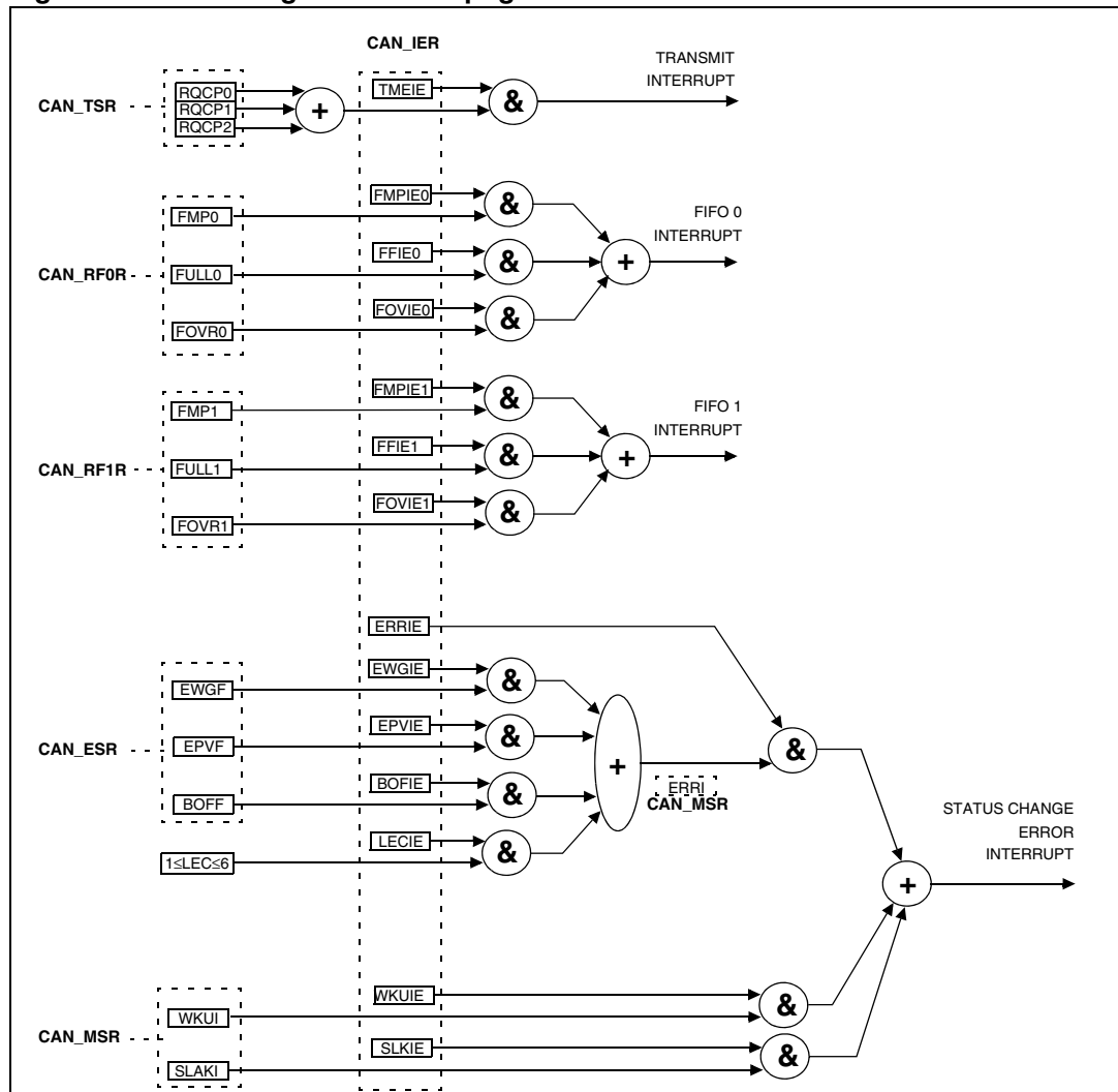
Figure 237. Event flags and interrupt generation
