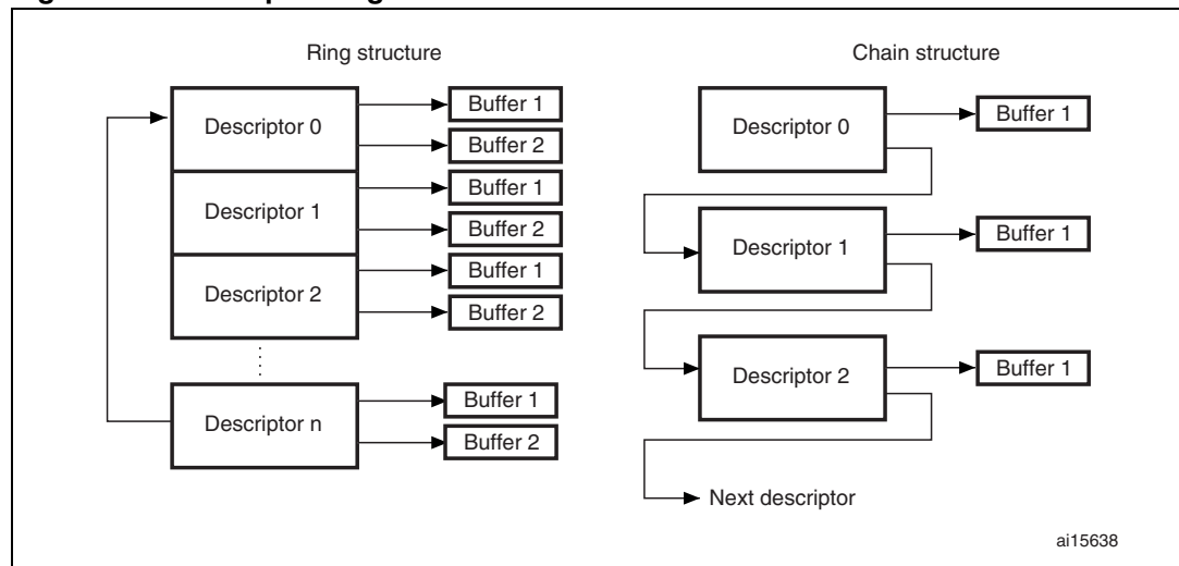
Figure 347. Descriptor ring and chain structure
