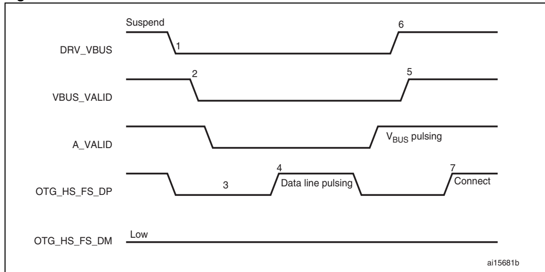
Figure 399. A-device SRP
