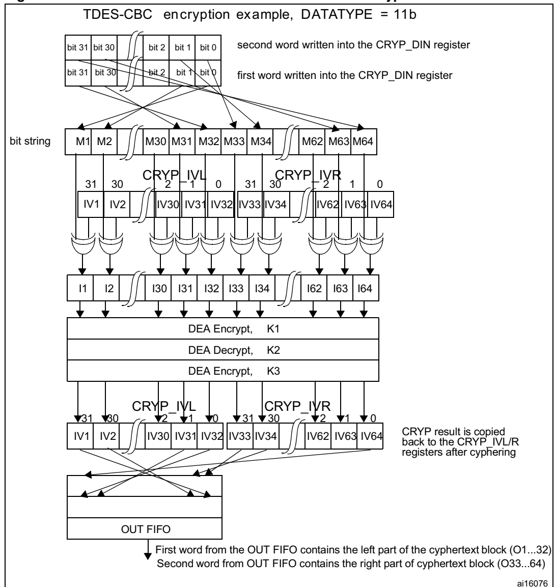
Figure 215. Initialization vectors use in the TDES-CBC encryption
