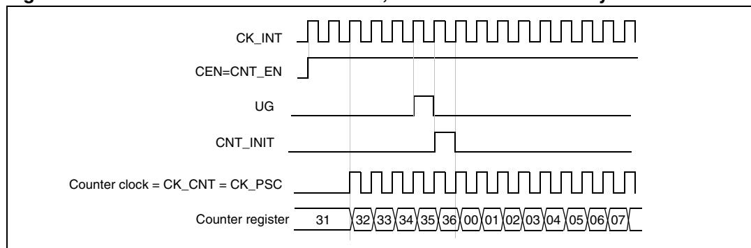
Figure 197. Control circuit in normal mode, internal clock divided by 1
