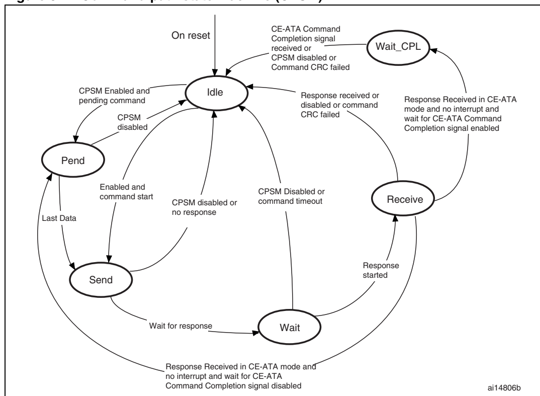
Figure 317. Command path state machine (CPSM)
