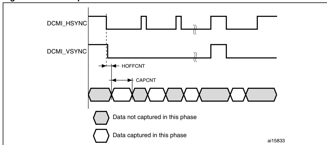
Figure 69. Data capture waveforms
