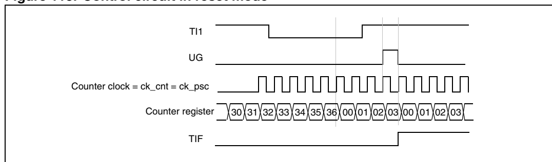
Figure 115. Control circuit in reset mode
