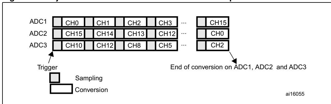
Figure 43. Injected simultaneous mode on 4 channels: triple ADC mode
