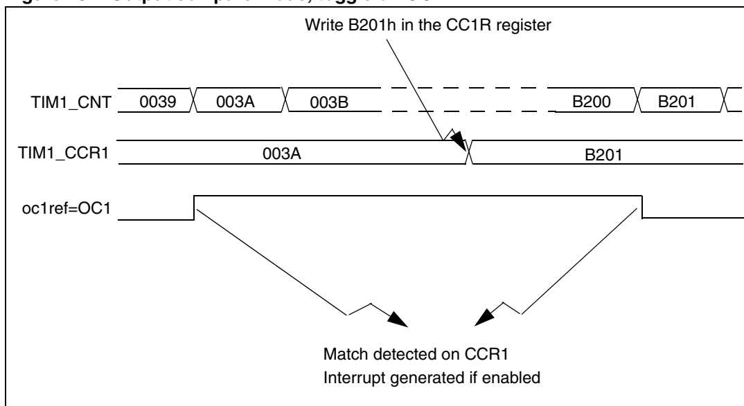
Figure 182. Output compare mode, toggle on OC1.
