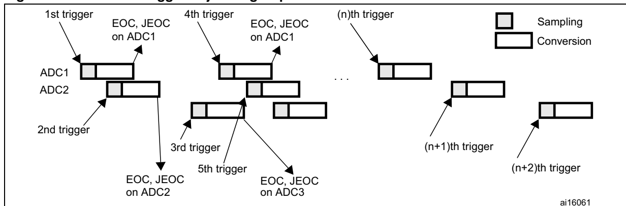
Figure 50. Alternate trigger: injected group of each ADC
