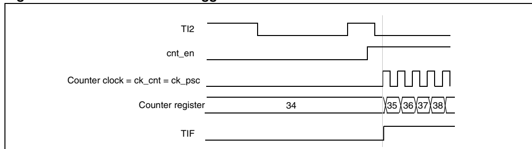
Figure 117. Control circuit in trigger mode
