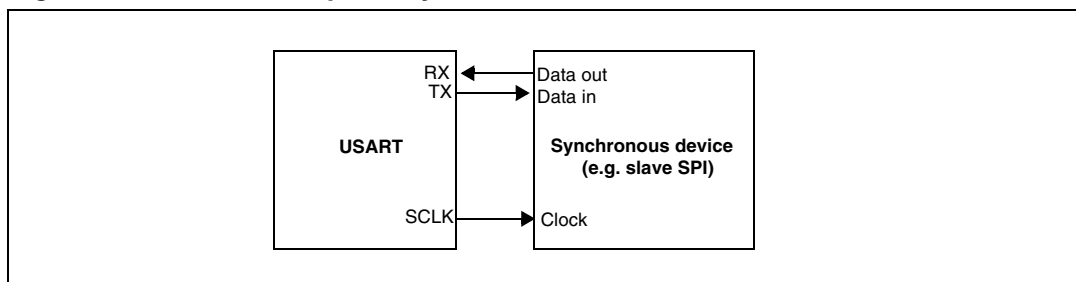
Figure 257. USART example of synchronous transmission
