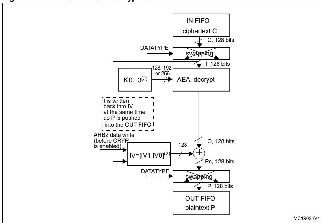
Figure 210. AES-CBC mode decryption
