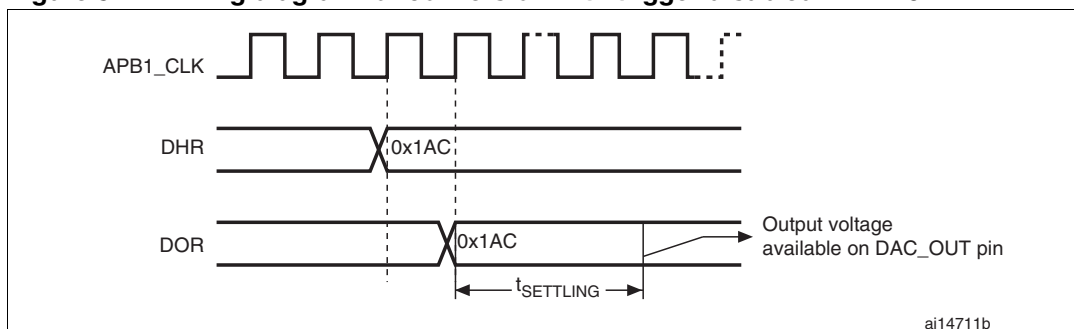
Figure 57. Timing diagram for conversion with trigger disabled TEN = 0
