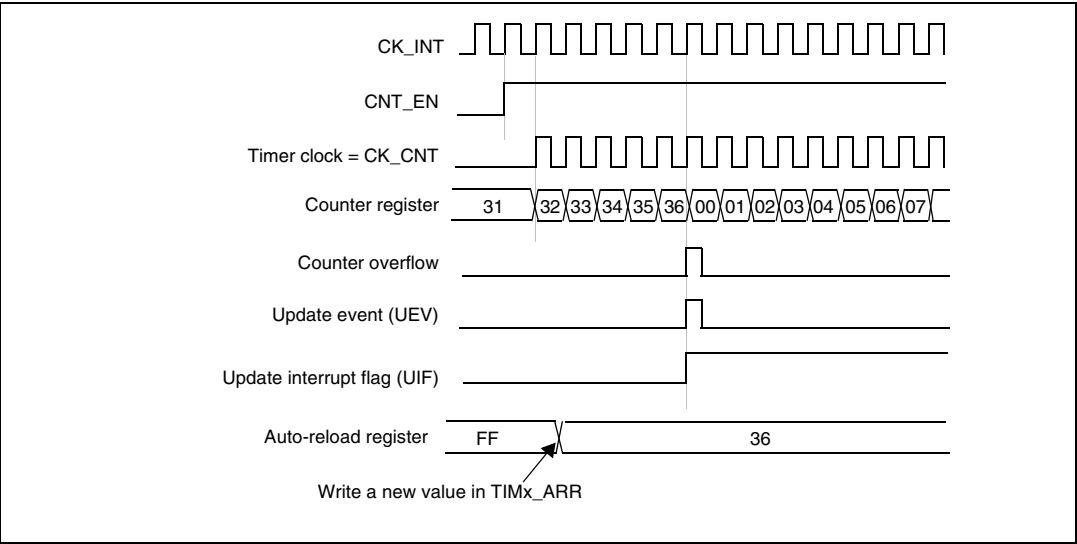
Figure 195. Counter timing diagram, update event when ARPE = 0 (TIMx_ARR not preloaded)
