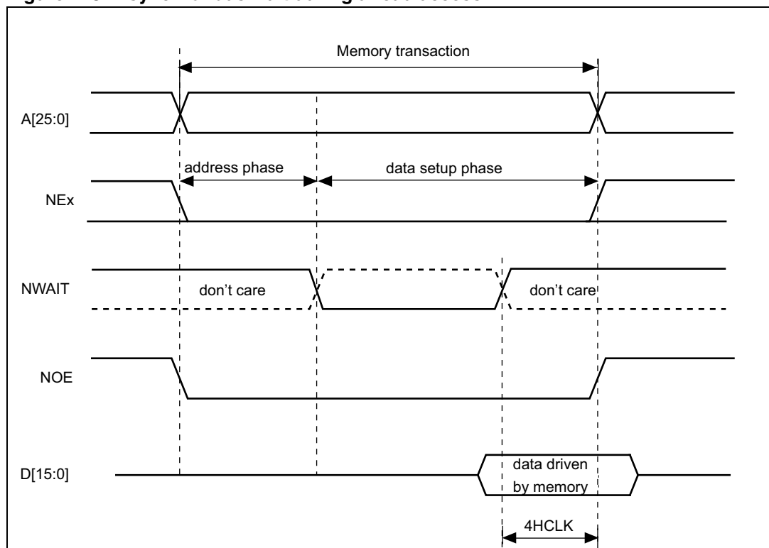
Figure 418. Asynchronous wait during a read access
