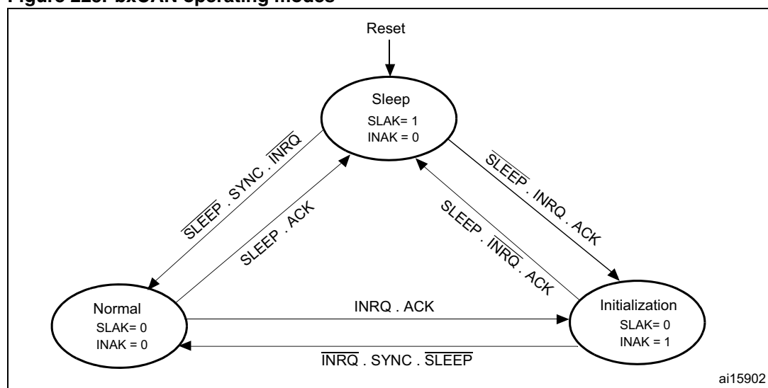
Figure 225. bxCAN operating modes
