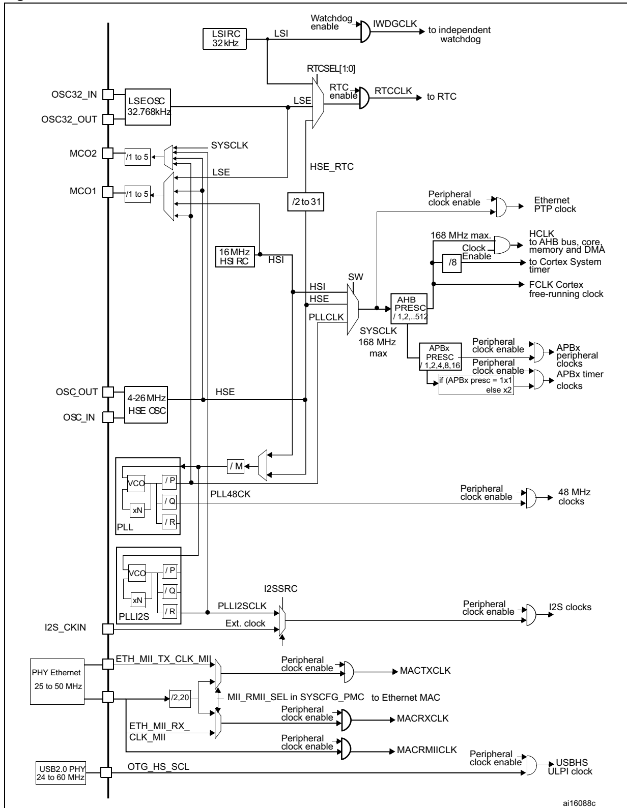
Figure 13. Clock tree
