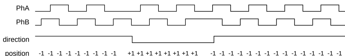
Fig 107. Quadrature Encoder Basic Operation
