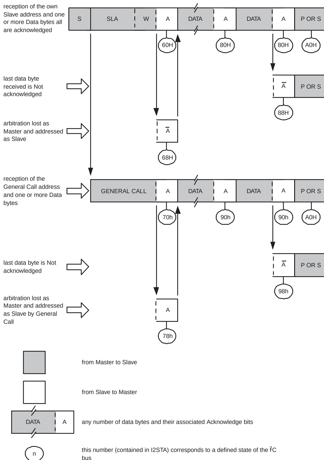
Fig 170. Format and states in the Slave Receiver mode
