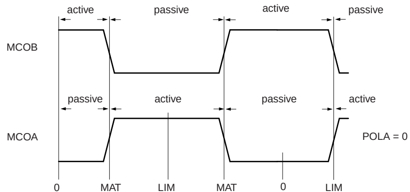
Fig 101. Center-aligned PWM waveform without dead time, POLA = 0
