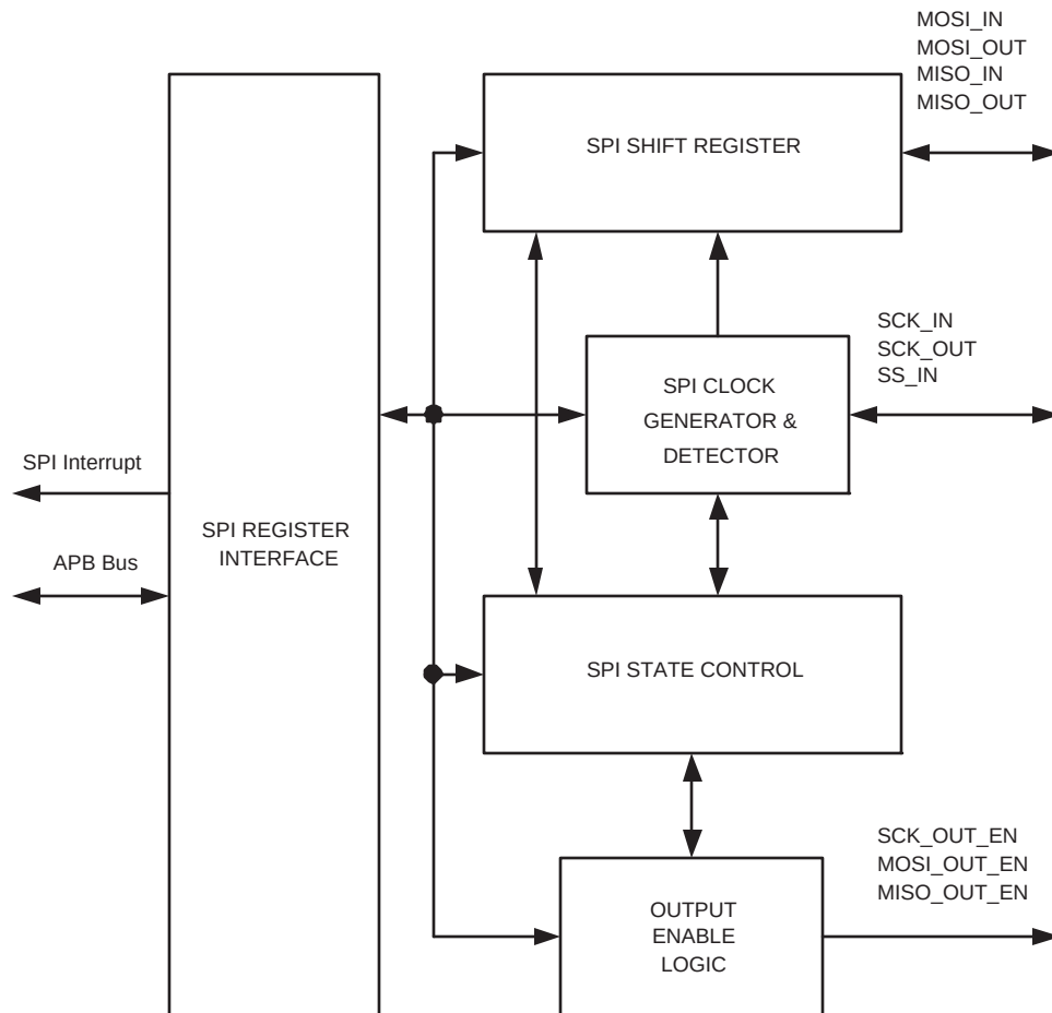
Fig 131. SPI block diagram
