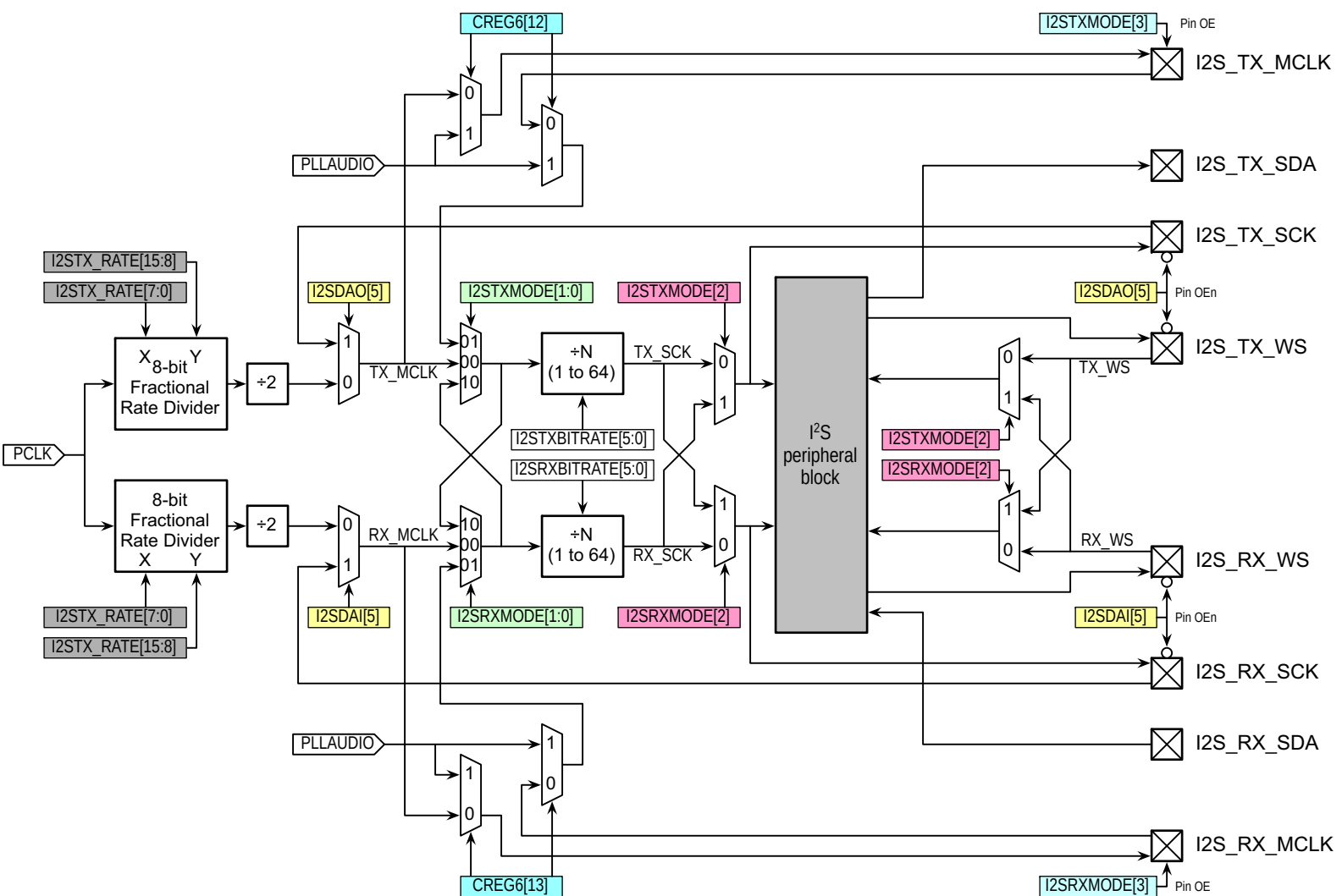
Fig 135. I2S clocking and pin connections
