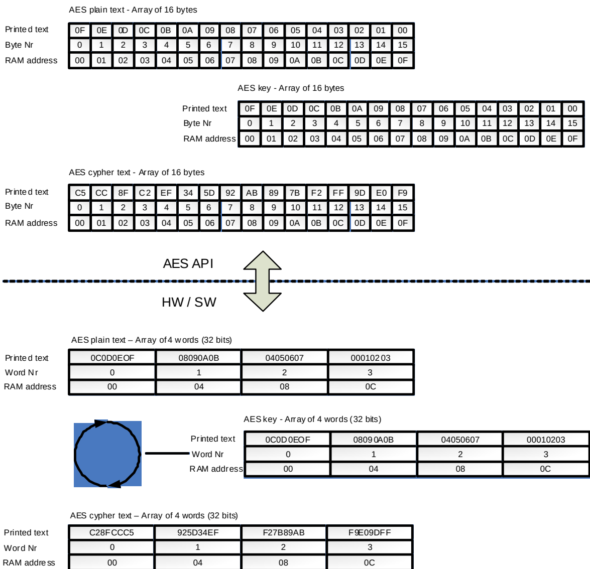
Fig 22. AES endianness
