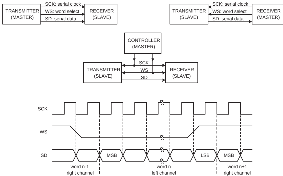
Fig 134. Simple I2S configurations and bus timing
