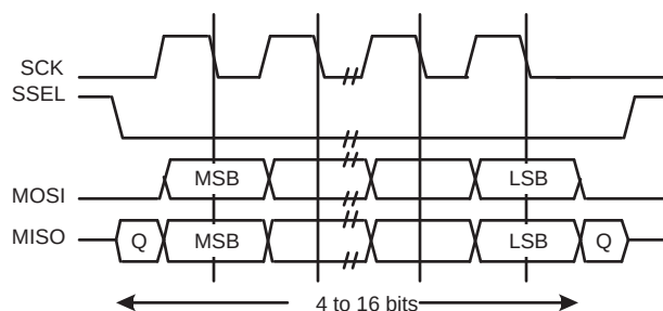
Fig 125. SPI frame format with CPOL=0 and CPHA=1
