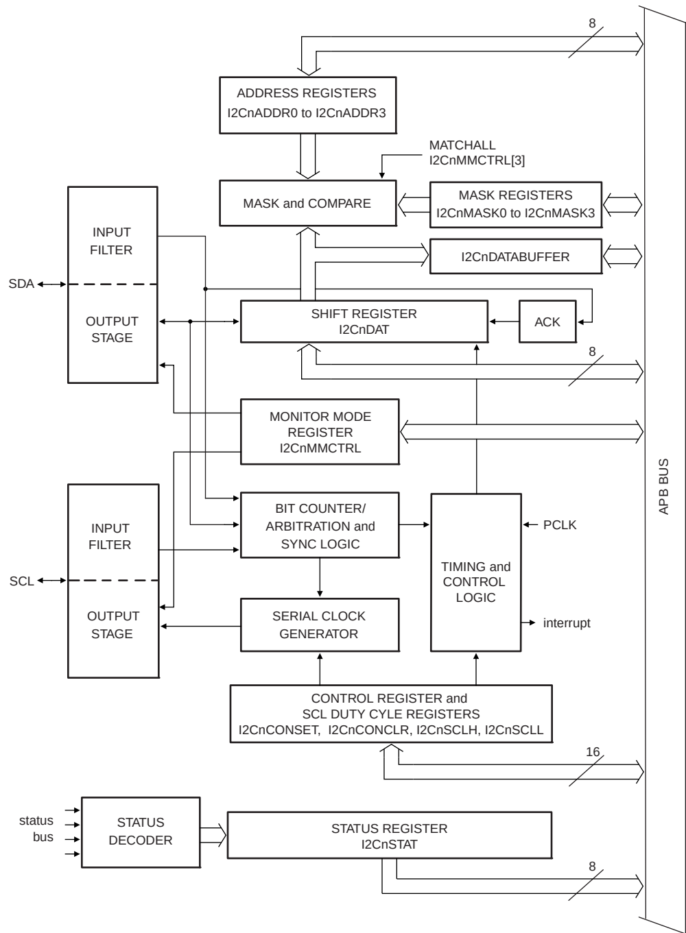
Fig 165. I 2 C serial interface block diagram
