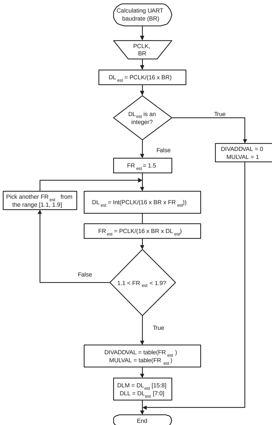
Fig 117. Algorithm for setting USART dividers
