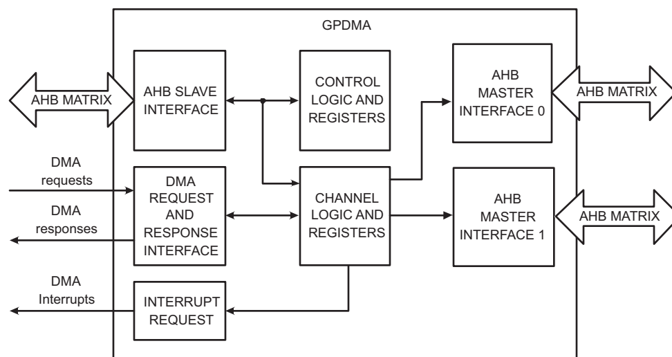
Fig 44. DMA controller block diagram
