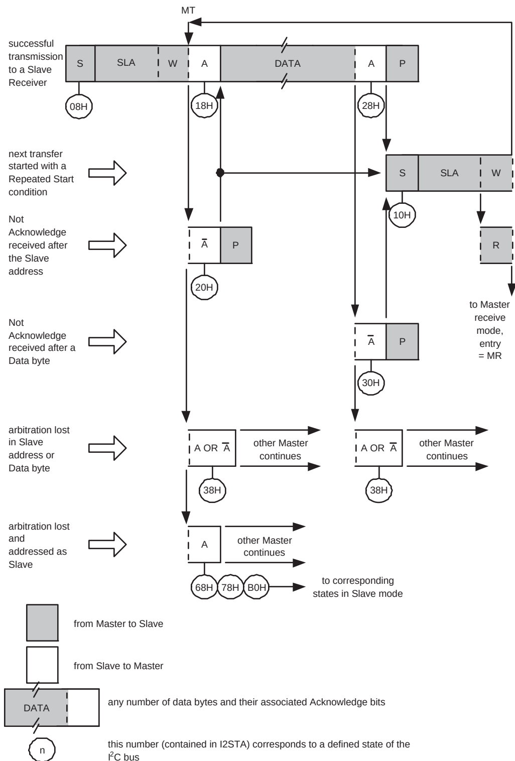
Fig 168. Format and states in the Master Transmitter mode
