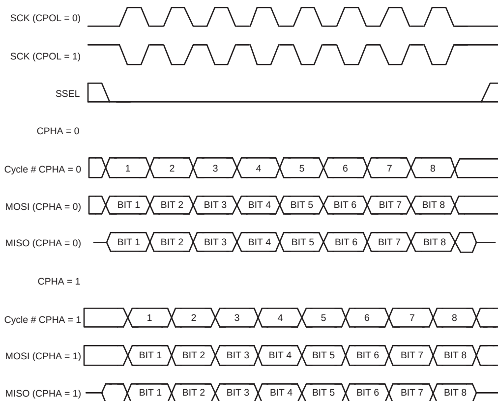
Fig 132. SPI data transfer format (CPHA = 0 and CPHA = 1)
