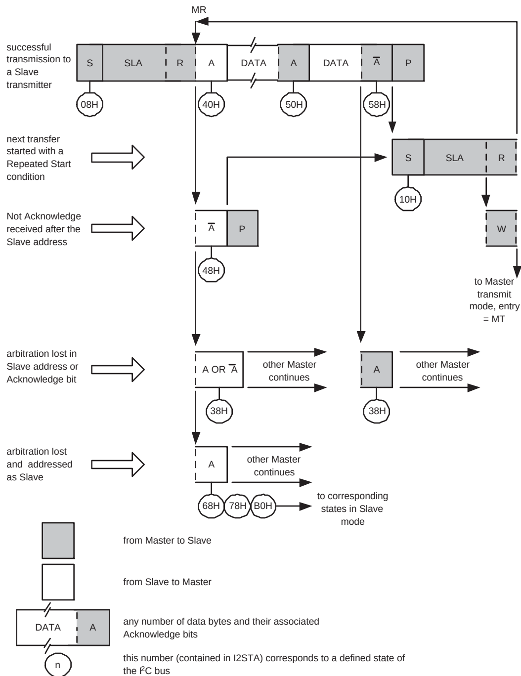
Fig 169. Format and states in the Master Receiver mode
