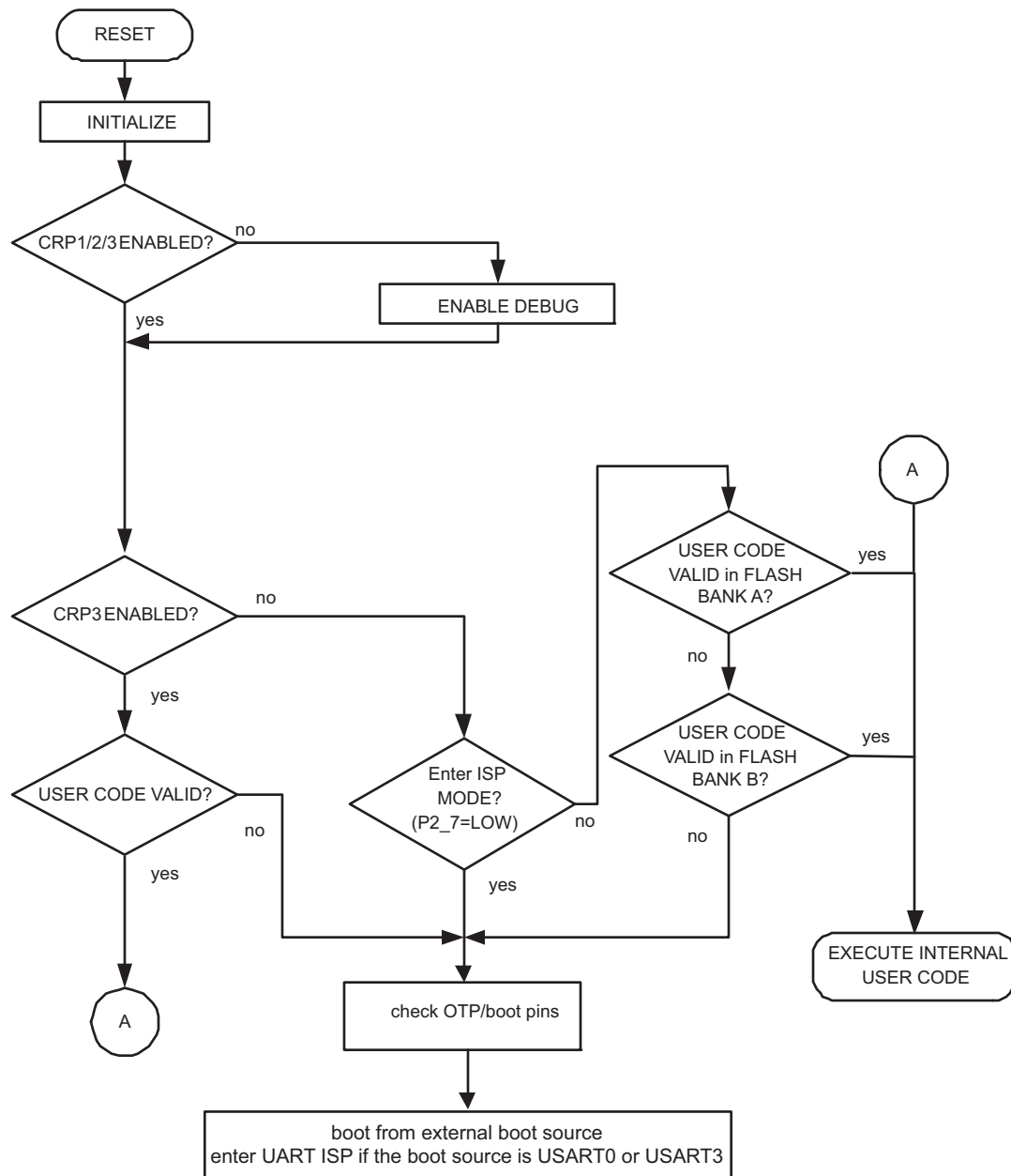
Fig 176. Boot process flowchart for LPC43xx parts with flash
