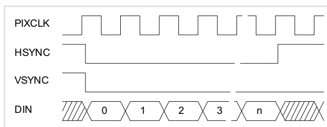
Fig 43. SGPIO camera interface configuration
