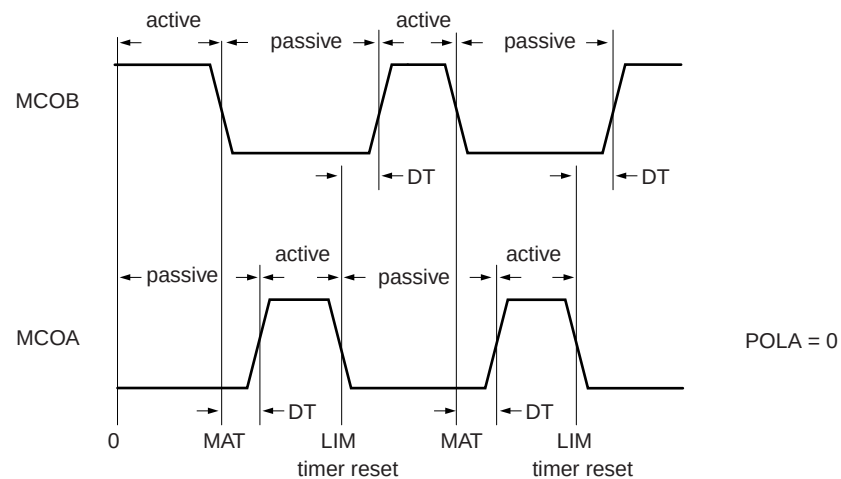
Fig 102. Edge-aligned PWM waveform with dead time, POLA = 0
